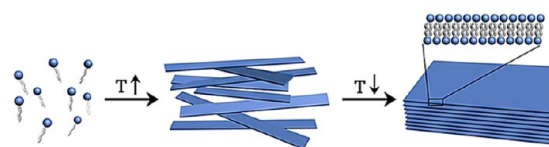
Figure 16. Illustration of structural transition of surfactant in ionic liquid as a function of temperature [Reprinted with permission from ref 201. Copyright 2016. John Wiley and Sons].
