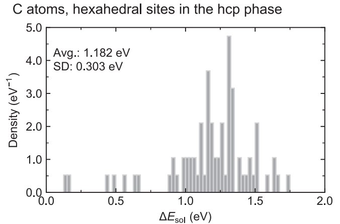
FIG. 10. Distribution of computed solution energies \Delta E_{\text{sol}} of interstitial C atoms at the hexahedral sites in hcp CrMnFeCoNi. The average (avg.) and the standard deviation (SD) of \Delta E_{\text{sol}} are also shown in the panels.
