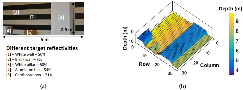
Figure 13. (a) Photograph of the example target scene and (b) 32 \times 32 image reconstructed in a scanning LiDAR setup [8].
