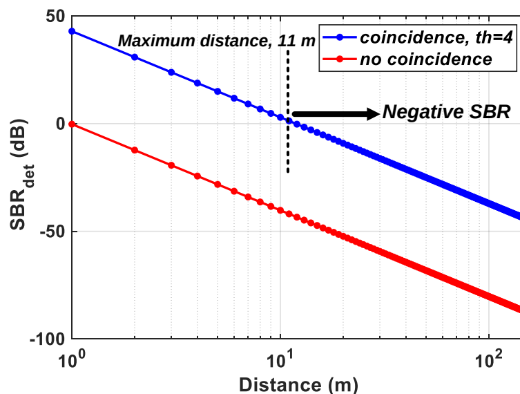
Figure 11. SBR achieved after detection without and with coincidence with th = 4 .
