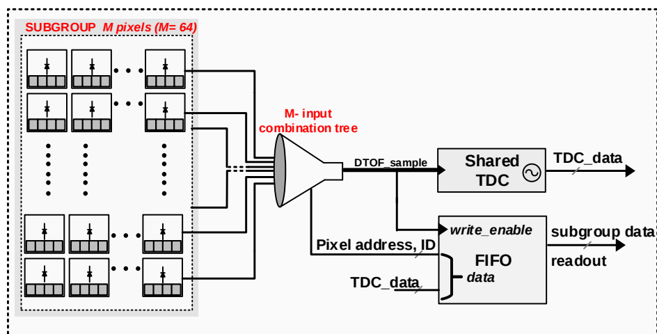
Figure 4. A block diagram of a DTOF sensor in a shared architecture.
