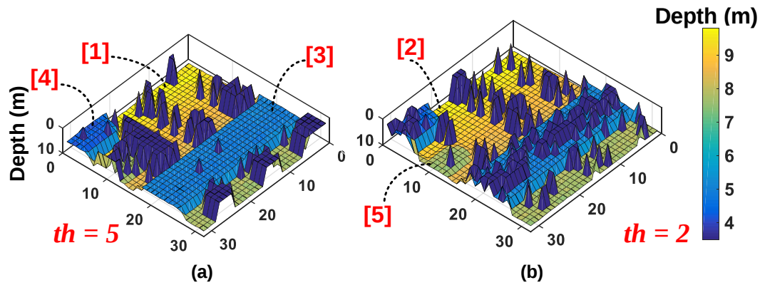
Figure 15. Simulated result of the 3D image reconstructed through proposed DTOF model (a) coincidence threshold, th = 5 and (b) coincidence threshold, th = 2 .
