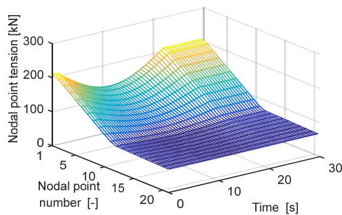
(b) Belt tension
