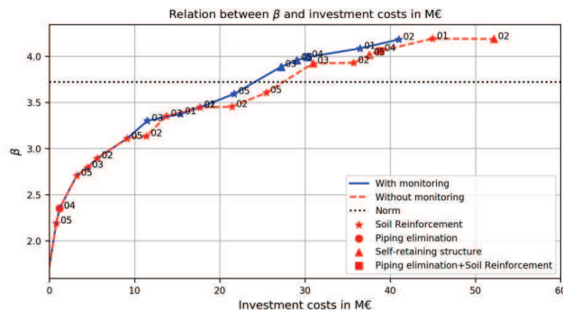
Figure 5. Total investment costs (LCC) versus the reliability for the entire segment for prioritized investments with and without monitoring. Symbols indicate different measures, numbers indicate the section. Where lines overlap identical measures are taken in both strategies.
