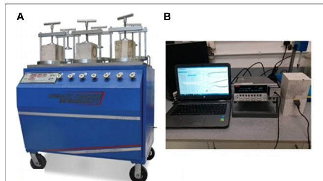
FIGURE 3 | (A) Digimatic concrete water permeability apparatus and (B) thermal conductivity test using C-THERM Tckit.
