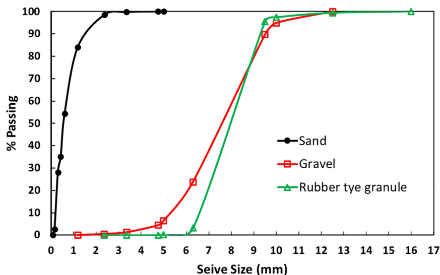
FIGURE 2 | Grain size distribution of different types of aggregates.
