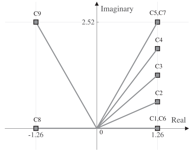
Fig. 1. Experimental conditions shown on the complex plane.
