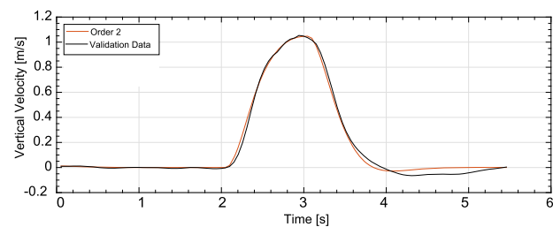
(c) Vertical velocity response to thrust command
