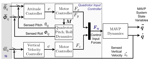
Fig. 18 On-board quadrotor input controller showing inner attitude and vertical velocity stabiliser loops. Motor inputs c are generated by controllers, resulting in forces F and moments M . Internally stabilised quadrotor attitude is perturbed by M ; control force F_u affects MAVP dynamics. Sensed measures are internally fed-back on-board the quadrotor
