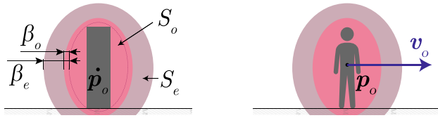
Fig. 2 Cuboid obstacle ( left ) with fixed position p_o or dynamic (human) obstacle ( right ) with constant velocity v_o each modelled by bounding S_o and expanded S_e ellipsoid with dimensional buffers \beta
