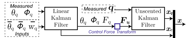
Fig. 6 Cascaded state estimation using Linear and Unscented KF and measured MCS data. Linear KF estimates \mathbf{x}_c based on the quadrotor input model, measured true pitch, roll and inputs. Unscented KF estimates \mathbf{x}_q based on MAVP model, measured MAVP configuration \mathbf{q} and control force inputs computed by (3) using the Linear KF outputs
