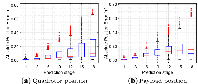
Fig. 13 Absolute position error for the 18 predicted stages of quadrotor and payload position when compared to measured true values for a point-to-point navigation task with a collinear dynamic obstacle
