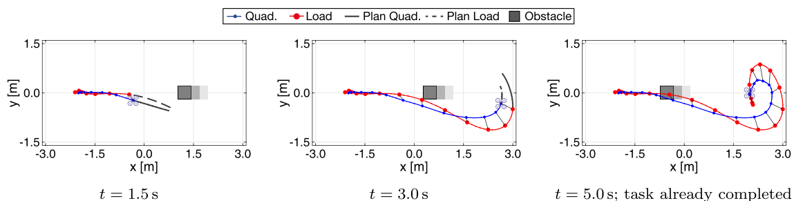
Fig. 21 Point-to-point navigation with collinear dynamic obstacle, N = 10 and assistive steering enabled; showing planned and executed trajectory and current quadrotor position. Notice how the steering guide
