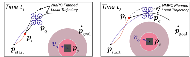
Fig. 3 System moves towards \mathbf{p}_{\text{goal}} with t_2 > t_1 ; planned local trajectory (grey) at the current time ( left ) that is updated in a future time ( right ) with the new state and obstacle data. Schematic projected top view with illustrative obstacle ellipsoids shown
