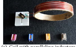
(a) Coil with paralleling inductors with different inductance
