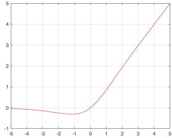
Fig. 3. Mish activation function
