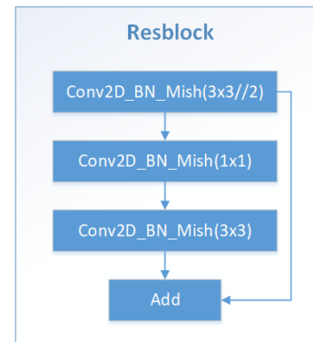
Fig. 4. Module Resblock
