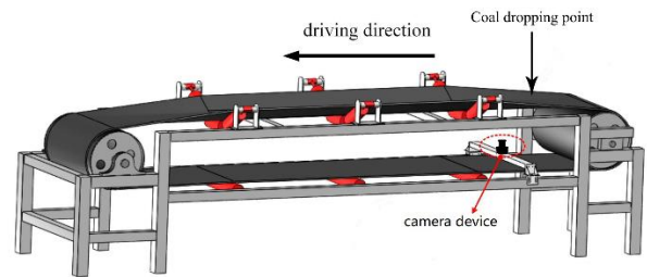
Fig. 10. Hardware installation location diagram
