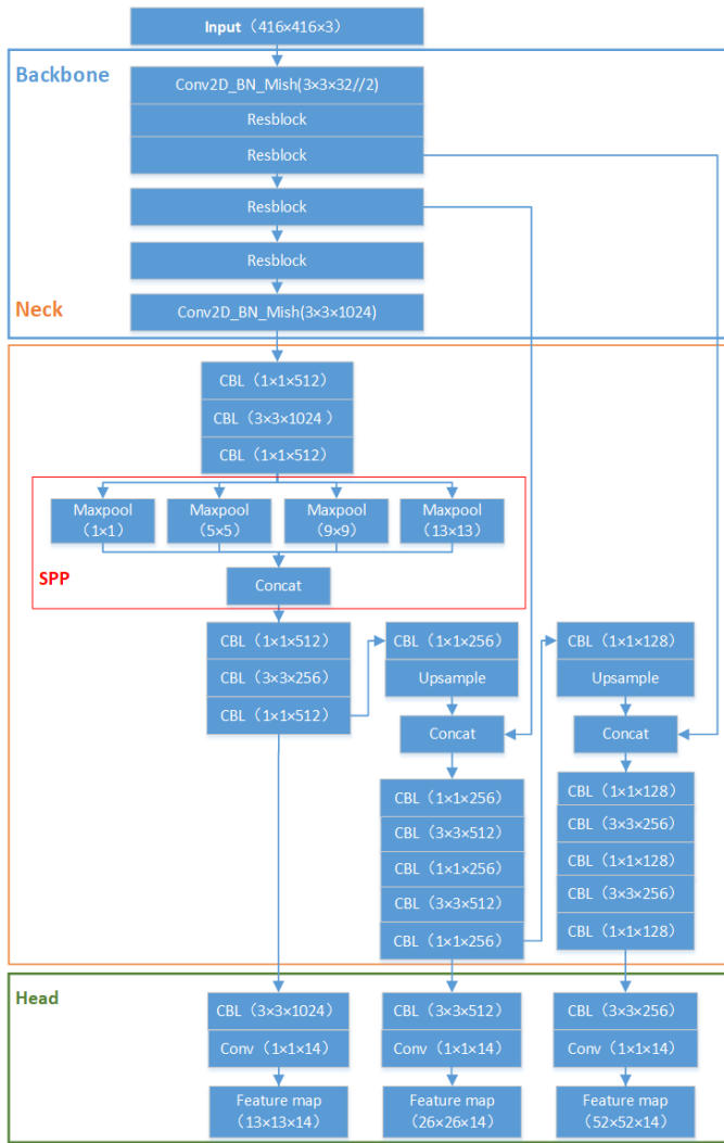
Fig. 2. ADCN structure
