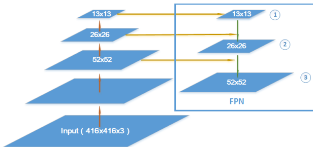
Fig. 6. FPN structure
