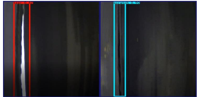
Fig. 13. The detection results under ADCN method
