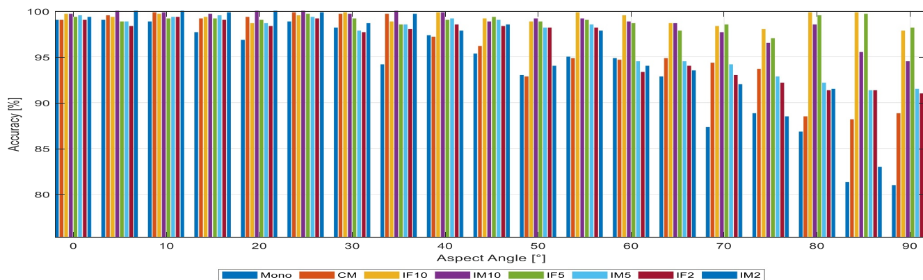
FIGURE 8 Comparison of the accuracy of the eight geometries (mono, CM, IF10, IM10, IF5, IM5, IF2, IM2) for all the activities for the scenarios where the aspect angle changes from 0^\circ to 90^\circ with 5^\circ steps. The IM configuration outperforms slightly or equates the IF configuration for angles up to 55^\circ for overall accuracy. The tendency changes to IF outperforming slightly or equating IM up to 70^\circ and then at high aspect angles IF clearly outperforms the IM configuration. IF10 maintains an accuracy of over 97.58% (94.5% for IM10) overall and 97.08% with IF5 (91.3% for IM5). Even with a reduction in the baseline, the IF radar maintains good performance at high aspect angles
