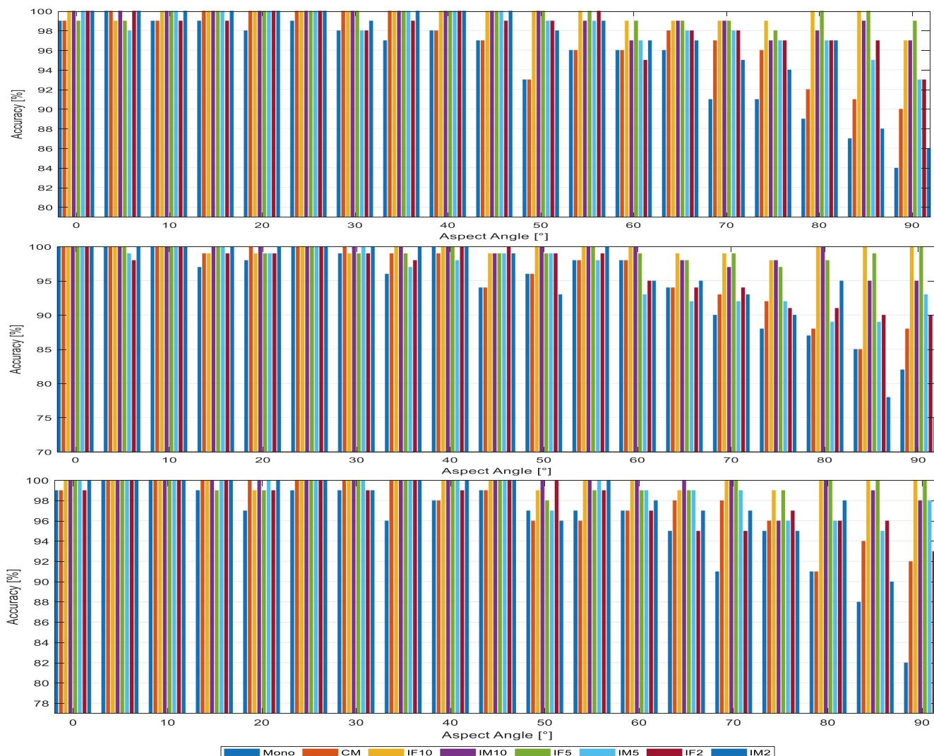
FIGURE 6 Comparison of the accuracy of the eight geometries (mono, CM, IF10, IM10, IF5, IM5, IF2, IM2) for: (a) activity I—the IF configuration dominates in high aspect angles ( >55^\circ ) and IM and IF have 100% recognition up to 50^\circ , (b) activity II—the IF configuration dominates or equates IM in high aspect angles ( >45^\circ ), and IM dominates or equates IF up to 40^\circ and (c) activity III—the IF configuration dominates or equates IM in high aspect angles ( >65^\circ ), and IM dominates or equates IF up to 65^\circ for the scenarios where the aspect angle changes from 0^\circ to 90^\circ with 5^\circ steps
