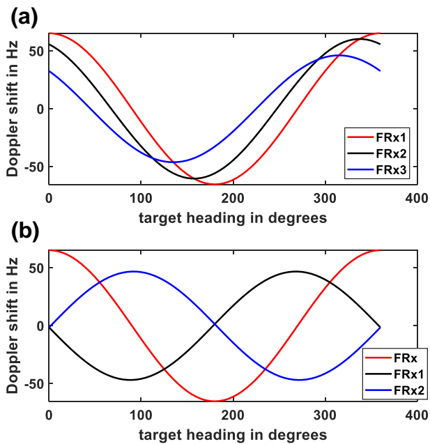
FIGURE 3 The expected Doppler shifts for: (a) the CM configuration with nodes at 0^\circ , 45^\circ and 90^\circ and (b) the in-line configuration with a 10 m baseline ( Rx_1/Rx_2 have the same Doppler shifts in the interferometric case) for a carrier frequency of 9.8 GHz
