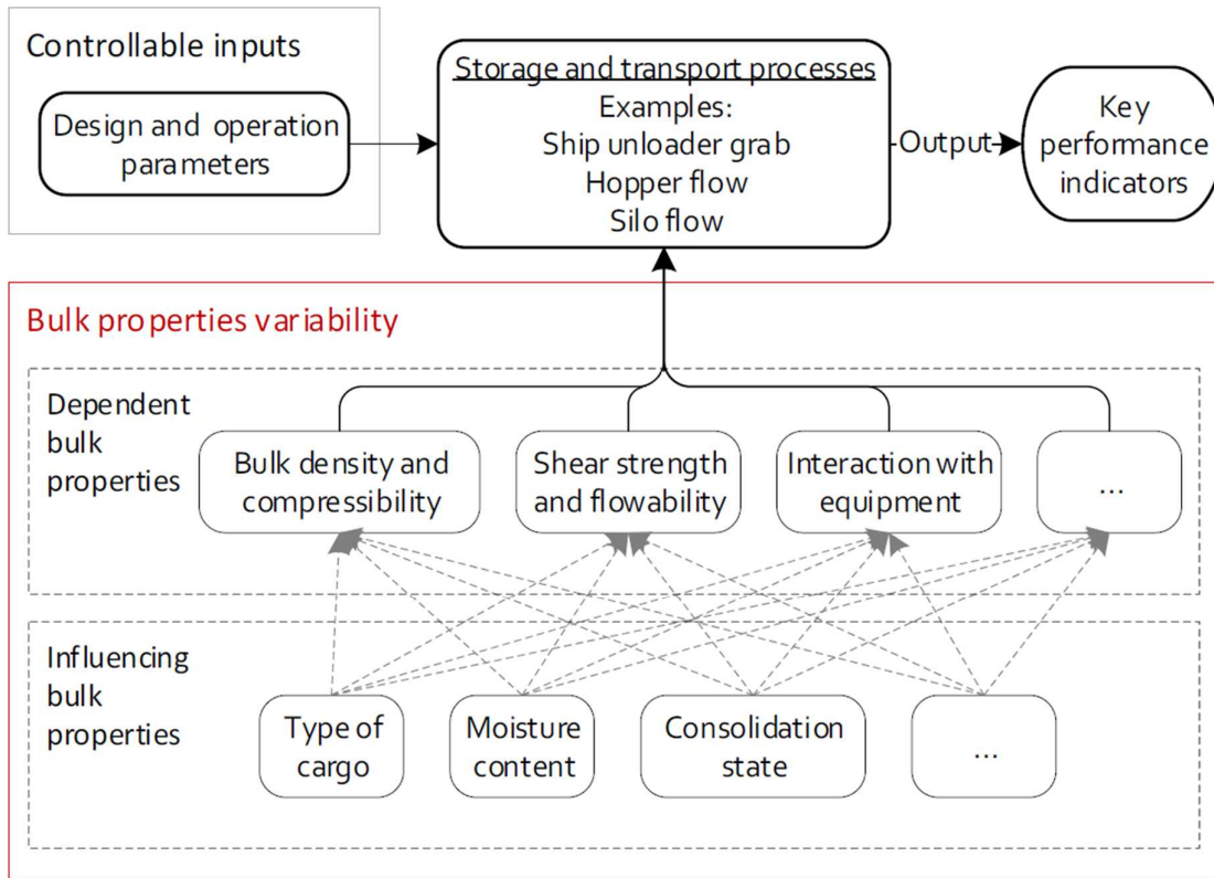
Figure 3-1. Controllable and uncontrollable inputs in bulk storage and transport processes, including ship unloader grabs
