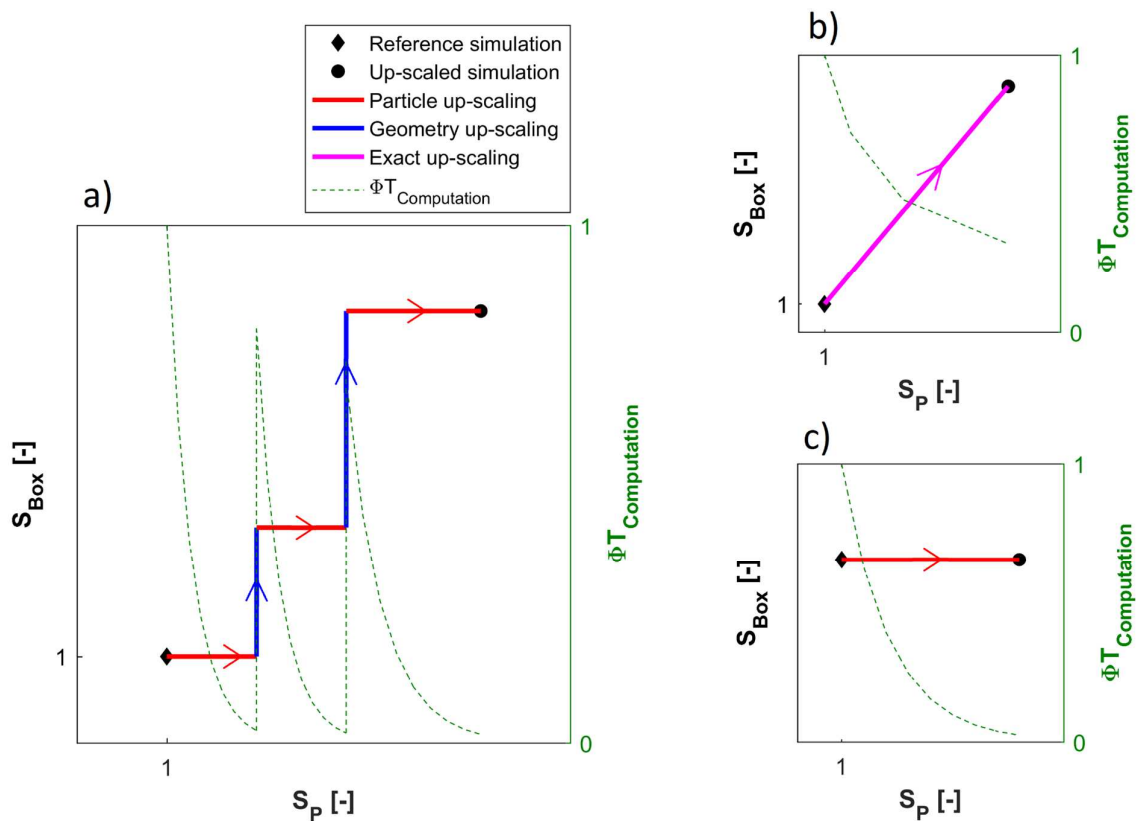
Figure 4-6. Scaling approaches, (a) hybrid particle-geometric scaling approach (b) Exact Scaling, and (c) particle upscaling
