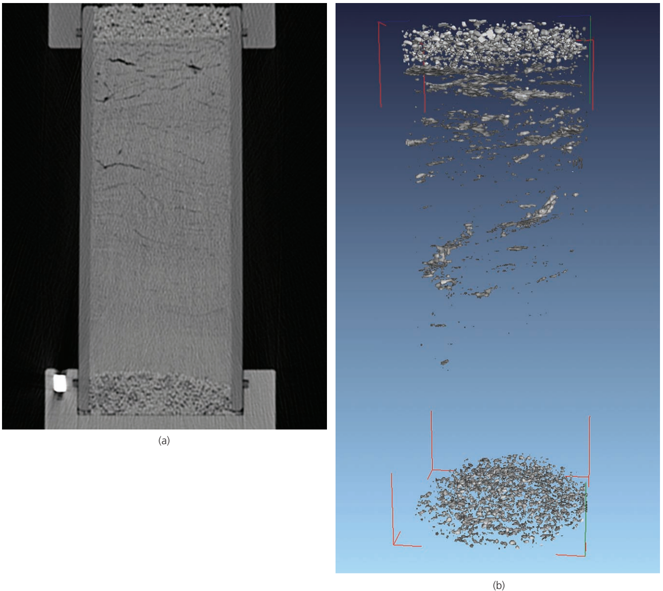
Figure 8. Result of the gas distribution in the sand column treated at ambient pressure with multiple substrate flushes: (a) X-ray CT scanned images; (b) constructed three-dimensional image
