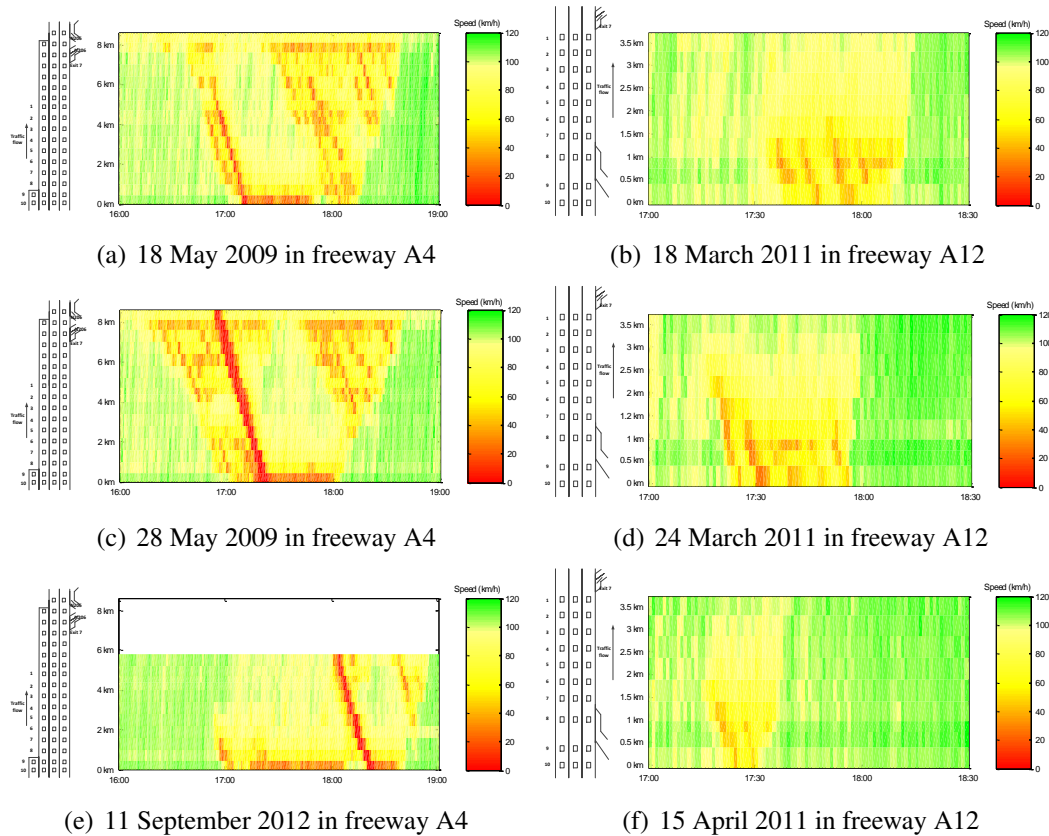
Figure 3.4: Speed contour plots of study traffic situations on freeway A4 (a, c, e) and freeway A12 (b, d, f).
