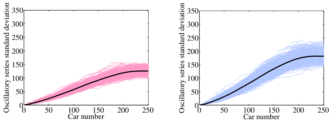
(a) Standard deviation of oscillatory series with v_{\text{lead}} = 30 km/h.
