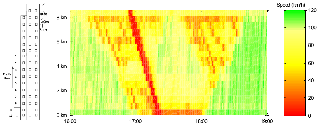
(b) Speed contour on 28 May 2009
