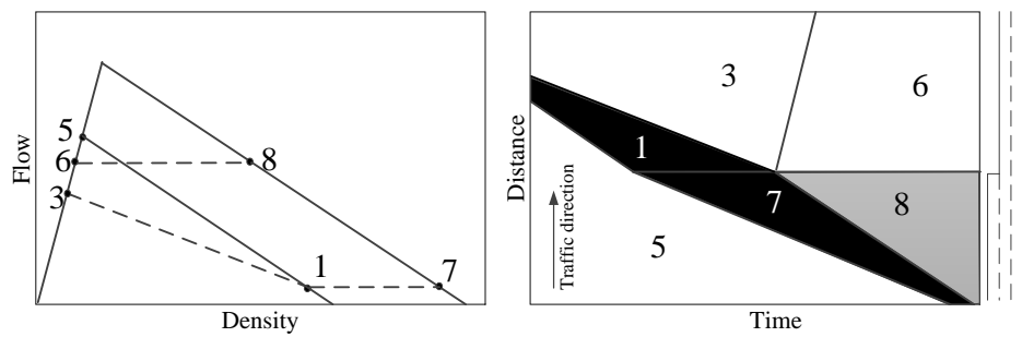
(c) Case 3: Lane-drop node scenario
