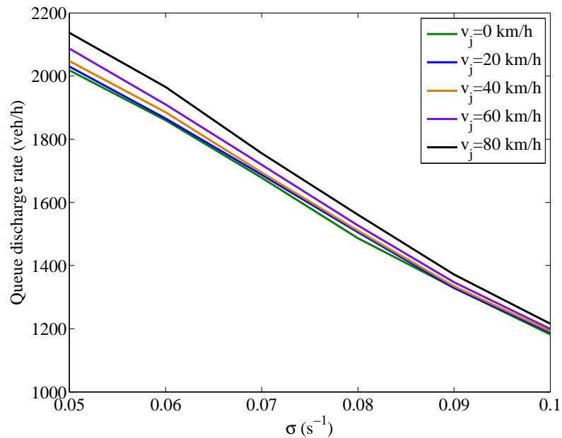
(b) Sensitive analyses of parameter \sigma with \beta = 0.07s^{-1} and N = 441 veh.
