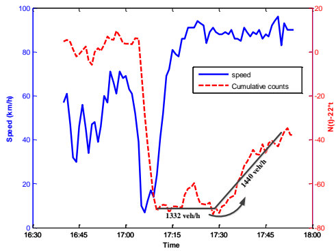
(f) Shoulder lane, location 1, 28 May 2009
