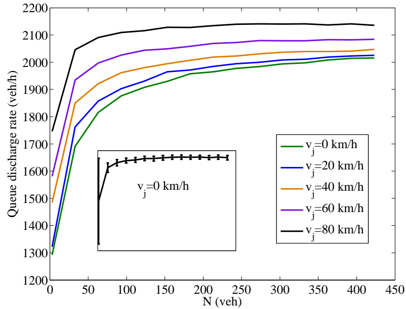
(a) Sensitive analyses of parameter N with constant \beta = 0.07s^{-1} and \sigma = 0.05s^{-1/2} .
