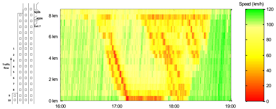
(a) Speed contour on 18 May 2009
