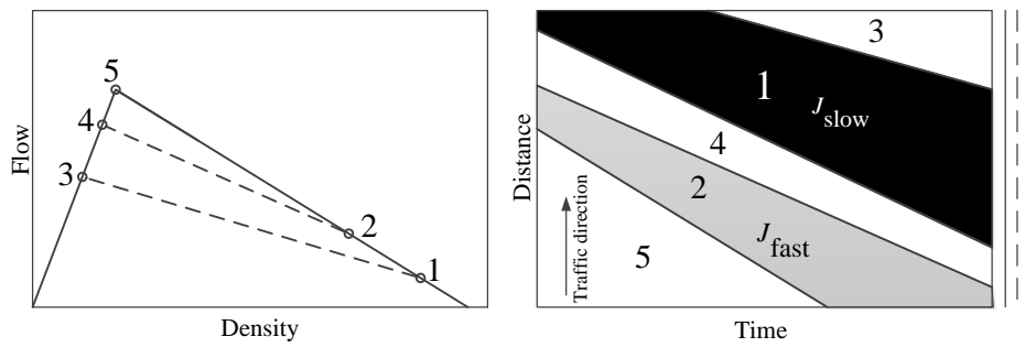
(b) Case 2: Heavy congestion J_{slow} downstream
