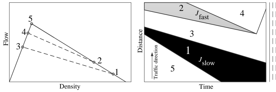
(a) Case 1: Heavy congestion J_{slow} upstream
