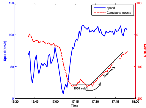
(b) Median lane, location 1, 28 May 2009
