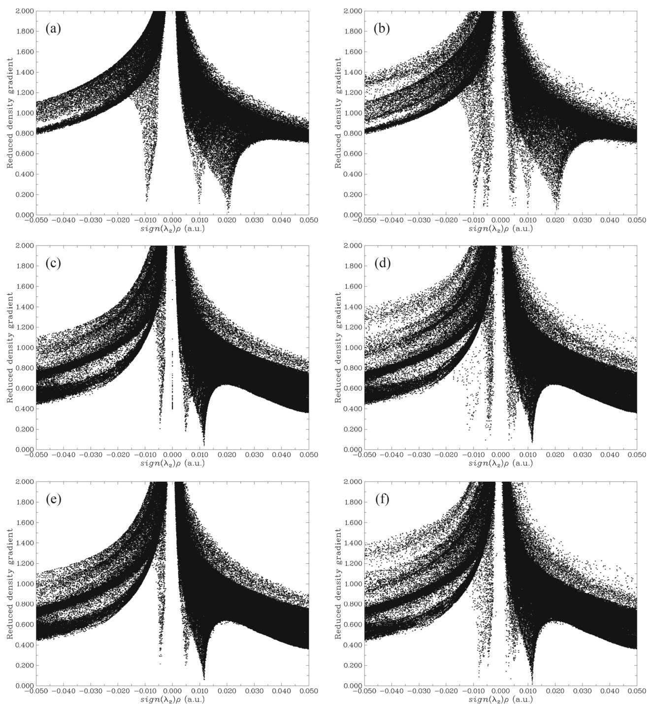
Figure 7. RDG (Y-axis) vs. \text{sign}(\lambda_2)\rho(r) (X-axis) plots for (a) CNT, (b) HCFC-124/CNT complex, (c) SiCNT, (d) HCFC-124/SiCNT complex, (e) SiCGeNT and (f) HCFC-124/SiCGeNT. The results are obtained at the \omega B97XD/6-311G(d) level of theory.
