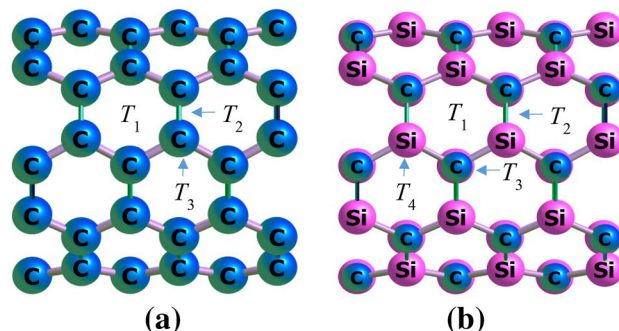
Figure 1. Unit cells of (a) carbon nanotube (CNT) and (b) silicon carbide nanotube (SiCNT).
