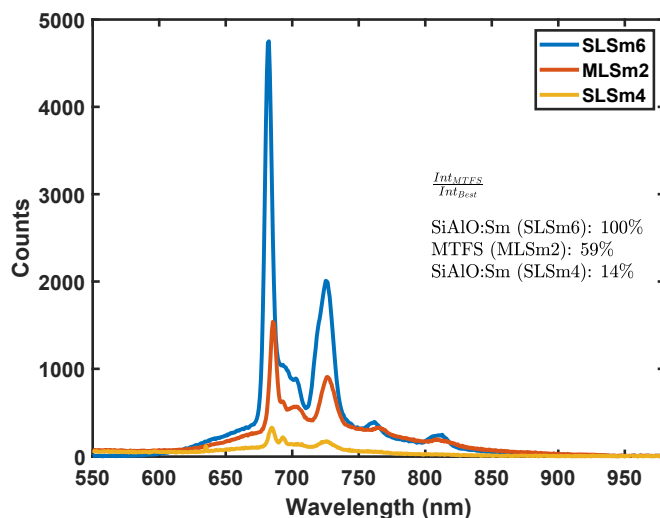
Fig. 8. Comparison of the photoluminescence emission intensity between samples SLSm6 (blue), MLSm2 (red), and SLSm4 (yellow) excited at 375 nm. The numbers in the inset compare the total integrated intensity (between 550 and 950 nm) of each sample with the PL intensity observed in SLSm6.
