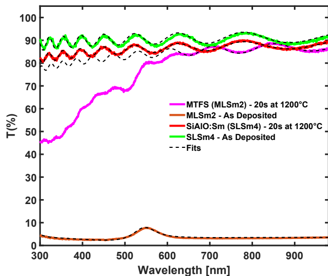
Fig. 7. Comparison of transmittance among one reactively co-sputtered SiAlO:Sm single-layered thin-film (SLSm4) and a MTFP (MLSm2), before and after rapid thermal annealing. See Table 2 for further details about the deposition conditions used for each sample.
