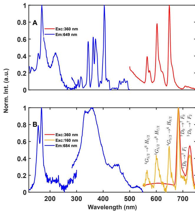
Fig. 2. PL and PLE spectra for phosphor A) SGSm and B) SLSm3, both recorded at T = 10 K. All spectra are normalized with respect to their maxima. The excitation spectrum was obtained using a deuterium light source from 120 to 300 nm combined with a xenon light source from 280 to 550 nm.
