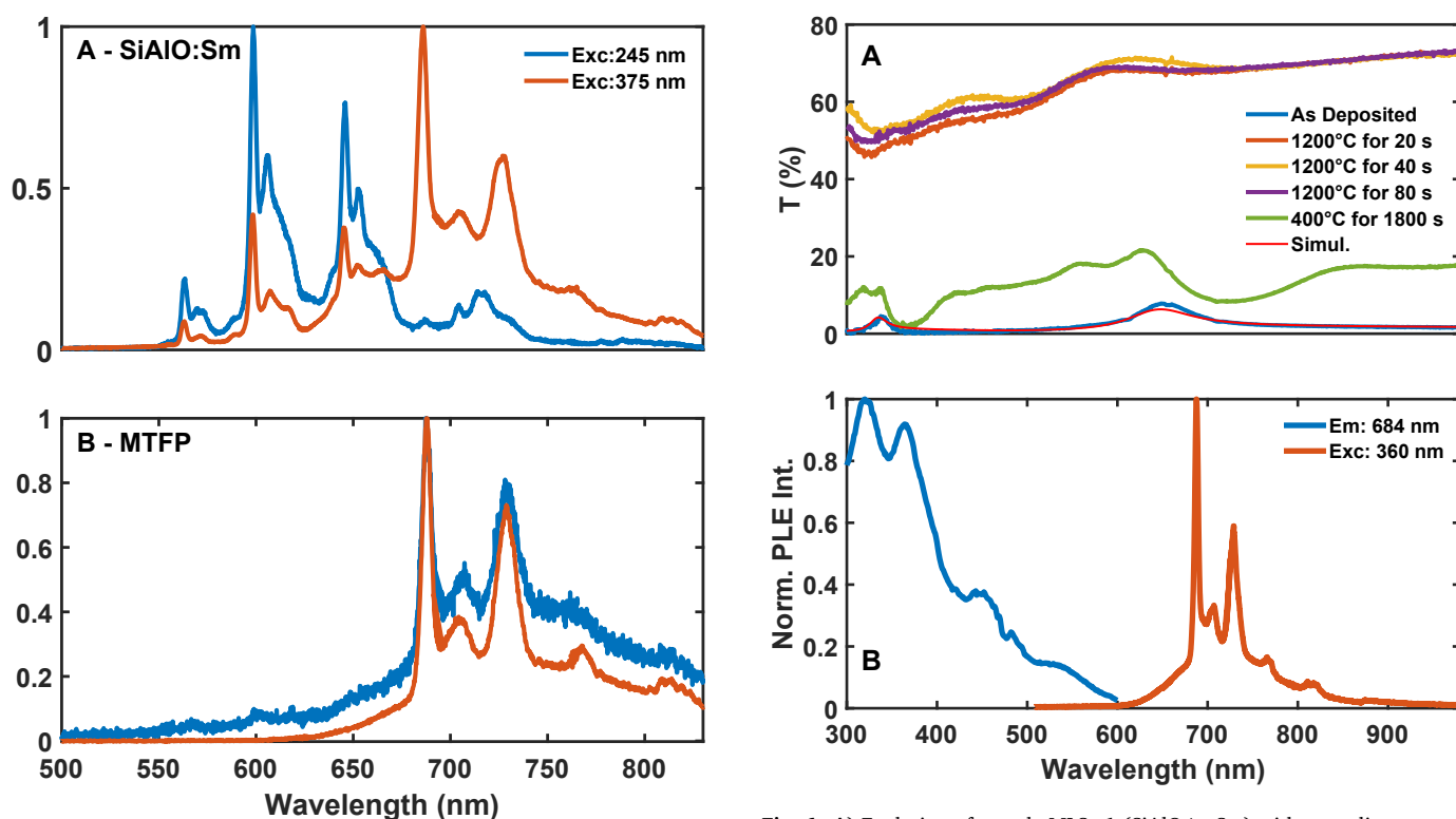
Fig. 6. A) Evolution of sample MLSm1 (SiAlO/m-Sm) with annealing temperature and time. The sample becomes transparent with higher annealing temperature and slightly changes with longer annealing times at 1200 °C. In blue is MLSm1 in as-deposited state and, in red, is the transmittance simulated by RefFIT of 7 SiAlO 190 nm-thick layers interspersed with 7 metallic Sm 11 nm-thick layers. See supplementary information for more details on these simulations. B) Normalized excitation and emission photoluminescence spectra of sample MLSm1 after annealing treatment.
