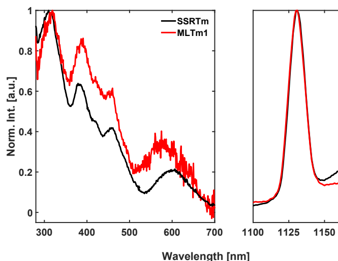
Fig. 9. (Left) Normalized photoluminescence excitation spectra of SSRTm (black) and MLTm1 (red) obtained by monitoring the emission at 1130 nm. (Right) Normalized photoluminescence emission spectra of the same samples in black and red (excitation at 470 nm). Further data acquisition details are in section 2.3.
