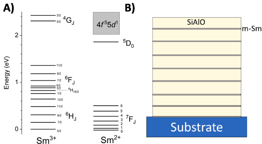
Fig. 1. A) Schematic energy level diagram of both \text{Sm}^{3+} (left) and \text{Sm}^{2+} (right) associated with the transitions in the visible range of the spectrum. The lines represent 4f^6 states whereas the rectangle represents a combination of broad 4f^55d^1 states. Energy values from Ref. [13]; B) Schematic representation of one multilayered thin-film structure. The structure is composed of Ln layers, sputtered using metallic conditions on the m-Ln target, interspersed with SiAlO layers, reactively sputtered using fully oxidized Si and Al targets.
