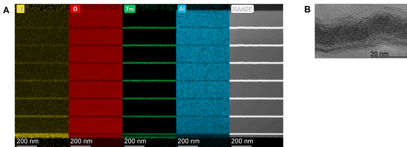
Fig. 4. TEM-EDX cross section maps of 7 layered SiAlO/m-Tm MTFP (sample MLTm2) in as-deposited state. A) From left to right: EDX maps of Si, O, Tm, Al, and ADF TEM image. B) Typical high resolution TEM image of one Tm layer grown by igniting only the Tm target in metallic mode. Notice layer irregularities and the presence of Tm-related nano-crystalline structures.
