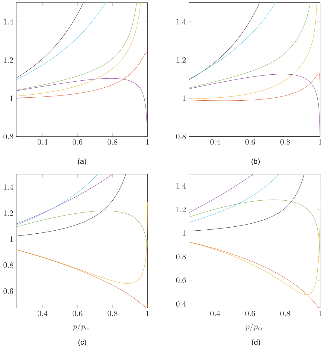
FIG. 3. Variation of fluid properties along the critical isotherm for several fluids, where \infty denotes the properties estimated at v \rightarrow \infty . (a) nitrogen, (b) \text{CO}_2 , (c) toluene, and (d) siloxane MM. Fluid parameters: Black line \gamma/\gamma_\infty , blue line \gamma_{pv}/\gamma_{pv,\infty} , orange line \Gamma/\Gamma_\infty , yellow line G/G_\infty , purple line \Psi/\Psi_\infty , and green line 1/Z .
