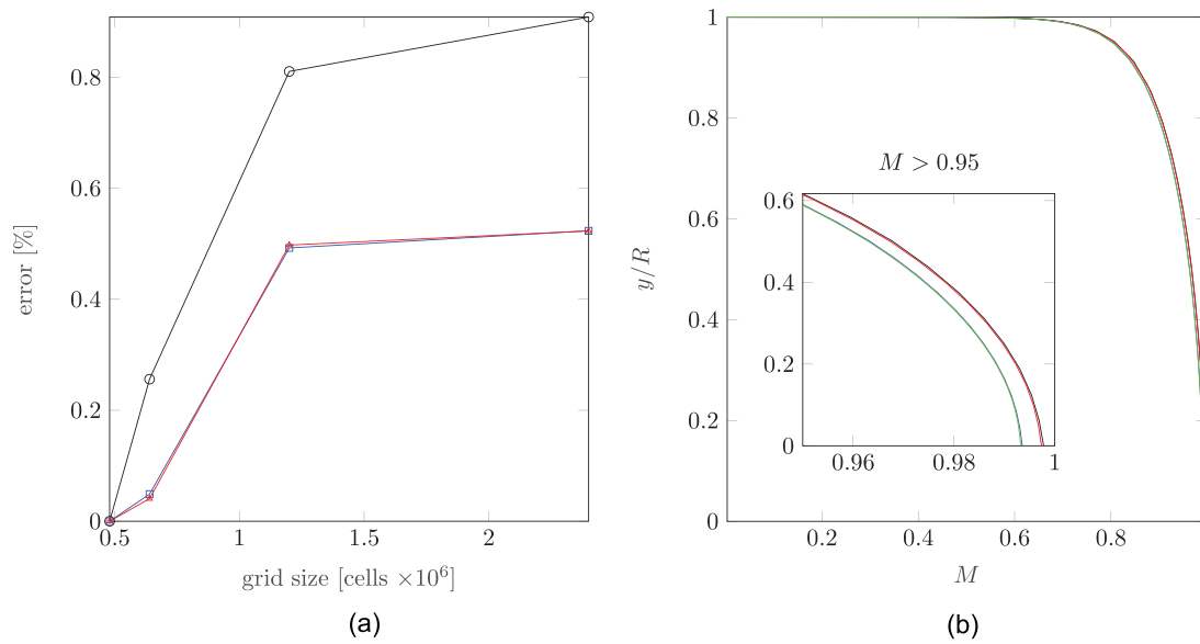
FIG. 16. Grid independence study. (a) Relative deviation, as a function of the computational mesh size, of the values of C_f , M , and Re_D from the ones computed using the coarsest mesh of 480 000 cells. Each variable is calculated with a mass flow average over the outlet section of the pipe. (b) Mach number at the outlet pipe section vs normalized radial coordinate for four different computational grids. Grid size: black line: 480 000, red line: 640 000, blue line: 1.2M, green line: 2.4M. A close-up of the Mach profile in proximity of the pipe centerline is also displayed.
