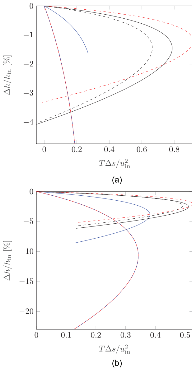
FIG. 11. Fanno curves in the non-dimensional h-s thermodynamic plane for different fluids at fixed inlet Mach number, M_{in} = 0.7 . The considered fluids can be identified with the colors and markers reported in Table IV. Two sets of inlet reduced temperatures and pressures are reported: (a) T_r = 1.05 , p_r = 1.15 ; and (b) T_r = 0.9 , p_r = 0.05 .
