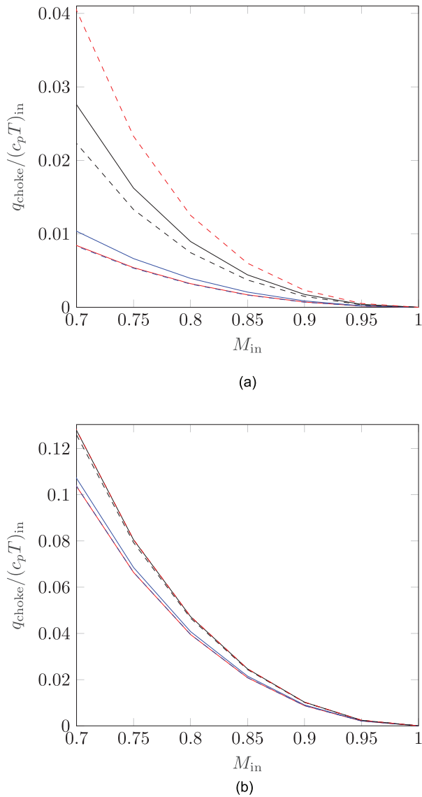
FIG. 7. Non-dimensional energy transfer as heat required to attain choked conditions as a function of the inlet Mach number. Markers and colors identifying the curve in relation to each fluid are reported in Table IV. Considered cases: (a) T_r = 1.05 , p_r = 1.15 ; and (b) T_r = 0.9 , p_r = 0.05 .
