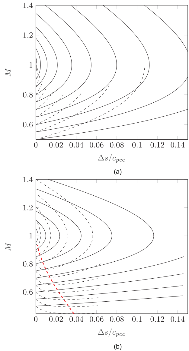
FIG. 8. Mach number vs entropy in Rayleigh processes in (a) nitrogen and (b) siloxane D 6 for different inlet Mach numbers. Two sets of inlet reduced temperature and pressures are considered: --- T_r = 1 , p_r = 0.9 ; — T_r = 0.9 , p_r = 0.05 . The red line identifies the locus of M_{\min} .
