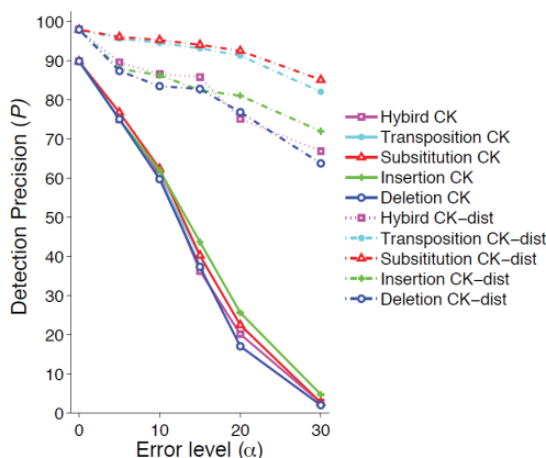
Supplemental figure S2.3: We tested four extreme cases of experimental error. (Light blue) 100% errors are due to transposition. (Red) 100% errors are due to substitution. (Green) 100% errors are due to insertion. (Blue) 100% errors are due to deletion. Solid lines are for CK fingerprinting. Dotted lines are for CK-dist fingerprinting.
