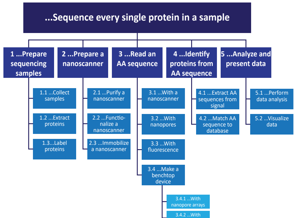
Figure 6.2: The technology tree unbundles the underlying technologies necessary for Single-Molecule Protein Sequencing.
