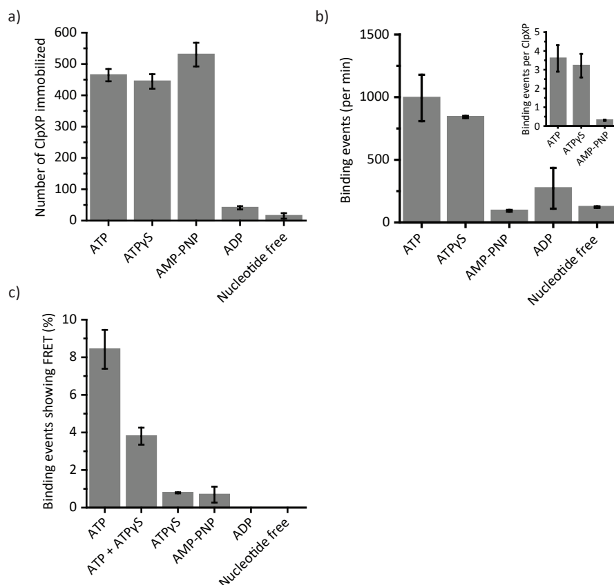
Figure 4.2: (a) Number of ClpXP complexes immobilized on the surface in under different nucleotide conditions. (b) The total number of acceptor-labeled substrates binding to donor-labeled ClpXP complexes over time. The inset shows the binding events per minute normalized to the number of immobilized ClpXP complexes. Error bars are SEM obtained from 10 measurements. (c) The percentage of binding events resulting in translocation of the substrate defined as traces showing a peak in FRET efficiency as shown in Figure 4.1c .
