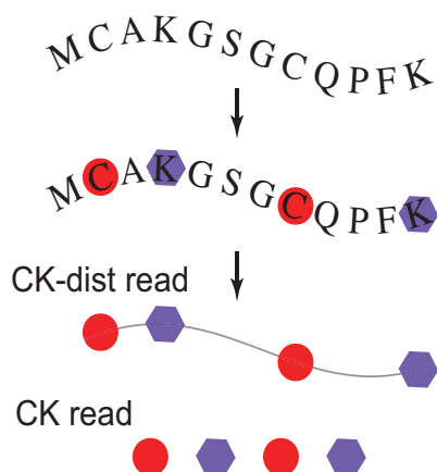
Figure 2.1: A single-molecule read-out. CK fingerprinting read: the order of C's and K's are detected. CK-dist fingerprinting read: the distances between C's and K's are additionally measured.
