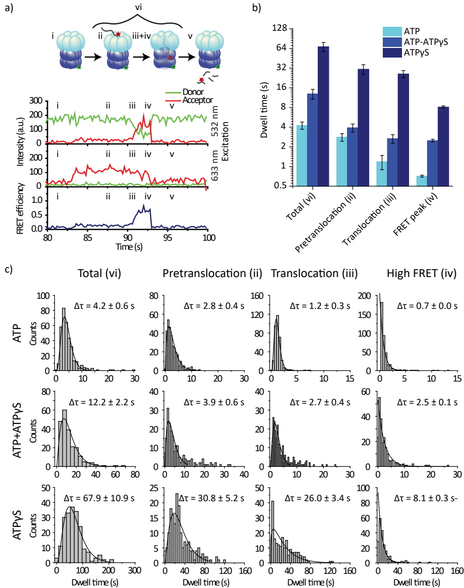
Figure 4.3: (a) A typical time trace representing a successful translocation event. i) High donor intensity reports on the presence of immobilized and labeled ClpXP. ii) Binding of an acceptor-labeled substrate results in a sudden increase in signal after direct acceptor excitation. iii) The pretranslocation phase is determined as the time a substrate remains bound to ClpXP prior to translocation. iv) Translocation of a substrate by ClpXP results in a gradual increase in FRET efficiency. v) Release of the substrate is indicated by a sudden decrease in FRET coinciding with a sudden decrease of direct acceptor excitation signal. vi) Represents the total time it takes for a substrate to be processed by ClpXP. (b) The dwell times of the
