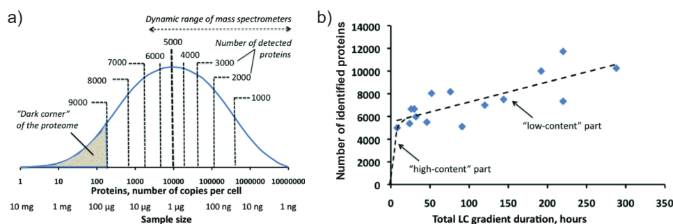
Figure 6.1: (a) Conventional proteomics analysis detects highly abundant proteins and stretches for about four orders of magnitude. Deeper proteome analysis requires much larger sample size. The “dark corner” represents part of the proteome that is most challenging for detection. (b) Analysis of the first approximately 5000 proteins is very fast, while deeper analysis yields on average <20 additional proteins per hour of LC gradient. (Figures adapted from (11)).
