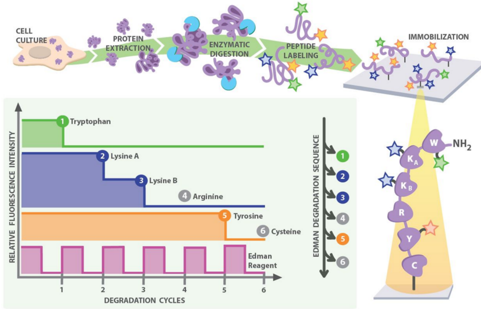
Figure 1.3: Schematic representation of fluorescence-based protein sequencing with Edman degradation. (Figure adapted from (46)).
