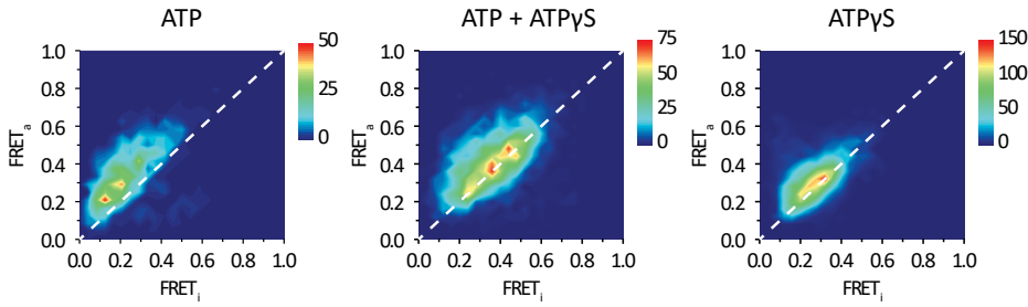
Figure 4.4: Transition density plots. FRET change was analyzed by measuring FRET i at t = \tau and FRET a at t = \tau + \delta\tau , with \delta\tau = 0.4 s, for every time point at stage (iii) (see Figure 4.3a for the schematic) and was deposited in a 2D distribution plot. The dotted line represents FRET i = FRET a . The transition density plots were obtained for ATP, ATP+ATP γ S and ATP γ S. In the presence of ATP, FRET a \geq FRET i , indicating a forward movement of ClpXP. For ATP+ATP γ S and ATP γ S on the other hand, FRET a < FRET i was observed, indicating backward movement of ClpXP along the substrate.
