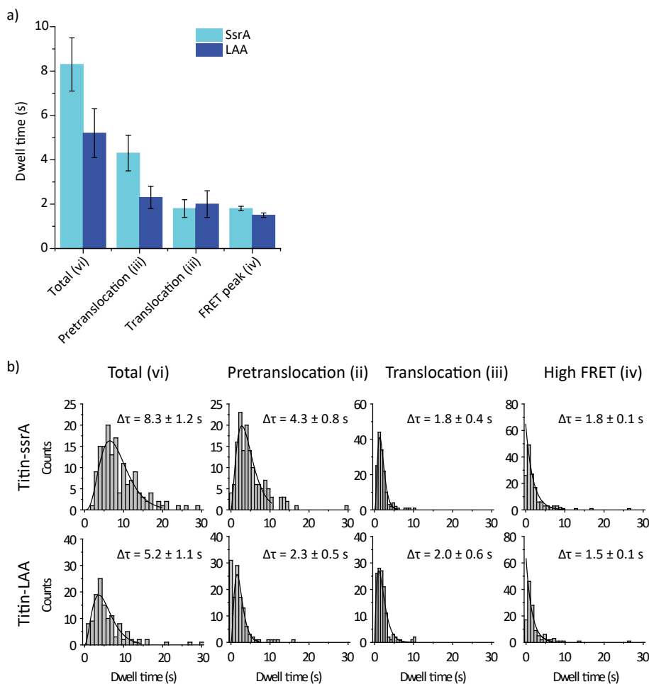
Figure 4.6: (a) The dwell times of the individual features in the traces as described in Figure 4.3a were determined for titin-ssrA and titin-LAA. (Error bars were obtained by bootstrapping with 1000 resamples.) (b) Dwell time histograms underlying the bar graphs in Figure 4.6a . (Error were obtained by bootstrapping with 1000 resamples.)
