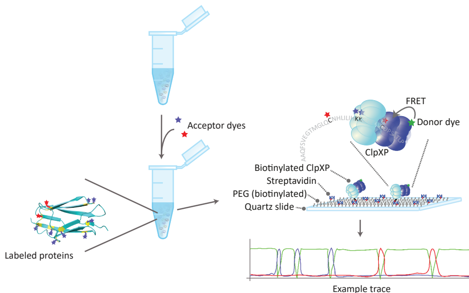
Figure 1.4: Schematic representation of the single-molecule protein fingerprinting technique further described throughout this thesis.
