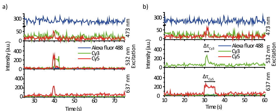
Supplemental figure S3.2: (a) The original time trace used in Figure 2b to present a three-color FRET event. Note the original, not summed up, levels of Cy3 and Cy5 signals in the middle panel. (b) A substrate was labeled with Cy5 fluorophore at the N-terminal end and with Cy3 internally. A typical time trace obtained from a three-color ALEX measurement showed a colocalized signal from Cy3 (middle trace) and Cy5 (bottom trace) excitation. For presentation of multiple traces with clarity, we introduced an arbitrary offset of 200 A.U. to the Alexa488 trace (top) and plotted the sum of the signals from Cy3 and Cy5 upon 532 nm excitation (middle).
