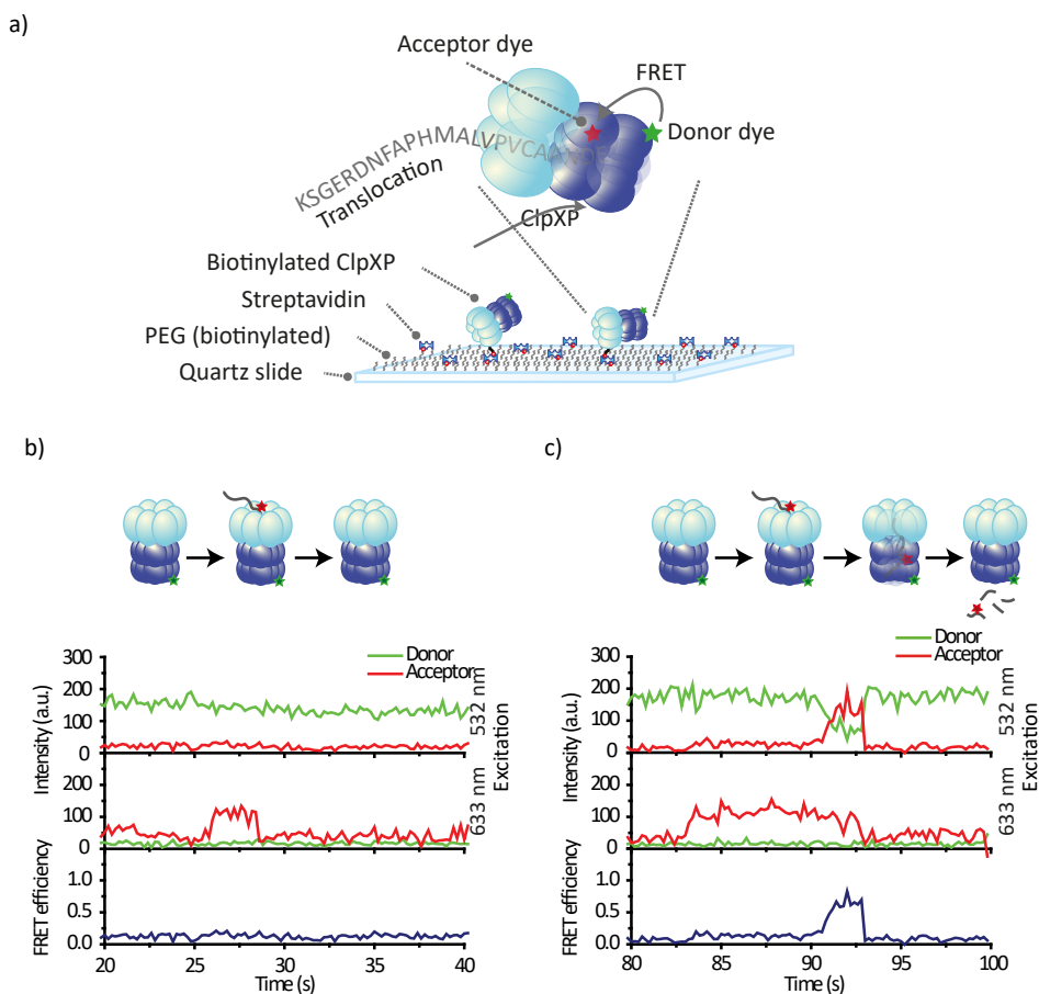
Figure 4.1: (a) Schematic representation of the single-molecule FRET assay. Donor labeled ClpXP is immobilized on a passivated quartz slide via biotin-streptavidin interactions. Acceptor labeled substrates with ClpX recognition tags are introduced to the fluidic chamber. ClpX will recognize and translocate the substrate into the ClpP chamber, where FRET will occur between acceptor fluorophore and donor fluorophore. (b) A typical time trace of a binding event obtained using ALEX. The donor signal is from Cy3-labeled ClpXP ( Figure 4.1b , upper graph). The sudden appearance of acceptor signal during acceptor-direct excitation indicates binding of acceptor-labeled substrate to ClpXP ( Figure 4.1b , middle graph). Loss of signal is the release of the substrate. (c) typical time trace for binding events resulting in translocation. Similar to Figure 4.1b , the sudden increase in acceptor signal after direct excitation ( Figure 4.1c , middle graph) reports on binding of a substrate to ClpXP. Translocation into the ClpP chamber is represented by a gradual increase in FRET ( Figure 4.1c , lower graph).
