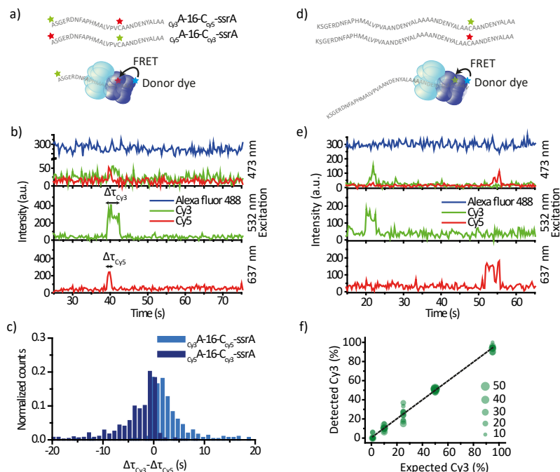
Figure 3.2: (a) Substrates (A-16-C-ssrA, Supplemental table S3.1 ) were labeled with Cy3 fluorophore at the N-terminal end and with Cy5 internally. (b) A typical time trace obtained from a three-color ALEX measurement showed FRET between Alexa488 and Cy3; and Alexa488 and Cy5 (top trace) and a colocalized signal from Cy3 (middle trace) and Cy5 (bottom trace) excitation. For presentation of multiple traces with clarity, we applied an arbitrary offset of 200 A.U. to the Alexa488 trace (top). We also plotted the sum of the signals from Cy3 and Cy5 upon 532 nm excitation (middle). For the original trace, see Supplemental Figure S2a. (c) Comparison of the dwell times of the two acceptor signals. We subtracted the dwell time of Cy5 ( \Delta\tau_{\text{Cy5}} ) from the dwell time of Cy3 ( \Delta\tau_{\text{Cy3}} ) for each event (blue). The same analysis was made for a construct that had the two acceptors swapped (black). (See also Supplemental Figure S2b) Approximately 900 events from three independent experiments were used for each analysis. (d) Substrates (K-38-C-ssrA) were labeled with either Cy3 or Cy5 (acceptors). (e) A representative time trace of three-color FRET. Two batches of polypeptides labeled with either Cy3 or Cy5 were mixed in different ratios. Both Cy3 and Cy5 labeled polypeptides showed FRET (top). At t \sim 20 s a Cy3-labeled substrate binds, as reported by Alexa488-Cy3 FRET (top) and 532nm direct excitation (middle). At t \sim 50 s, a Cy5-labeled substrate binds reported by Alexa488-Cy5 FRET (top) and 637nm direct excitation (bottom). For presentation of multiple traces with clarity, we applied an arbitrary offset of 200 A.U. to the Alexa488 trace. (f) The percentage of processed Cy3-labeled substrates compared to the total number of all processed substrates was plotted against the expected percentage of Cy3-labeled substrate in the mixture. Each dot is based on a 100 sec measurement and represents between 8 and 57 translocation events. The number of events is represented by the size of the dot. The solid black line is a linear fit (slope of 0.99 \pm 0.02 , intercept 0.44 \pm 0.77 , R^2 = 0.99 ).
