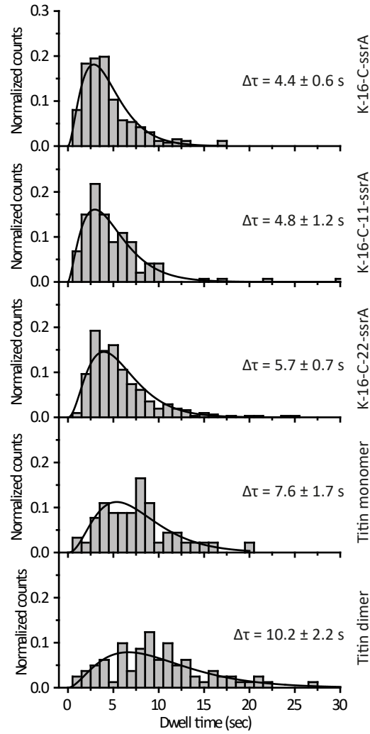
Supplemental figure S3.3: Total dwell times (stages ii + iii; see Figure 3.1b for schematic) were determined for ssrA-tagged polypeptides of increasing lengths and monomeric and dimeric titin. Total dwell times for all substrates showed gamma-like distributions. Errors were obtained by bootstrapping with 1000 resamples.
