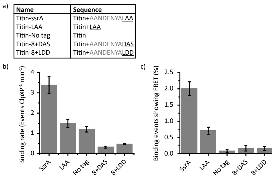
Figure 4.5: (a) SsrA tag mutants used in this study. The underlined amino acids are interacting with the ClpX pore to initiate binding and translocation. (b) The total number of acceptor-labeled substrates binding per donor-labeled ClpXP complexes per minute. Error bars are SEM obtained from 10 measurements. (c) The percentage of binding events resulting in translocation of the substrate defined as traces showing a peak in FRET efficiency as shown in Figure 4.1c .
