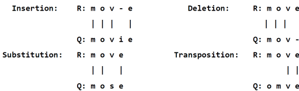
Figure 2.4: Expected experimental errors. ‘R’ is reference sequence. ‘Q’ is query sequence.
