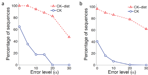
Supplemental figure S2.6: Percentage of (a) HRSV and (b) TB proteins whose CK fingerprints are absent in human at various error levels. Blue line for CK fingerprints, red line for CK fingerprints with distance information. The higher the percentage, the more HRSV/TB proteins show unique CK fingerprints against human proteins.
