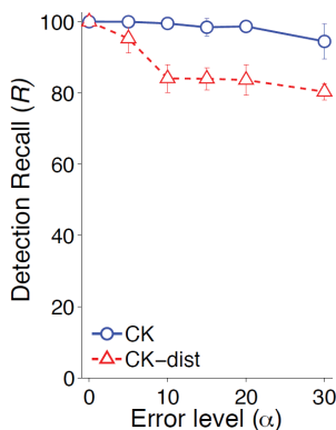
Supplemental figure S2.4: R at various error levels: blue for CK fingerprints, red for CK fingerprints with distance information (CK-dist fingerprinting).
