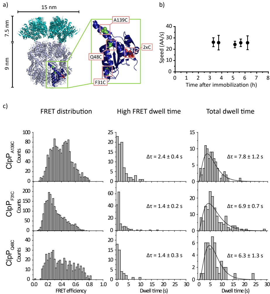
Supplemental figure S3.1: (a) Crystal structure of ClpXP. It was obtained by manually combining crystal structures from PDB:1YG6 and PDB:3RY2. Highlighted in red are the two cysteine residues present in wildtype ClpP. Highlighted in green are cysteines introduced in three mutants. (b) The translocations speed versus the time of the experiment after ClpXP immobilization. Data obtained from a single flow chamber. ClpXP translocation speeds remained the same up to 6 hours after immobilization. (c) FRET and dwelltime analysis. For our sequencing scheme to work, FRET events we observe should be distinct from background signals. Time trajectories showing successful translocation of acceptor (Cy5) labeled titin were selected. (Left) FRET distributions of stage iii (see Figure 3.1b for schematic) were
