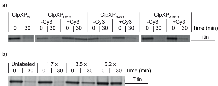
Figure 5.3: (a) Degradation assay of titinV13P-ssrA by ClpXP. Degradation capacity of unlabeled and labeled ClpP mutants was compared to wild-type ClpP. (b) Degradation assay of titinV13P-ssrA by ClpXP with increasing labeling efficiencies. ClpPF31C showed reduced degradation efficiency with increasing labeling efficiency.
