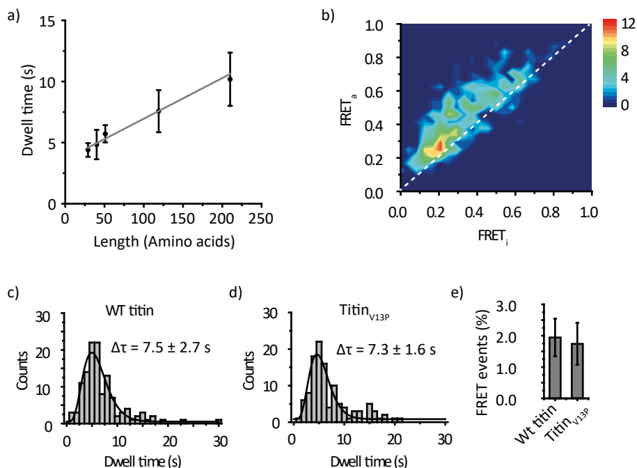
Figure 3.3: (a) Dwell times vs. length of the substrate. Total dwell times were obtained from fitting data in Supplemental Figure S3 with gamma distributions. Five different substrates were used: K-16-C-ssrA ( n = 227 ), K-16-C-11-ssrA ( n = 131 ), K-16-C-22-ssrA ( n = 290 ), titin monomer ( n = 85 ), titin dimer ( n = 81 ). Error bars were obtained by bootstrapping with 1000 resamples. Fitting the data with a linear curve results in an offset of 3.6 \pm 0.3 s and a speed of 30.1 \pm 4.0 AA/s. (b) Transition density plot. FRET change was analyzed by measuring \text{FRET}_{\text{initial}} at t = \tau and \text{FRET}_{\text{after}} at t = \tau + \delta\tau , with \delta\tau = 0.4 s, for every time point at stage (iii) (see Figure 3.1b for the schematic) and was deposited in a 2D distribution plot. The dotted line represents \text{FRET}_{\text{initial}} = \text{FRET}_{\text{after}} . A peptide substrate (K-38-C-ssrA) was used. (c) and (d) Total dwell times (stages ii + iii) (see Figure 3.1c for the schematics) for wild-type titin and titin V13P . For wild-type titin and titin V13P , \Delta\tau = 7.5 \pm 2.7 s and 7.3 \pm 1.6 s were obtained respectively by fitting with a gamma distribution. Errors were obtained by bootstrapping with 1000 resamples. Wild-type titin, n = 123 . titin V13P , n = 112 . (e) The percentage of traces showing FRET events for both wild-type titin and titin V13P . Error bars are standard deviations based on 15 measurements.
