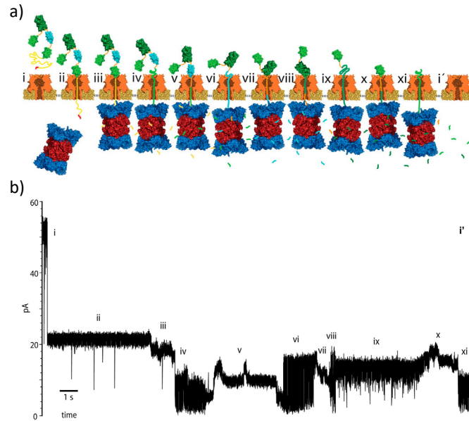
Figure 1.1: (a) Working model of ClpXP mediated protein translocation through a biological nanopore. (b) Representative current blockage profile revealing domain specific signals during ClpXP mediated translocation. (Figures adapted from (25)).
