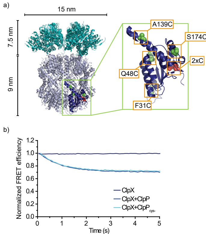
Figure 5.1: (a) Crystal structure of ClpXP (obtained by manually combining crystal structures obtained from 1YG6 and 3RY2) with highlighted in red the two cysteines present in wildtype ClpP and highlighted in green positions were cysteines were introduced in the three mutants. (b) Fluorescence-based activity assay to evaluate the activity of ClpXP. In the absence of ClpP, there is no degradation and the curve is flat. In the presence of ClpP, both wild-type and cys- mutant, a decrease in FRET efficiency is observed, indicating degradation of our model substrate.
