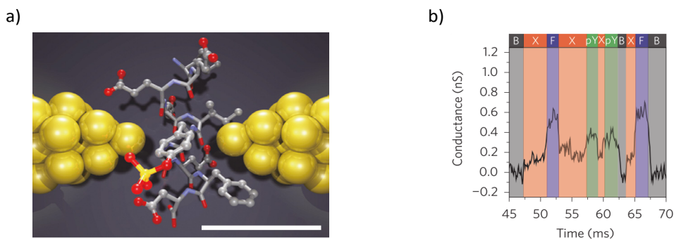
Figure 1.2: (a) Schematic representation of tunneling current measurements (Figure adapted from (35)). (b) Example trace with conductance levels assigned to individual amino acids (Figure adapted from (36)).
