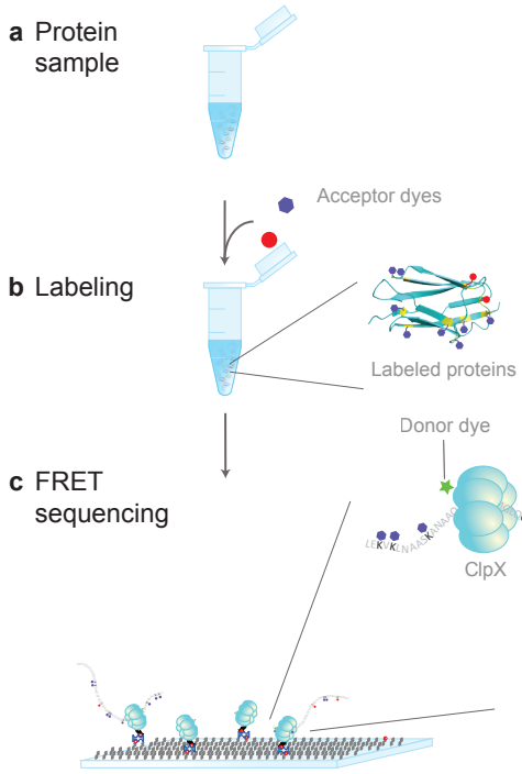
Figure 2.2: The schematic shows how single-molecule fingerprinting is carried out. (a) Proteins are obtained from diverse sources including single cells, tissues, and body fluids. (b) Extracted proteins are denatured, and cysteines and lysines are labeled with fluorescent dyes. (c) An engineered version of a protein translocase (e.g. bacterial ClpX) grabs individual substrate proteins, unfolds them, and translocates them through its nano-channel. Proteins are sequenced using FRET (Förster resonance energy transfer). The translocase is labeled with a donor dye. FRET occurs between the donor on the translocase and the two distinct acceptor dyes on a substrate when the substrate passes through the nanomachine. The FRET signals report the order of the labeled amino acids.
