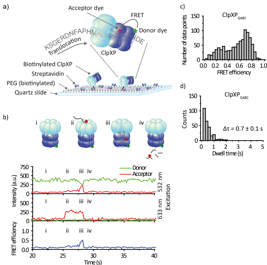
Figure 3.1: (a) Schematics of the single-molecule fingerprinting platform. Donor-labeled ClpXP is immobilized on a PEG-coated slide via biotin-streptavidin interactions. Acceptor-labeled substrates (K-38-C-ssrA with Cy5 at Cys, Supplemental table 3.1 ) are introduced to the microfluidic chamber. ClpX recognizes the substrate and translocate it into the ClpP chamber within which FRET occurs between donor and acceptor. (b) A typical fluorescence time trace. (i) The donor signal is from Cy3-labeled ClpXP (upper trace). (ii) The sudden appearance of acceptor signal during acceptor-direct excitation indicates binding of acceptor-labeled substrate to ClpXP (middle trace). (iii) A gradual increase in FRET represents the translocation of the substrate by ClpX into ClpP (bottom trace). (iv) Loss of signal represents the release of the substrate. (c) (Top) Dwell time of region (iii). (Bottom) FRET distribution of region (iii). Error represents SEM ( n = 239 ).
