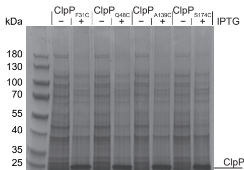
Figure 5.2: Full cell lysate on 4-20% SDS-PAGE gel after coomassie stain. Protein expression profiles were compared before and after induction with IPTG. For all four mutants a thick band appeared at the size of ClpP monomers.
