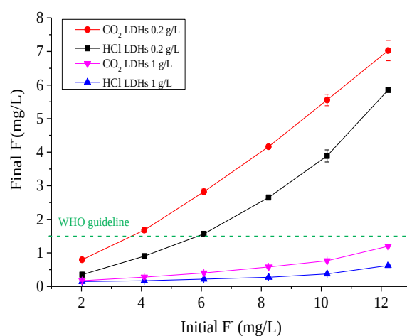
Figure S4. The effect of initial F^- concentrations on F^- removal efficiency. (Initial F^- =2,4,6,8,10,12 mg/L; pH=6; LDHs dose=0.2 or 1 g/L; T=22\pm 1^\circ\text{C} )
