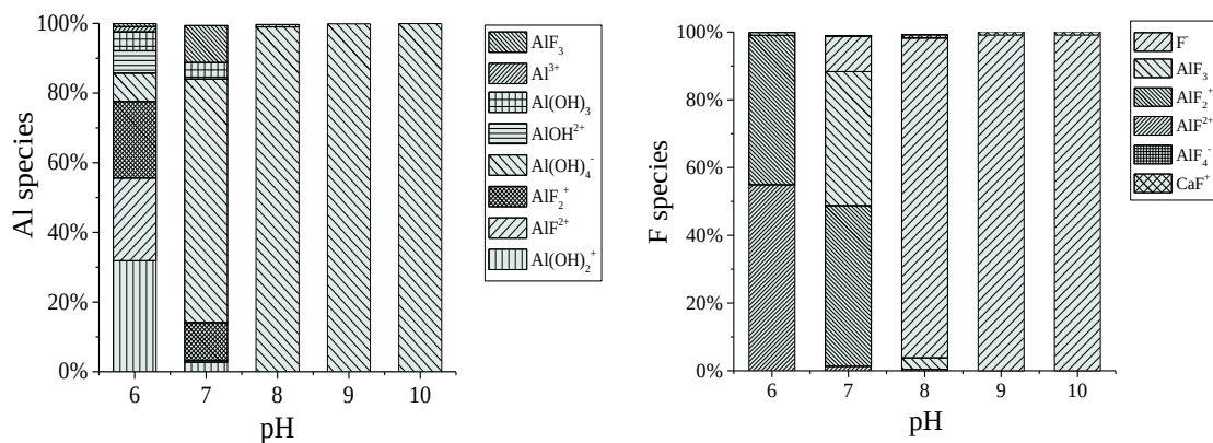
Figure 6. Distribution of Al and F species under different pH conditions simulated by PHREEQC. T=25^\circ\text{C} , \text{pH}=6\text{--}10 , \text{F}^-=10\text{ mg/L} , the molar ratio of \text{F}^-/\text{Al}^{3+}=0.2 .
