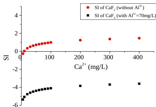
Figure S5. The SI values of \text{CaF}_2 with and without \text{Al}^{3+} . (pH=6, F^- =10mg/L, T=25^\circ\text{C} )
