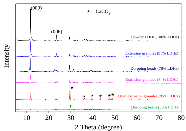
Figure S5. XRD patterns of the powder and granulated \text{Ca-Al-CO}_3 LDHs.
