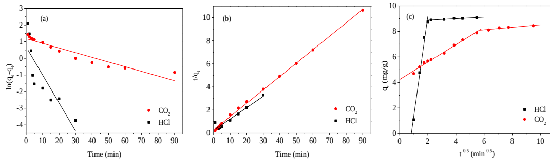
Figure S3. First-order kinetics model (a), Pseudo-second-order kinetics model (b) and Intraparticle diffusion model (c) fitting of the removal kinetics.
