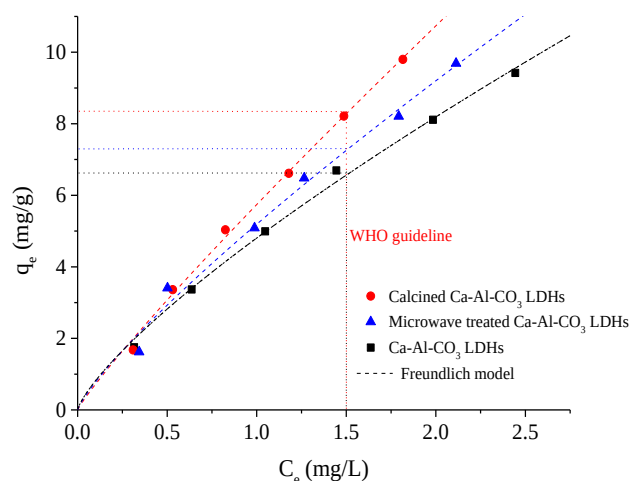
Fig. 2. \text{F}^- adsorption isotherm on \text{Ca-Al-CO}_3 LDH and its modified products, with loadings at WHO guideline of 1.5 mg/L value indicated as dashed lines.
