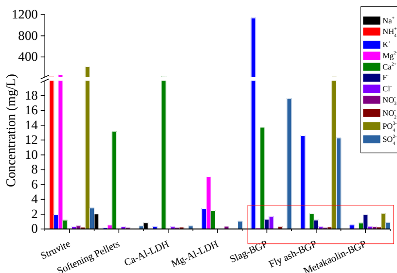
Figure 4. Ion leaching from low-cost mineral-based materials; Inset: \text{F}^- leaching from geopolymers. (BGP: based geopolymer)
