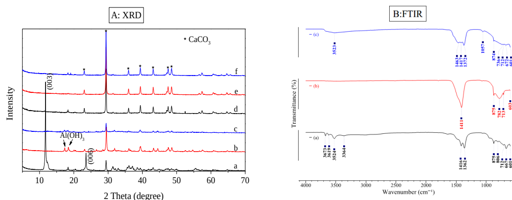
Fig. 1. XRD (A) and FTIR(B) spectra of Ca-Al- \text{CO}_3 LDHs (a), calcined Ca-Al- \text{CO}_3 LDHs (b) and microwave treated Ca-Al- \text{CO}_3 LDHs (c), Ca-Al- \text{CO}_3 LDHs after adsorption (d), calcined Ca-Al- \text{CO}_3 LDHs after adsorption (e) and microwave treated Ca-Al- \text{CO}_3 LDHs after adsorption (f); FTIR only measured before adsorption.
