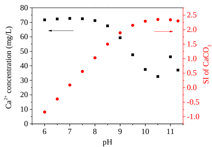
Figure S4. \text{Ca}^{2+} concentrations and the saturation-index (SI) of \text{CaCO}_3 at different pH.
