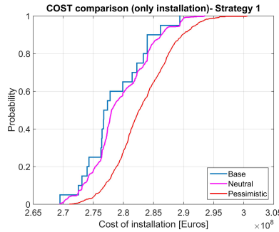
Figure 5.10: Cost of Strategy 1 for different risk aversions.
