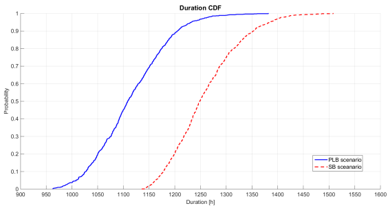
Figure 2.18: CDF curve of duration concerning PLB and SB scenarios including performance and failure uncertainties.
