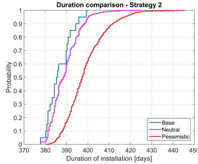
Figure 5.11: Duration of Strategy 2 for different risk aversions.
