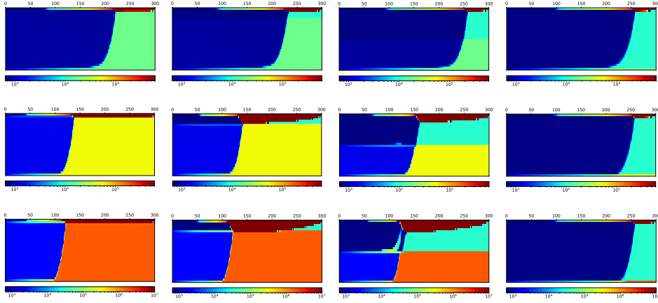
Figure 5.14: Total mobility ( mD/(Pa \cdot s) ) distributions in different layers at steady state. In all case, the higher-permeability layer is at the bottom. The plots illustrate different permeability ratios ( K_1/K_2 (first row), K_1/K_3 (second row), and K_1/K_4 (last row)) and different thickness ratios (1 m/29 m (first column), 5 m/25 m (second column), 15 m/15 m (third column), and 29 m/1 m (last column)), respectively.
