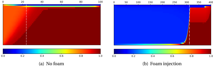
Figure 5.2: Water saturation profile ( f_{w} = 25\% ) at steady state. The white dashed line is the segregation point predicted by Eq. 5.1. In both cases, there are transition zones where water saturation is lower than that at the initial condition.
