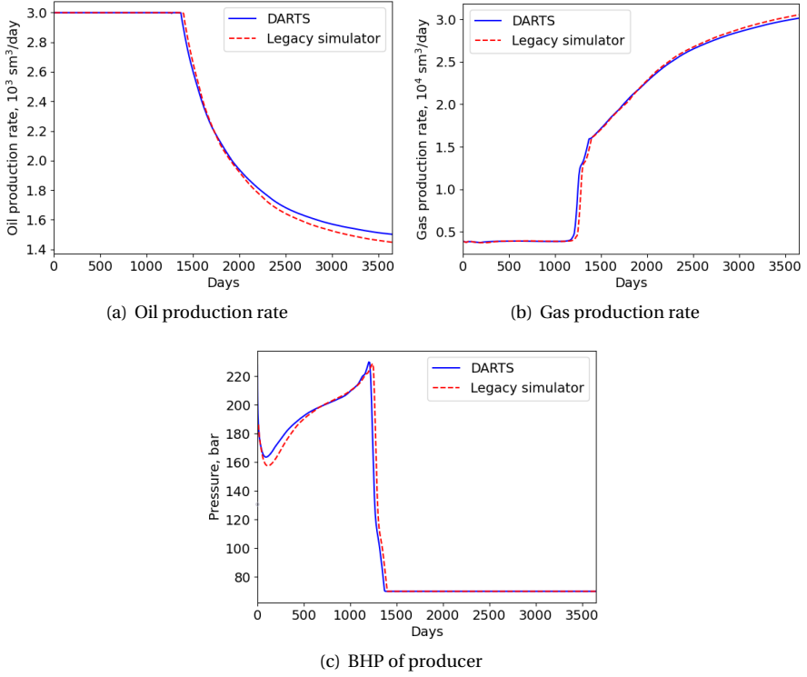
Figure 3.3: Comparison of well rates and BHP of producer with different simulators.
