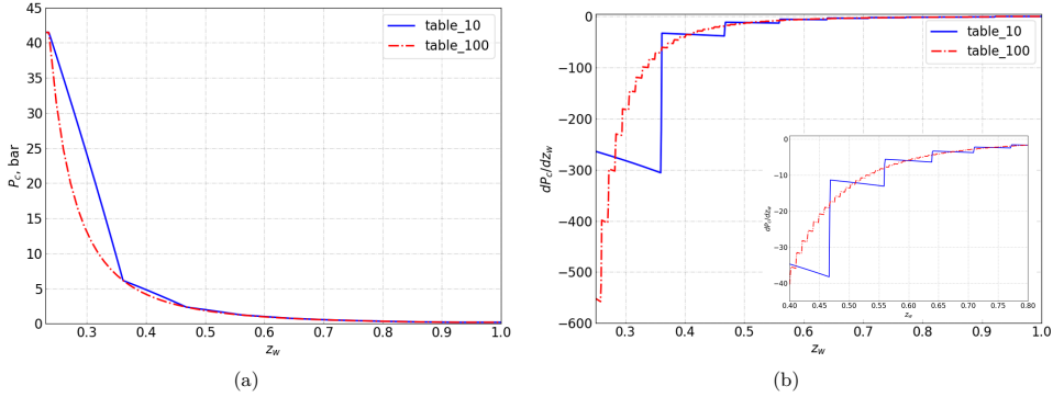
Figure 2.3: Capillary pressure (a) and its derivative (b) with respect to composition. Table 10 and Table 100 represent 10 and 100 supporting points in the given table, respectively. The subfigure zooms inset in (b) locally for a better visualization.
