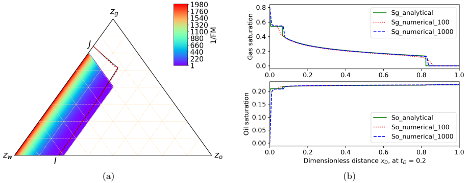
Figure 4.3: (a) Composition path ( f_{moil}=0.3 ) for Case 1 of Scenario 2 in ternary diagram. The injection condition (J) is outside but initial condition (I) is just inside the foam region. (b) Gas-saturation and oil-saturation profiles as functions of dimensionless position x_D at time t_D = 0.2 PVI. 100 and 1000 in numerical solutions represent different grid resolution.
