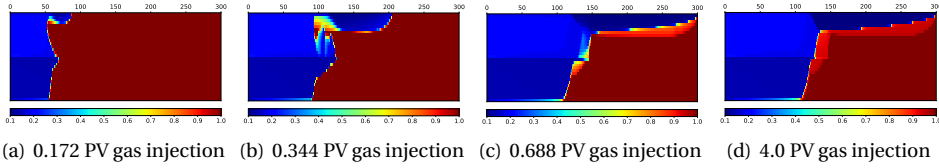
Figure 5.15: Variation of water saturation in transient flow in the case where the low-permeability layer is at the top. The permeability contrast is K_1/K_4 and the thickness is equal in the two layers.
