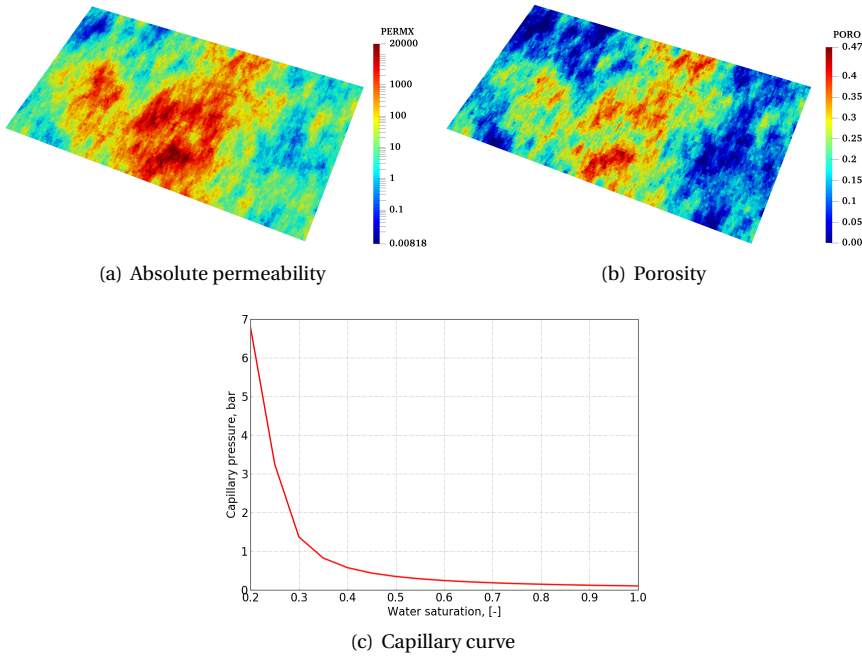
Figure 3.14: Porosity and permeability distribution, and capillary pressure curve of the 10th SPE comparative study.
