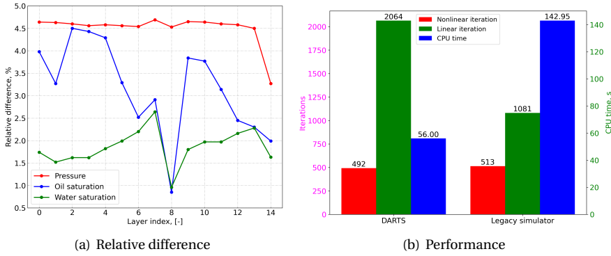
Figure 3.13: The accuracy and performance of two simulators for UNISIM model. (a) Relative difference of pressure and saturation between DARTS and the legacy simulator in each layer; (b) Comparison of the numerical performance between two simulators.
