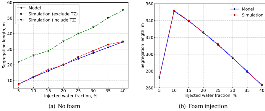
Figure 5.3: Comparison between analytical model and simulation results. (a) no foam; (b) foam. 'TZ' is an abbreviation of 'Transition Zone'.
