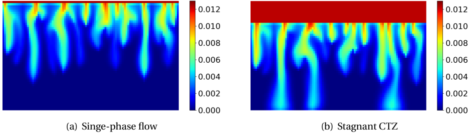
Figure 6.3: Fingers of dissolved \text{CO}_2 concentration (mol/mol) at 200 years for the simulations.
