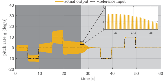
(c) Doublet response of pitch rate
