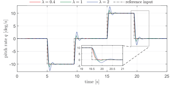
(d) Comparison of output signals with different values of \lambda_2
