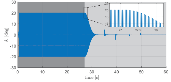
(b) Deflections of elevators
