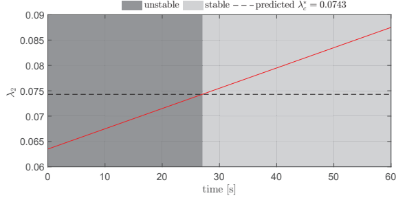
(a) The minimum eigenvalue \lambda_2 increases over time and intersects with the predicted bound for stability \lambda_c^* .
