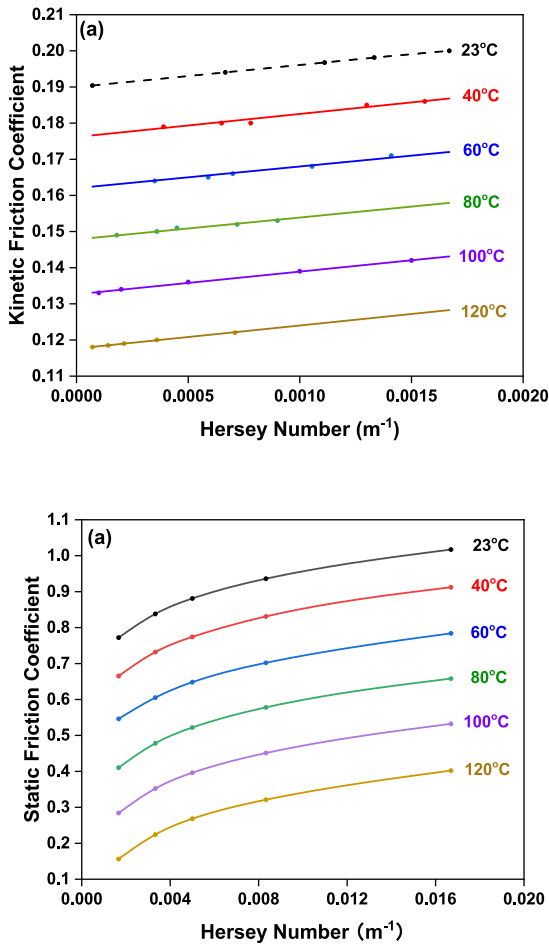
Fig. 20. Effect of test temperature on experimental friction coefficient and Hersey number: (a) Kinetic; (b) Static.
