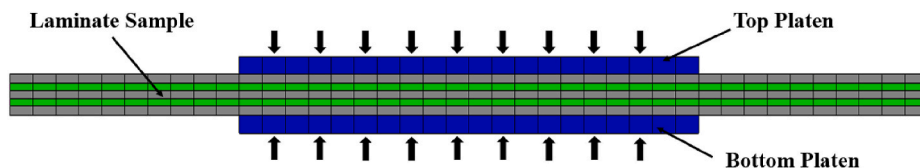
Fig. 21. Finite element model of the inter-ply friction test of the pre-stacked laminates.
