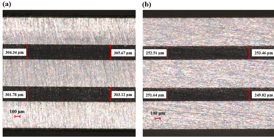
Fig. 19. Cross-section micrographs after friction test performed with a temperature of (a) 40 °C and (b) 120 °C – ( × 80).
