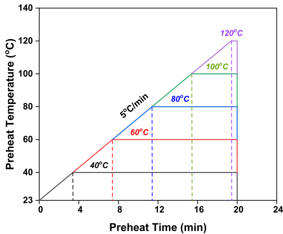
Fig. 3. Preheat temperature and time cycles for the pre-stacked GLARE materials.
