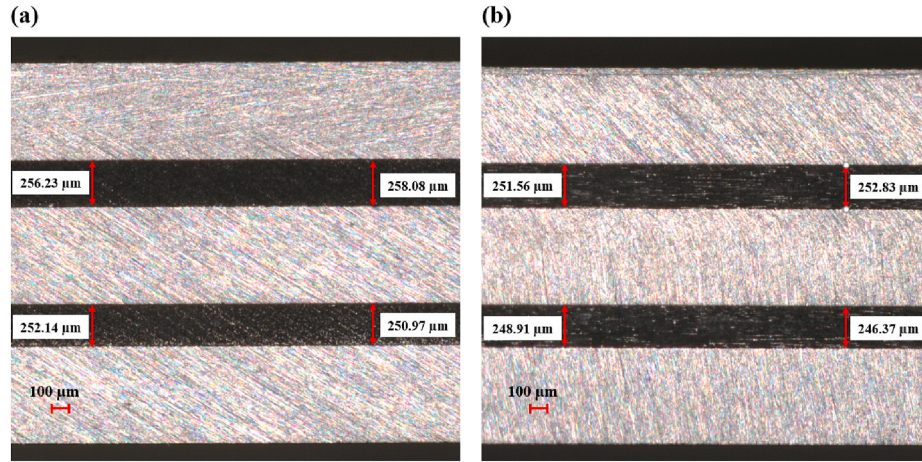
Fig. 16. Cross-section micrographs after friction test performed with a fibre orientation of (a) 45°/45° and (b) 90°/90° at the temperature of 80 °C – ( × 80).
