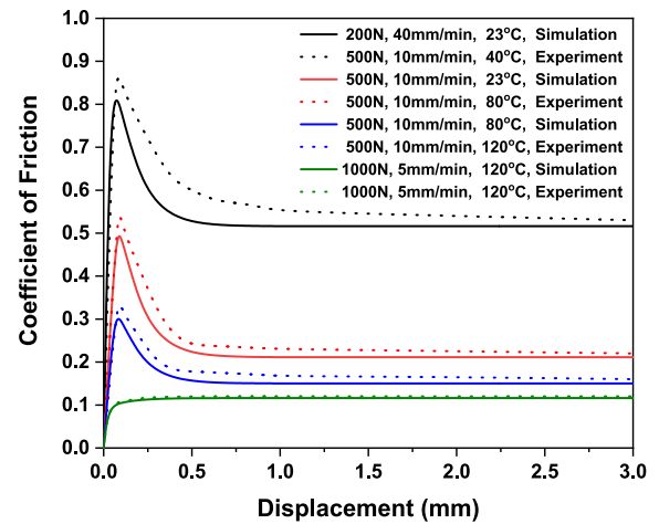
Fig. 22. Friction coefficient versus displacement curves from simulation model and experimental validation.
