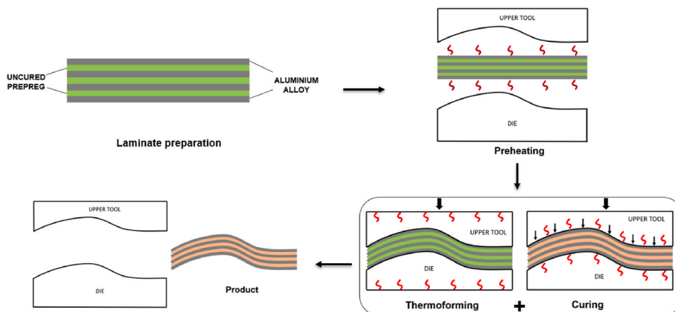
Fig. 1. Proposed hot-pressing process of fibre metal laminate manufacturing.
