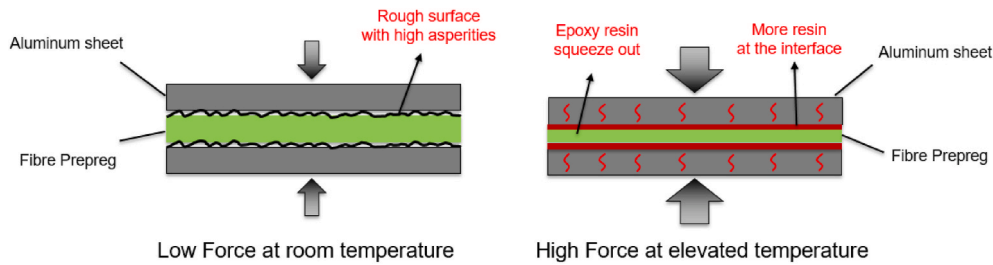
Fig. 10. Sketch for illustrating the effect of normal force and temperature after the friction test.
