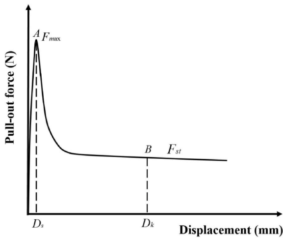
Fig. 8. Schematic curve of pull-out force and displacement relation for the friction test.
