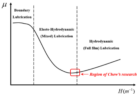
Fig. 2. Stribeck curve on friction coefficient versus Hersey number, indicating the range of Chow's research [25].
