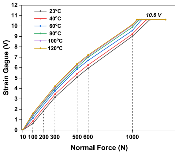
Fig. 6. Normal force and strain voltage curve under various temperatures for the clamping loadcell.
