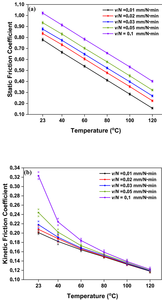
Fig. 17. Experimental friction coefficients under different temperatures: (a) Static; (b) Kinetic.
