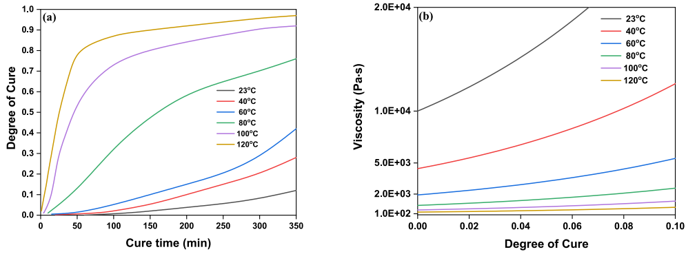
Fig. 7. Predicted cure development of FM-94 epoxy at different test temperatures:(a) Degree of cure; (b) Viscosity.
