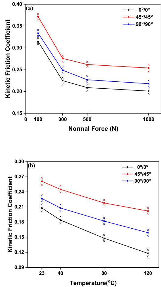
Fig. 14. Kinetic friction coefficients of normal force at room temperature of (a) 23 °C and temperature at (b) 500 N.
