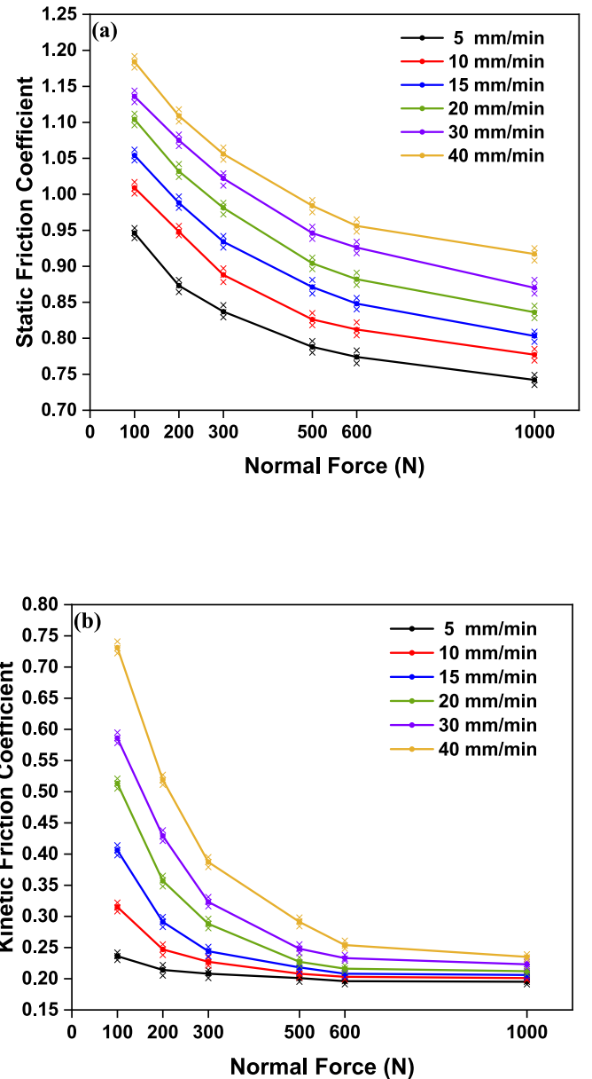
Fig. 9. Friction coefficients as a function of normal force and sliding velocity at room temperature: (a) Static; (b) Kinetic.
