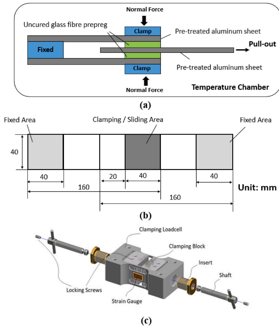
Fig. 4. (a) Schematic diagram and (b) Dimension for the inter-ply friction test, (c) Details of the clamping loadcell unit.
