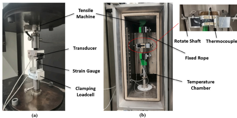
Fig. 5. Experimental setup and apparatus: (a) Calibration test of the normal force; (b) Inter-ply friction test.
