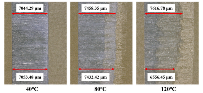
Fig. 18. Sliding surfaces after the friction test performed with different temperatures for 0°/0° interfaces– ( × 12).
