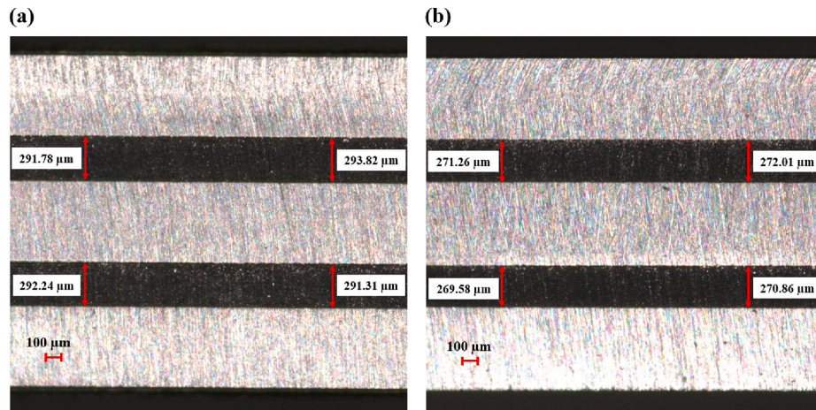
Fig. 12. Cross-section micrographs after friction test performed with a normal force of (a): 200 N and (b)1000 N at the temperature of 80 °C – ( \times 80 ).
