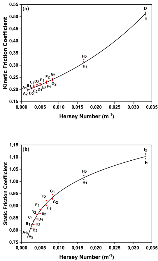
Fig. 13. Hersey number versus experimental friction coefficient at room temperature: (a) Kinetic; (b) Static.
