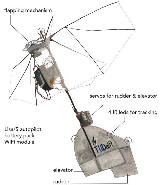
Figure 2: The DelFly II flapping-wing MAV used in this study. Commissioned illustration by Sarah Gluschitz, licensed under CC BY-ND.
