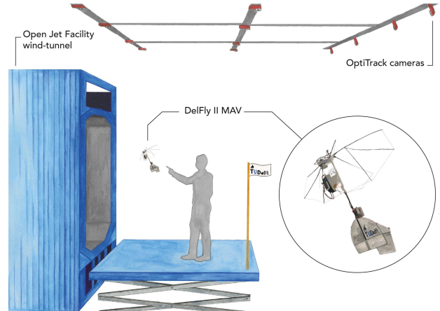
Figure 1: The DelFly II preforming a precision flight in the wind-tunnel. The achieved precision of \pm 2.5 cm will allow unprecedented in-flight aerodynamic measurements in future. Commissioned illustration by Sarah Glusnitz, licensed under CC BY-ND.
