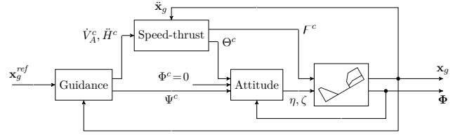
Figure 5: The hierarchic control scheme for the DelFly control approach.
