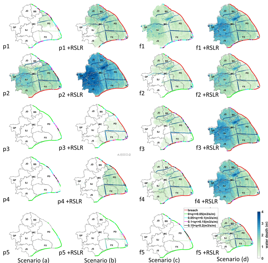
Fig. 10 Spatial extent of inundation depth due to overtopping and breaching (with breach width of 1000 m) under four scenarios, and spatial distribution of breach locations (red line) and overtopping locations (green line shows an overtopping discharge rate ( q ) \leq 0.05 m 3 /s/m; cyan line shows 0.05 < q \leq 0.1 m 3 /s/m; magenta line shows 0.1 < q \leq 0.15 m 3 /s/m; black line shows 0.15 < q < 0.2 m 3 /s/m) for 10 hypothetical typhoons
