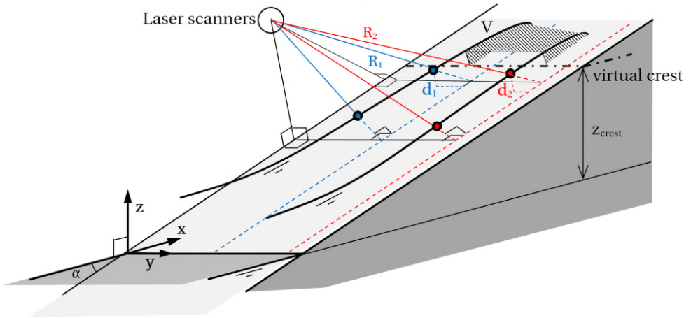
Figure 6.3: System set-up as used for the conversion of measured distances ( R_1 [m] and R_2 [m], blue and red lines) in polar coordinates to cartesian x , y , z -coordinates [m] according to the coordinate system as shown. Dike slope \alpha [°], laser scan lines (blue and red dashed lines), scanned points on water surface (blue and red dots), virtual crest level z_{\text{crest}} [m], run-up depths d_1 [m] and d_2 [m], and virtual overtopping volume V [m 3 ] indicated.
