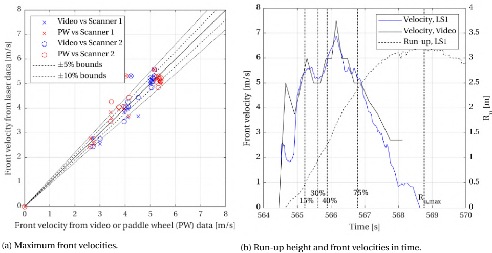
Figure 5.6: Left: Front velocities from laser data compared to video and paddle wheel (PW) data. Right: Run-up and front velocity time signals of one of the laser scanners and front velocity time signal from video analysis for a wave with a filling level of 5 m of test 1. Dotted lines indicate percentages of the maximum run-up level.
