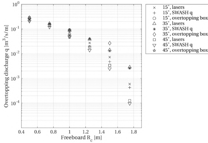
Figure 6.15: Overtopping discharge for several virtual crest levels as determined from the virtual laser scanner data for three SWASH simulations. Tests 10 to 12, with angles of incidence of 15° (crosses), 35° (triangles) and 45° (squares). SWASH discharge parameter q (pluses, asterisks, down-pointing triangles) and virtual overtopping box data (circles, diamonds, pentagrams) plotted as well. Simulations with a 1:4 slope, a JONSWAP spectrum with H_s = 1 m and T_p = 4 s.
