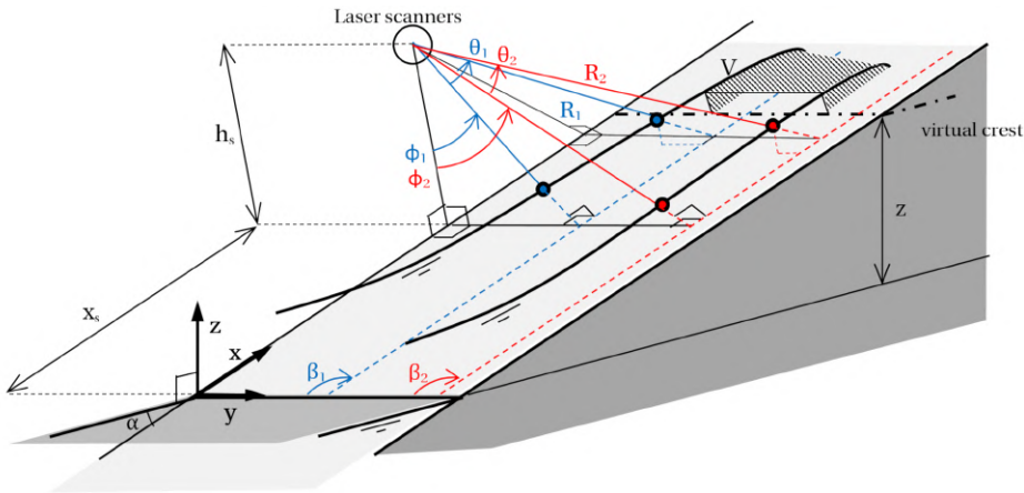
Figure 5.2: Schematised set-up with two laser scanners. Set-up based on Hofland et al. (2015) , but with two laser scanners. Scan lines (blue and red dashed lines), scanned points on water surface (blue and red dots) indicated. R [m] is the scanned distance, \theta [°] the scan angle, \phi [°] the slant angle, \beta [°] a correction in case the scanned line does not run straight along the slope. h_s [m] the laser scanner heights, x_s [m] the x -coordinate of the laser scanners, \alpha [°] the slope angle. V [m 3 /m] is a virtual overtopping volume.
