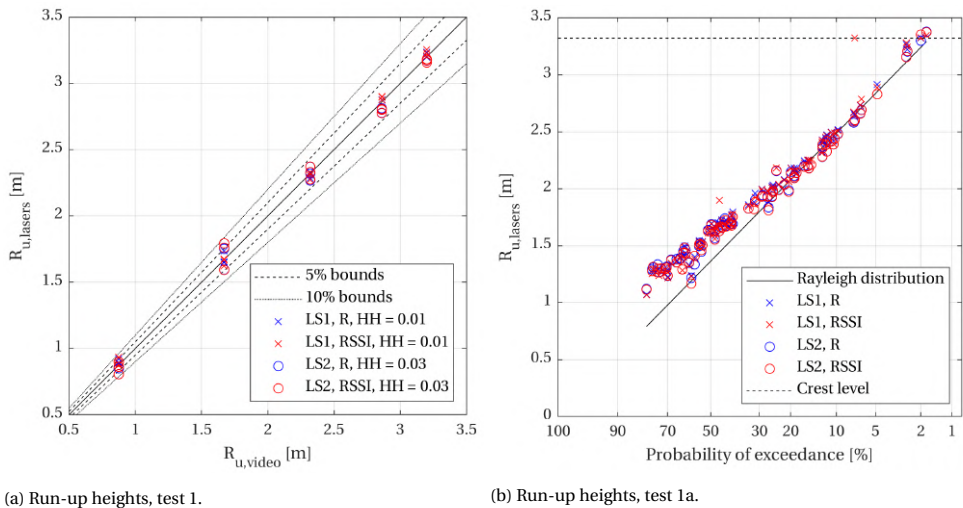
Figure 5.4: Left: Run-up data for test 1 from both laser scanners and based on both distance and RSSI versus run-up heights from video data. Right: Run-up data for test 1a from both laser scanners and based on both distance and RSSI, as well as Rayleigh distribution from wave run-up simulator filling level formula. The x -axis on Rayleigh scale, the dike crest level is indicated with the horizontal dashed line.
