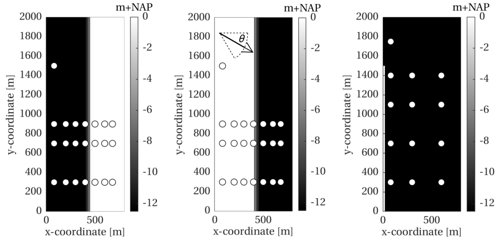
Figure 4.3: Bathymetries of the academic refraction (first two panels) and diffraction (third panel) models. Model (2D spectra) output locations shown with circles, range of angles of incidence \theta shown in middle panel.
