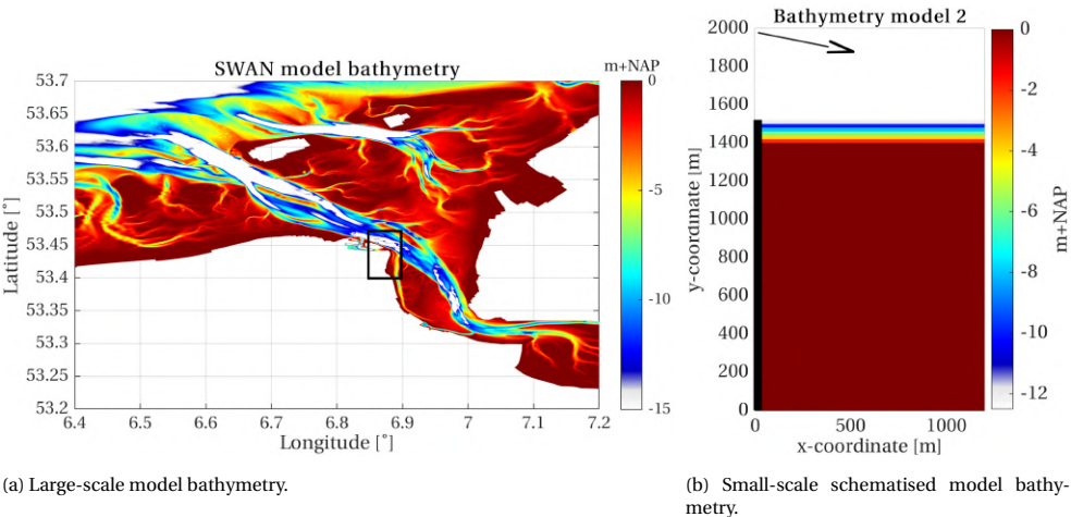
Figure 3.4: Left: SWAN model bathymetry as used for the quantification of propagation effects and the comparison of the two SWAN versions, with the area around the Eemshaven indicated by the rectangle. Right: Bathymetry of the schematised model of the area around the Eemshaven, including the shallow area in front of the dike and a 1:10 slope. The western boundary ( y = 0 m until y = 1500 m) is closed off, representing the dike (thick black line). Mean wave direction indicated with the arrow.
