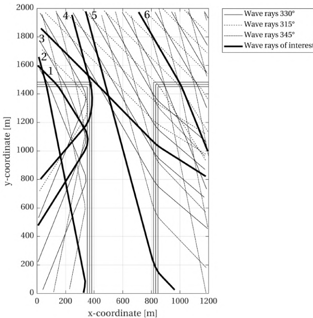
Figure 4.15: REFRAC wave rays for the detailed model. The mean wave direction and 30° directional spreading are represented by wave rays from 330°N, 315°N and 345°N. Several wave propagation effects occur: Relatively unaltered propagation onto shallow flats (2 and 6), relatively unaltered propagation into channel (5), wave defocusing on channel slopes (4), refraction out of channel (3), and wave reflection off the channel slope or wave trapping (1).
