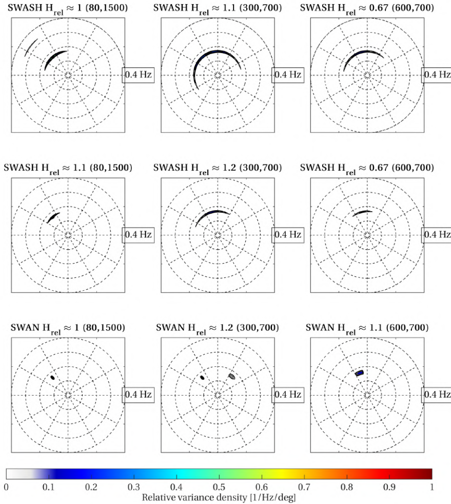
Figure 4.6: 2D spectra at three locations for regular waves travelling from shallower to deeper water with \theta = 48^\circ (318°N). Top row: SWASH with non-linear waves ( H_s = 1 m). Middle row: SWASH with linear waves ( H_s = 0.1 m). Bottom row: SWAN with non-linear waves ( H_s = 1 m). Variance density of each model normalised and colour-scaled with the maximum variance density at the offshore (80,1500) location.
