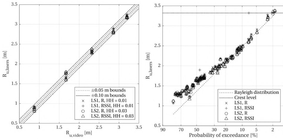
(a) Run-up heights, test with 21 perpendicularly incident waves. (b) Run-up heights, test with 100 randomly generated perpendicularly incident waves.
