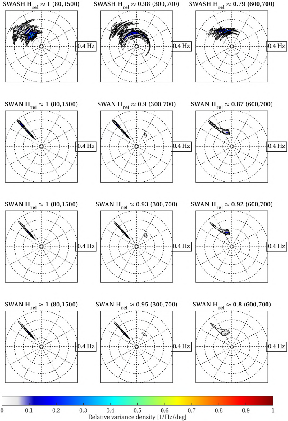
Figure 4.8: 2D spectra at three locations for irregular, narrow spread waves travelling from shallower to deeper water with \theta = 48^\circ (318°N). Top row: SWASH. Second row: SWAN with the recommended settings for the numerics (see sub-section 4.5.1 and appendix D) and the default settings for the physics (see appendix D). Third row: SWAN with the same settings, but with \alpha = 0.05 instead of \alpha = 0.8 . Bottom row: SWAN with the same settings, \alpha = 0.05 , 20 m grid cells and the diffraction approximation enabled. Variance density of each model normalised and colour-scaled with the maximum variance density at the offshore (80,1500) location.
