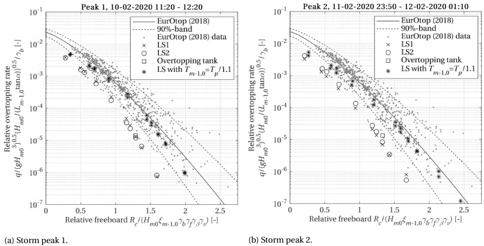
Figure 7.13: Relative overtopping rate for several virtual crest levels, based on both laser scanners (crosses, circles) and the overtopping tank (squares), for both storm peaks. The laser scanner data have also been plotted using the relation T_{m-1,0} = T_p/1.1 (asterisks). Results compared to EurOtop (2018) equations (solid and dashed lines) and data (dots). Figure based on EurOtop (2018). R_c [m] is the crest freeboard, \xi_{m-1,0} [-] is the breaker parameter, the different \gamma parameters [-] are influence factors, see EurOtop (2018).
