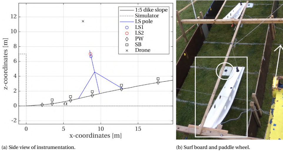
Figure 6.2: Left: Side view of system set-up and instrumentation. x -coordinates horizontal, z -coordinates vertical, y -coordinates perpendicular to the figure. \alpha [°] is the slope angle. LS pole is the laser scanner pole, LS1 the lower laser scanner, LS2 the upper laser scanner. PW are the 6 paddle wheels; SB the five surf boards. Right: Example of surf board (white rectangle) and paddle wheel (white circle). Up-slope direction indicated by the arrow.
