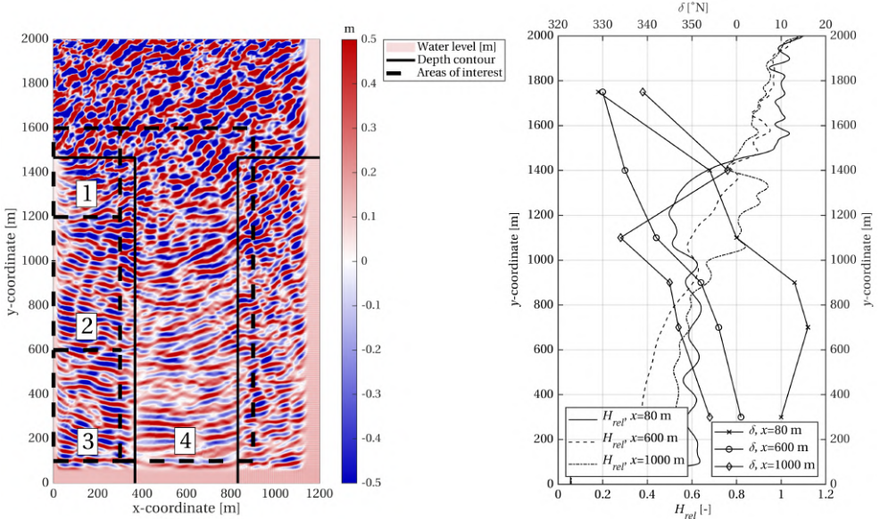
Figure 4.16: Left: SWASH snapshot of steady-state surface elevation and four areas of interest. Directional narrowing and reduction of wave energy, due to wave sheltering, diffraction, depth-induced breaking and refraction from the deep channel to the shallow flat (1). Directional narrowing and slight increase of wave energy, due to wave sheltering, wave (de)focusing and wave reflection or trapping (2). Reduction in wave sheltering, diffraction and wave (de)focusing (3). Directional narrowing and reduction in wave energy, due to wave (de)focusing (4). Right: Relative wave height H_{rel} [-] and mean wave direction \delta [°N] along three y-transects at x = 80 m, x = 600 m and x = 1000 m.
