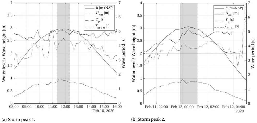
Figure 7.6: Overview of measurements near the toe of the dike around both storm peaks. The shaded regions indicate the considered storm peaks. h [m+NAP] is the water level, H_{m0} the significant wave height [m], T_p the peak wave period [s], T_{m-1,0} [s] the wave period based on the moments of the spectrum.
