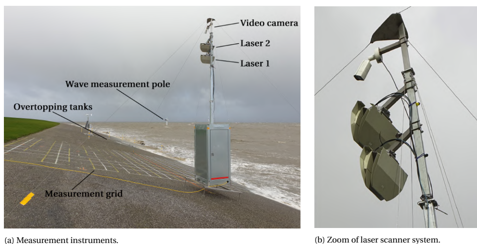
Figure 7.2: Left: New laser scanner system on the dike in the Eems-Dollard estuary, next to the overtopping tanks, during storm Ciara. The Rijkswaterstaat (wave) measurement pole can be seen in the distance. Rijkswaterstaat is the Directorate-General for Public Works and Water Management in the Netherlands. Right: From the bottom to the top, Laser scanner 1, laser scanner 2, video camera.
