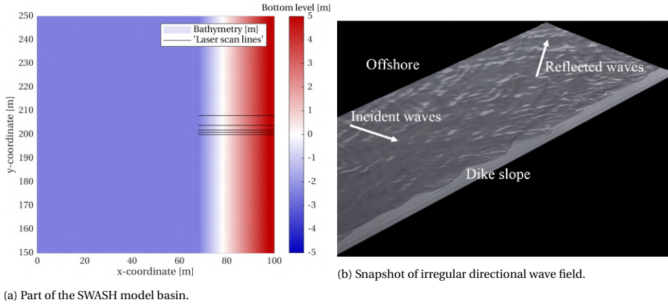
Figure 6.11: Left: Part of the 2.5 m deep SWASH basin with a 1:4 dike slope. The virtual laser scan lines are indicated as well. Right: Snapshot of irregular directional wave field, with an angle of incidence of 45^\circ and a directional spreading of 25^\circ . Also refer to https://youtu.be/cy-VWmV7aUA .
