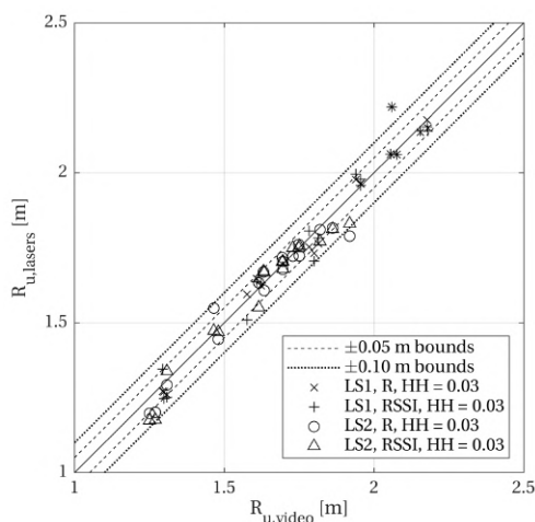
Figure 6.9: Run-up heights from both laser scanners, based on both measured distance ( R ) and laser reflectance ( RSSI ) versus run-up heights from videos, for a test with obliquely incident waves. Distance between laser lines 1.3 m.
