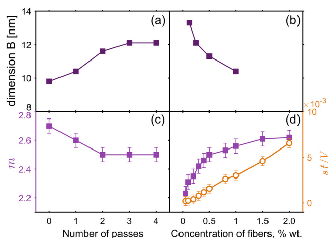
Fig. 2. Effect of HPH treatment and fiber concentration on structural parameters of citrus fiber dispersions as obtained by SAXS. (a,b) Kratky plot dimension B as a function of (a) number of HPH passes on a 1%wt. citrus fiber dispersion and (b) the concentration of citrus fibers. (c,d) Fitted structure power-law exponent m associated to mass fractal behavior as a function of (c) number of HPH passes on a 1%wt. citrus fiber dispersion and (d) the concentration of citrus fibers. In plot d also fitted volume fraction ( sf/V ) is presented. (right axis).
