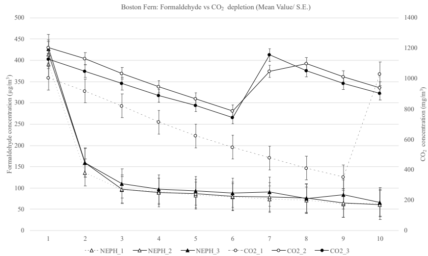
FIG. 4.9 Depletion of formaldehyde (NEPH_1, NEPH_2, and NEPH_3) vs depletion of CO 2 (CO2_1, CO2_2, and CO2_3): for the three Boston Ferns. Data means \pm SE, n=3.
