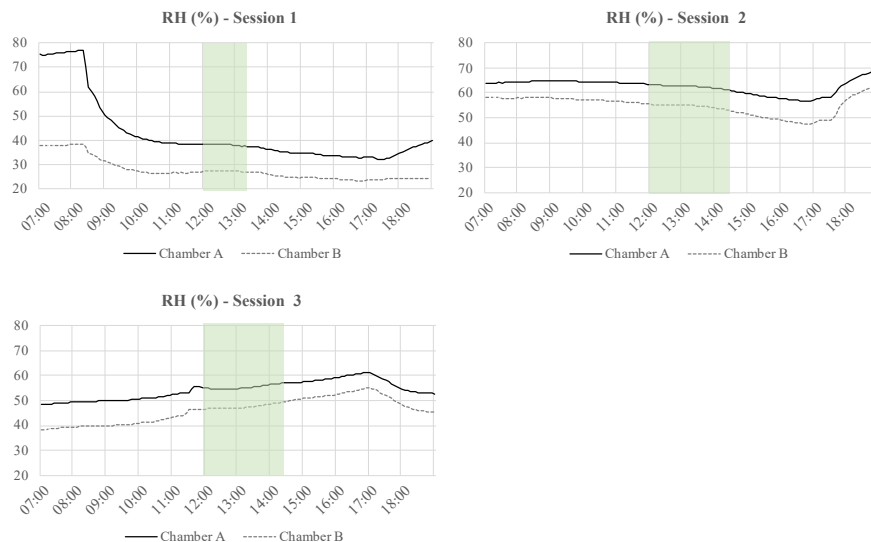
FIG. 5.6 Relative Humidity (RH) (%) at the days of the three sessions from 7.00 to 19.00 every 5 minutes. The highlighted section is the period when the participants executed the experiment and filled the questionnaires.
