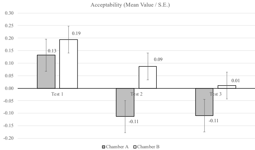
FIG. 5.9 Acceptability assessment for the two chambers during the three sessions: Mean values and Standard Errors (S.E.) (Session 1: n=44; Session 2: n=57; Session 3: n=46).
