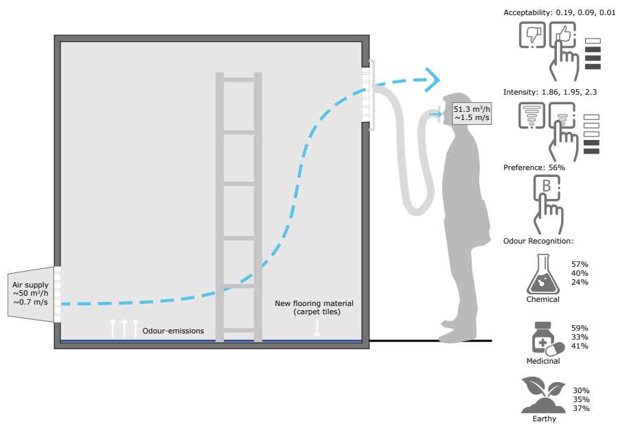
FIG. 6.5 Sensory assessment of chamber B.
