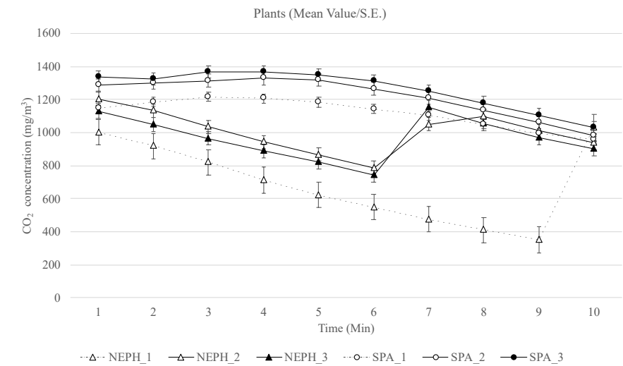
FIG. 4.8 Depletion of CO 2 (mg/m 3 ): for the three Boston Fern (NEPH_1, NEPH_2, and NEPH_3) and for the three Peace Lilies (SPA_1, SPA_2, and SPA_3). Data means ± SE, n=3.
