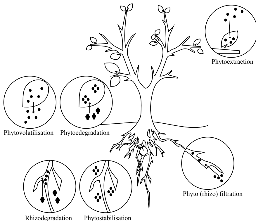
FIG. 2.1 Phytoremediation techniques.
