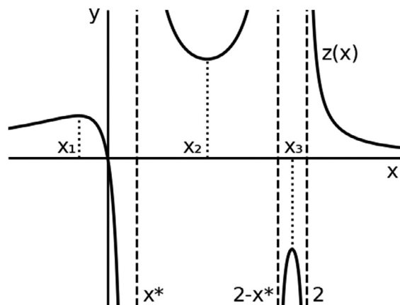
Fig. 16. The function z(x) in the proof of Theorem 3.2.
