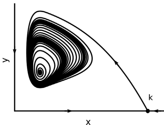
Fig. 19. System (4.1); \phi = 1 , k = 4 , \delta = .86 .
