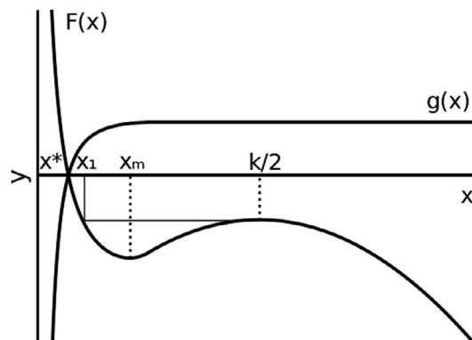
Fig. 21. F(x) and g(x) in system (4.9).
