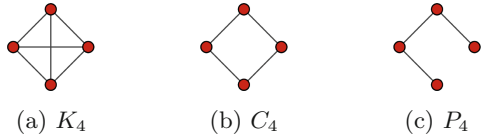
Fig. 1. Three types of graphs with 4 nodes.
