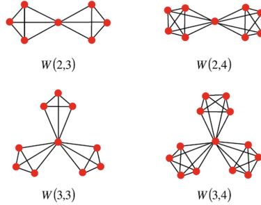
Fig. 5. Illustration of some windmill graphs W(\eta, k)
