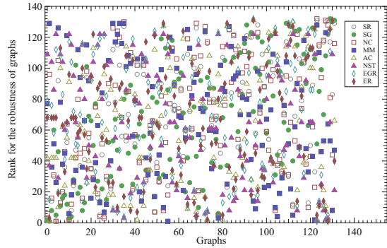
Fig. 3. Rank for the robustness of 132 graphs with 7 nodes and 10 links.
