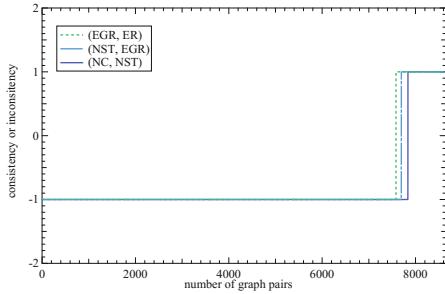
Fig. 4. The consistency (marked as 1) and inconsistency (marked as -1 ) results for metrics pairs of ( NC , NST ), ( EGR , NST ) and ( EGR , ER ).
