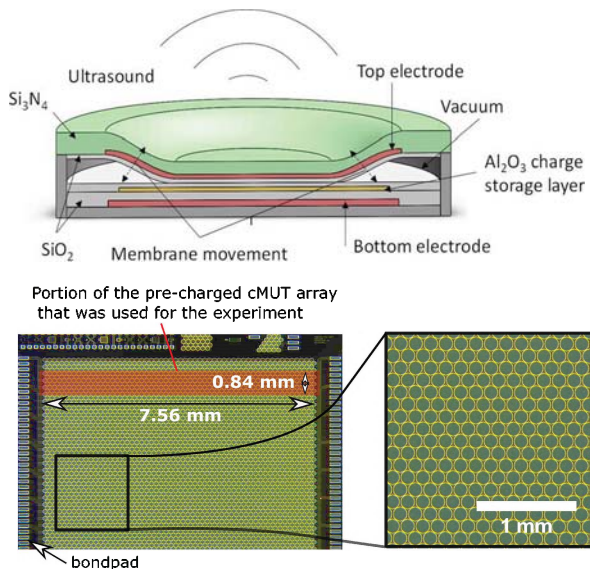
Figure 1 Cross sectional diagram of a pre-charged collapse-mode CMUT and an optical microscope photo of the ultrasound transducer.
