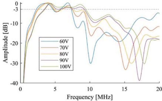
Figure 3 Impulse response showing the bandwidth of the CMUT for different external bias voltage.
