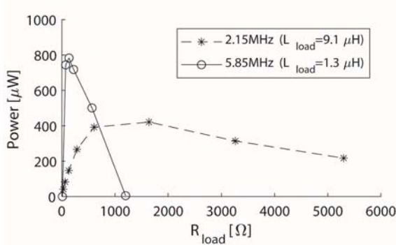
Figure 6 Ultrasound power transfer against load resistance.
