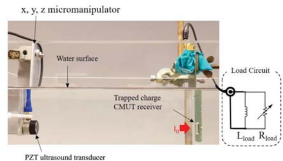
Figure 5 Experimental setup for testing maximum power transfer.
