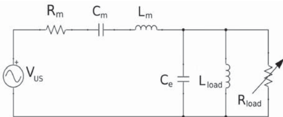
Figure 4 Equivalent circuit model of the CMUT during ultrasound power transfer.
