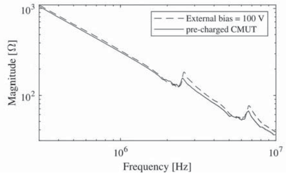
Figure 2 Impedance Spectrum of the pre-charged CMUT compared
