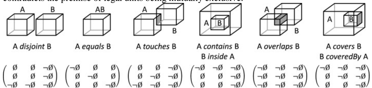
Figure 8: Eight predicates defining the possible topological relationships between two solids in 3D (Daum & Borrmann, 2014)
