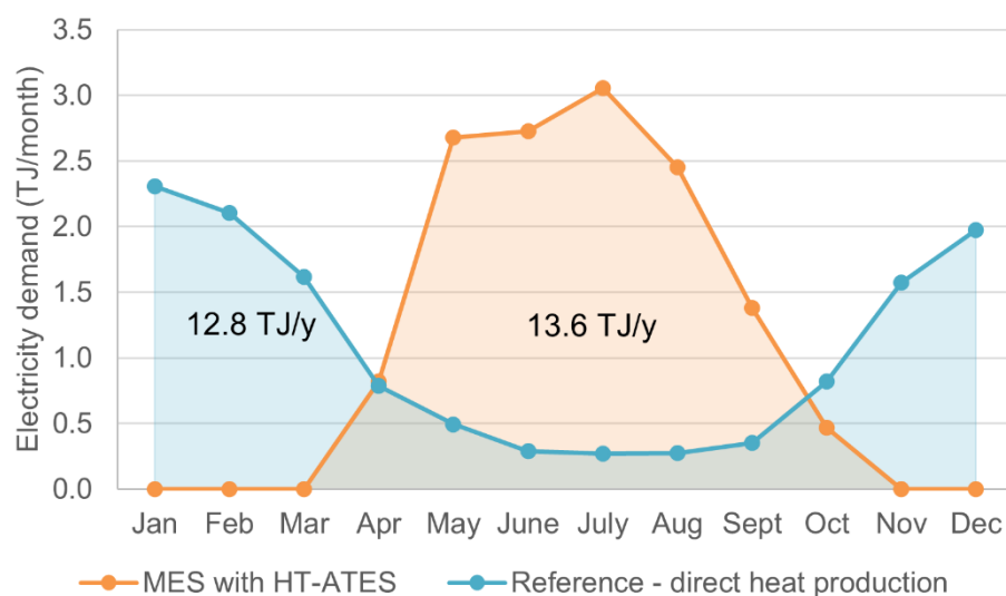
Figure 12. Comparison of the monthly electricity demand of a reference scenario with direct heat production by a heat pump with 8 °C evaporator temperature and the 50|30|1.5 scenario with HT-ATES. The areas under the graph show the total electricity demand over the year, in this case the year 2019.
