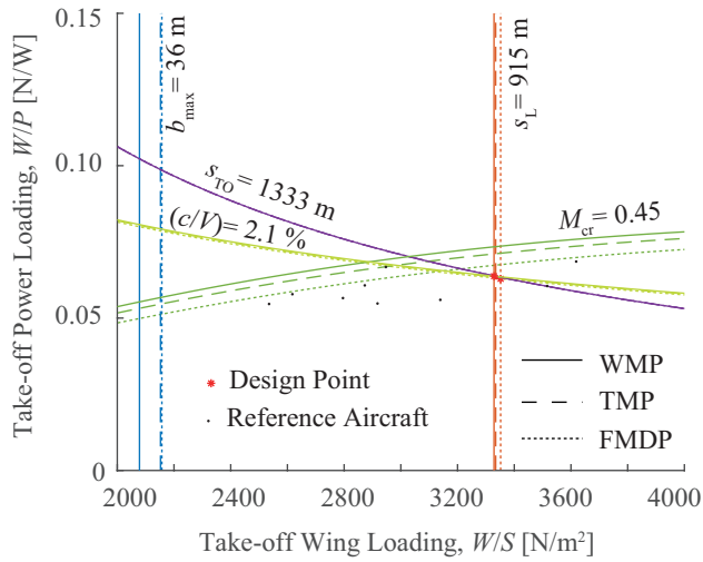
Fig. 4 Wing-loading versus power-loading diagram for each of the three synthesized aircraft configurations.
