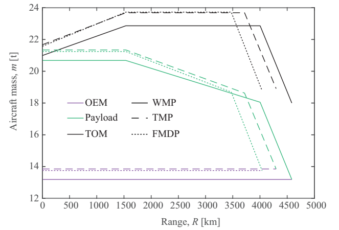
Fig. 10 Comparison of the payload-range diagrams for the three different aircraft. TOM is take-off mass, OEM is operational empty mass.
