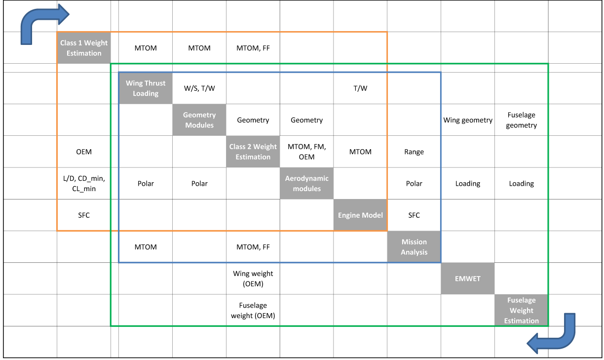
Fig. 2 Design Structure Matrix of the Initiator process flow. On the diagonal the main modules are shown, while on the off-diagonal cells the input/output of modules is displayed. The colored boxes indicate the three nested loops that the initiator executes iteratively.
