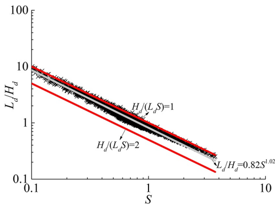
Figure 12. Cyclic step aspect ratio from about 3,000 numerical runs of the plunge pool model (The range of simulation parameters is C_f \in [0.01, 0.05] , u_i \in [0.1 \text{ m/s}, 0.9 \text{ m/s}] , S_f \in [0.1, 0.9] , q_w \in [0.001 \text{ m}^2/\text{s}, 5 \text{ m}^2/\text{s}] , and n \in [1.5, 4] ). The expected range of H_d/(L_d S) from 1 to 2 for natural step pools is shown by the two red lines. The gray line is a curve fitted to the numerical data with a power function.
