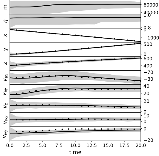
Fig. 4: Convergence of particle filter (noise model \Sigma_{n3} )
