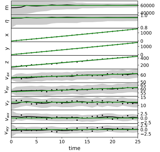
Fig. 2: Particle filter convergence (noise model \Sigma_{n2} )
