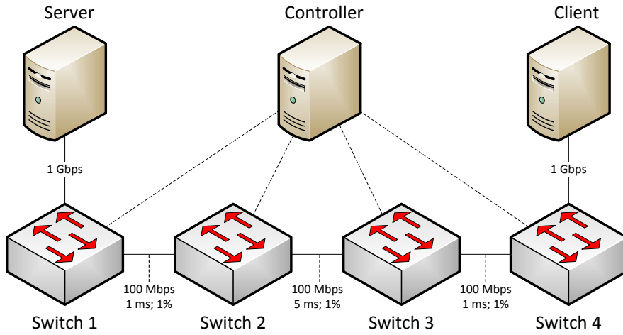
Figure 3.3: Experiment testbed topology. The measured traffic flows from Server to Client.
