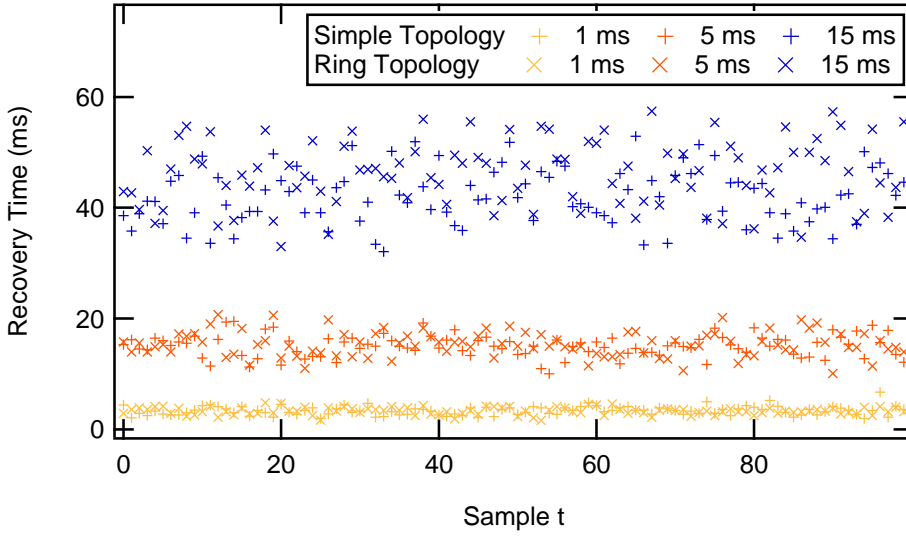
Figure 4.5: Recovery times for selected BFD transmit intervals and topologies.
