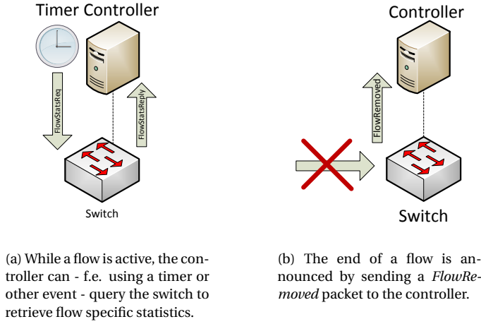
Figure 3.2: While a flow is active, the controller and switch can exchange messages concerning the flow's state.
