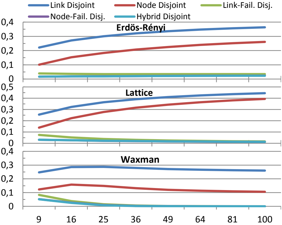
Figure 5.11: Average length of crankback paths relative to length of their respective shortest path.
