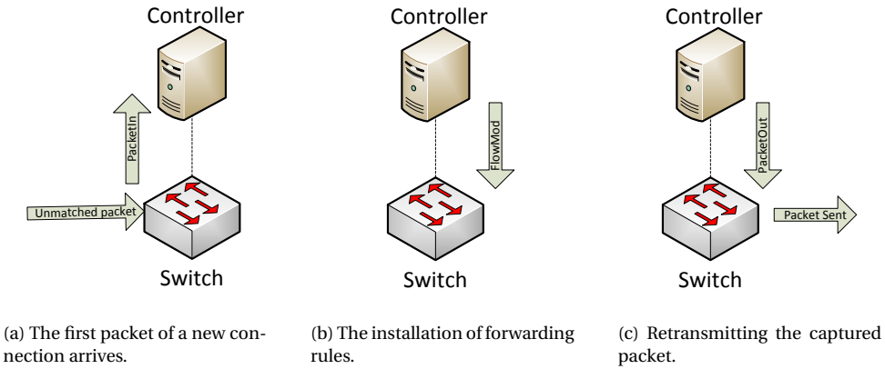
Figure 3.1: The three-step installation procedure of a new flow.
