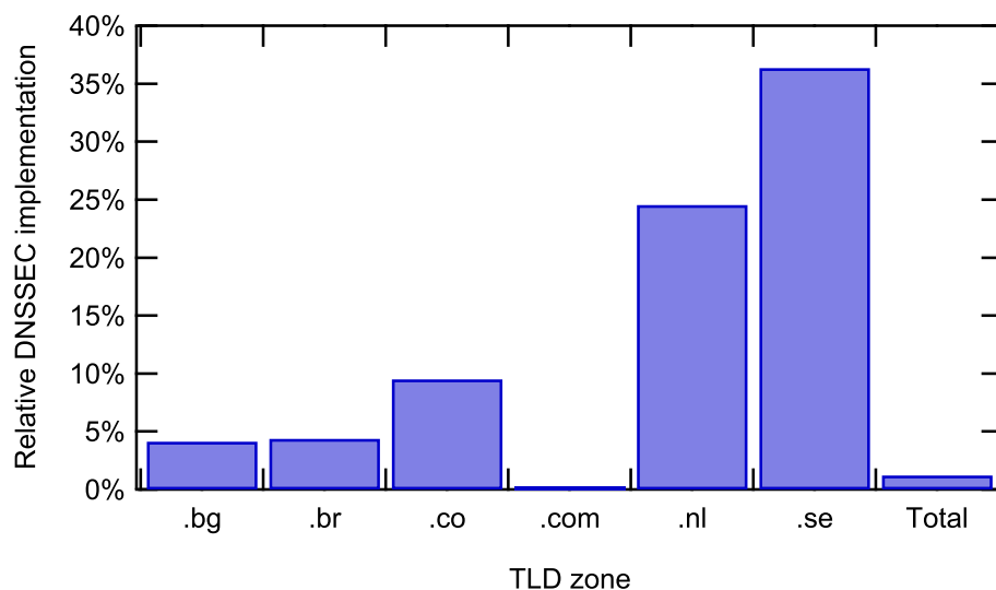
Figure 8.9: Relative implementation of DNSSEC found through bottom-up evaluation per country-code TLD.
