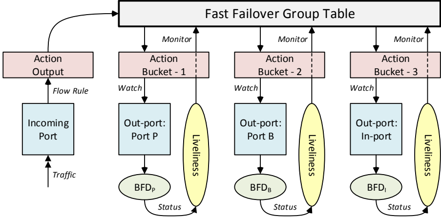
Figure 4.1: OpenFlow Fast Failover Group Table.
