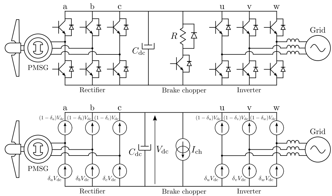
Figure 6. Back-to-back converter topology with a brake chopper ( top ) and an averaged model ( bottom ).
