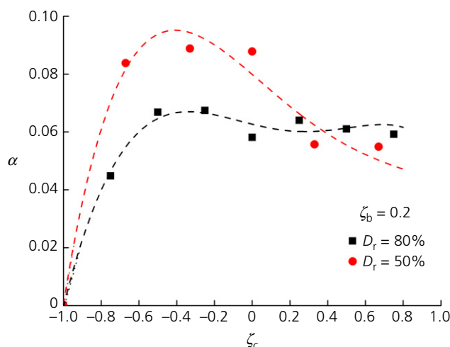
Figure 7. Load directional characteristic effects from cyclic tests
