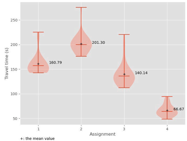
Fig. 17. Violin plot of the time spent by the participants during four assignments.
