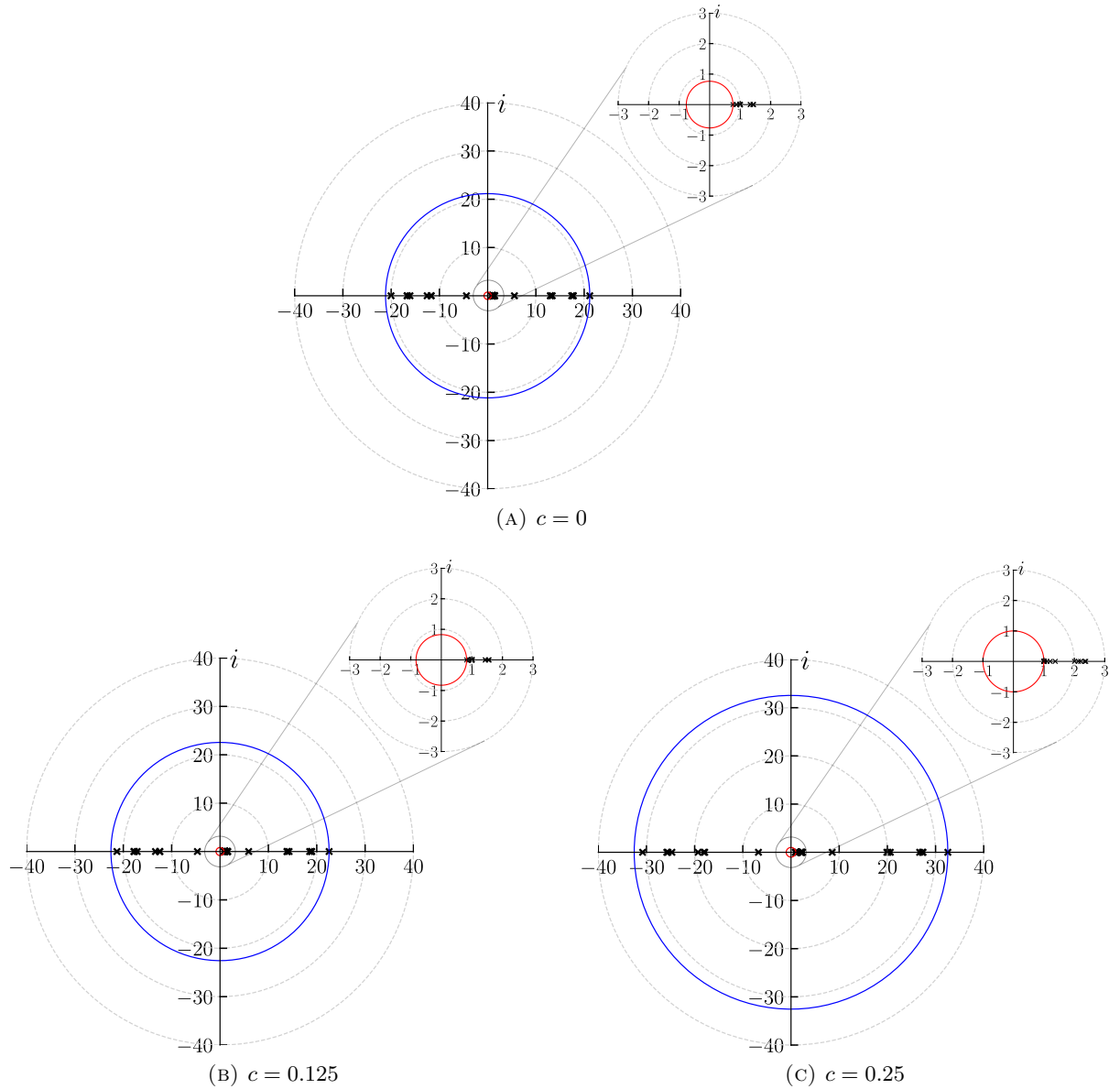
FIGURE 2.7: Results of the eigen-spectrum of \mathbb{F} for N = 1 , K = 2 . The radii of the blue and red circles are the moduli of the eigenvalues of the maximum and minimum modulus respectively.
