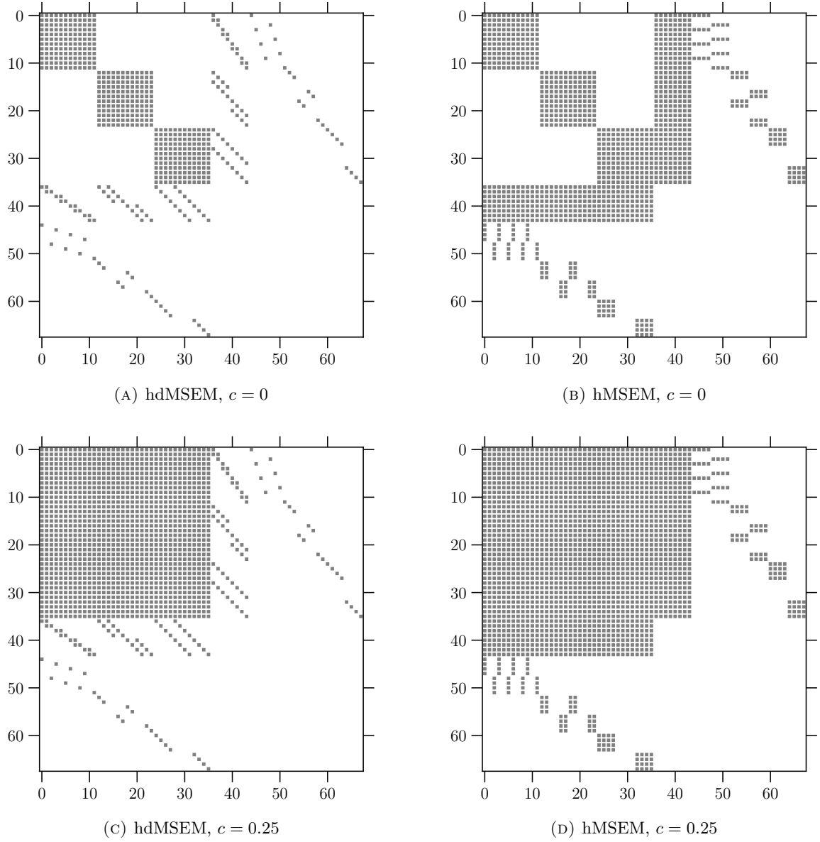
FIGURE 5.1: Sparsity plots of the left-hand-side matrices of (5.29) and (5.30) in the element \Omega_0 of the crazy mesh, see Complement 2.14, for K = 1 , N = 2 and c = 0, 0.25 .
