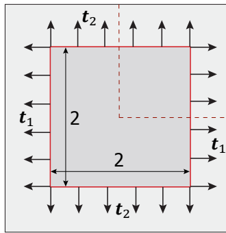
Figure 5.5: Schematic of the biaxial tension example with tractions t_1 and t_2 prescribed to edges of a square design domain as shown. The design domain is immersed into a larger background domain that is discretized by constant strain triangles. Due to symmetry, only a quarter of this domain is considered.
