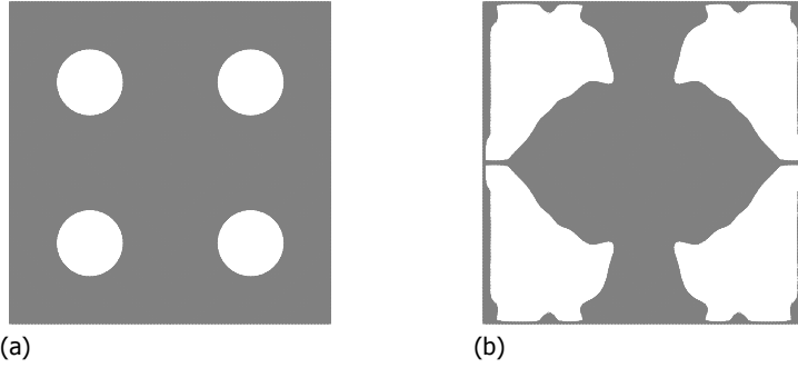
Figure 5.17: (a) Initial design with four holes in the whole domain where the ratio J_2/J_1 = -1 ; (b) The corresponding optimized design with J_2/J_1 = -14.85 .
