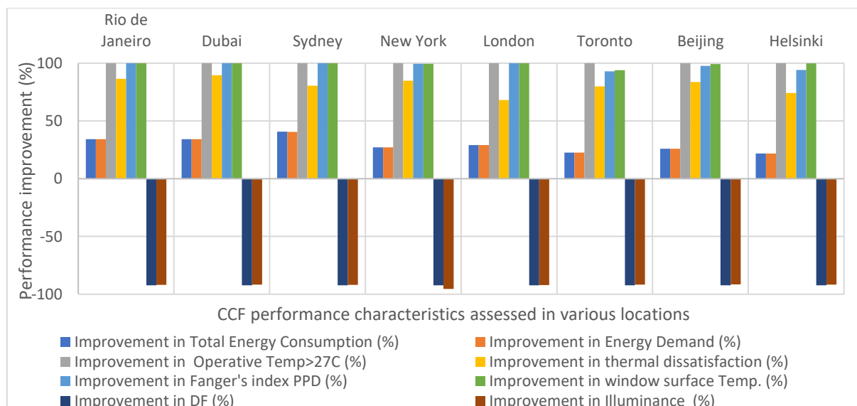
Figure 3. Performance improvements (%) of CCF compared to conventional DGU.
