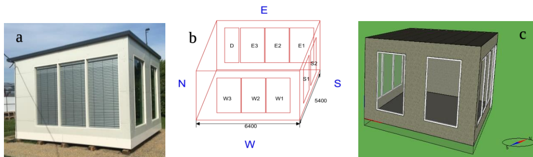
Figure 2. (a) The real MATELab experimental facility, (b) The 3-D CAD drawing and (c) The model in IDA ICE.
