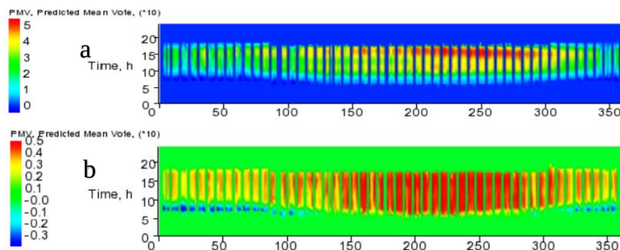
Figure 4. Fanger's index PMV in dry desert hot climate of Dubai (a) for DGU and (b) for CCF.
