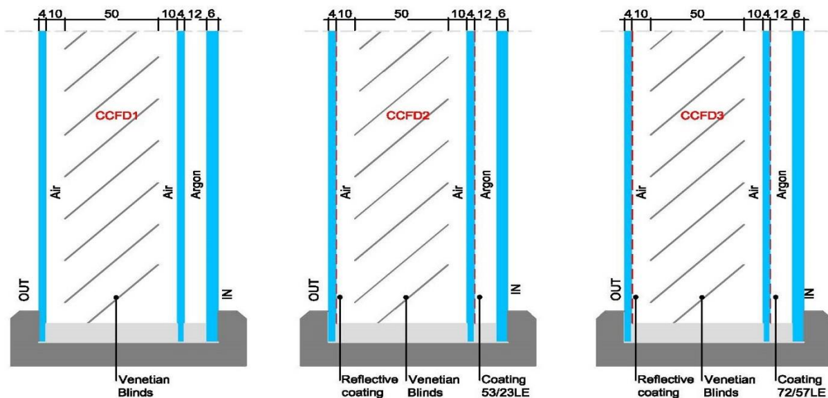
Figure 1. Schematic diagrams of the three groups of CCFs configurations simulated.
