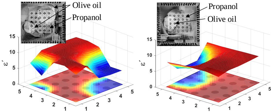
Figure 5.9: 3D permittivity plots and projected images captured by the sensing array chip using drops of olive oil in a base liquid consisting of 2-propanol.
