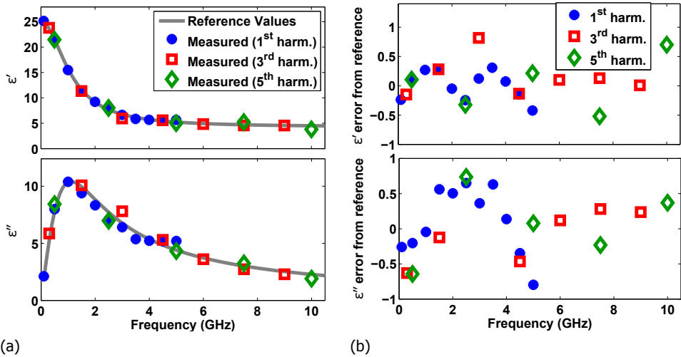
Figure 4.9: (a) Independent measurement of ethanol permittivity versus frequency. The Debye model of ethanol is shown as a reference value. (b) Error between the measured permittivity of ethanol and the values corresponding to its Debye model.
