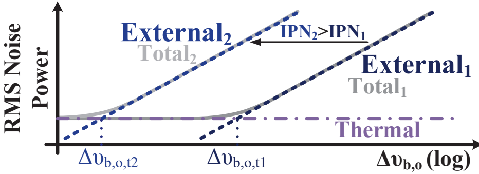
Figure 2.17: Thermal and external noise contributions to the bridge output noise versus bridge differential output voltage, \Delta v_{b,o,t} ) for two different levels of IPN of the external source, showing the reduced noise contribution of a balanced bridge.
