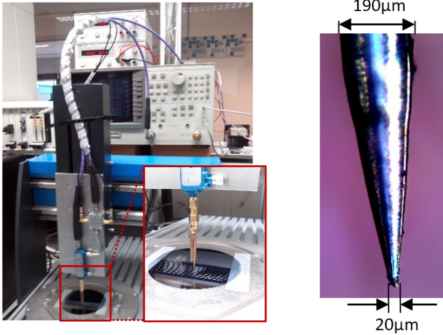
Figure 2.9: Photo of the experimental setup with zoom-in of the probe and the wafer (left) and probe microphotograph and dimensions (right).
