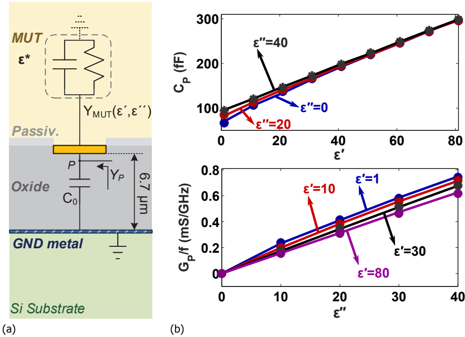
Figure 2.5: (a) Cross-section of utilized patch sensing element and (b) equivalent patch capacitance and conductance from EM simulations (solid lines) and RFM model (dots) for various values of \epsilon' and \epsilon'' at f = 1 GHz.
