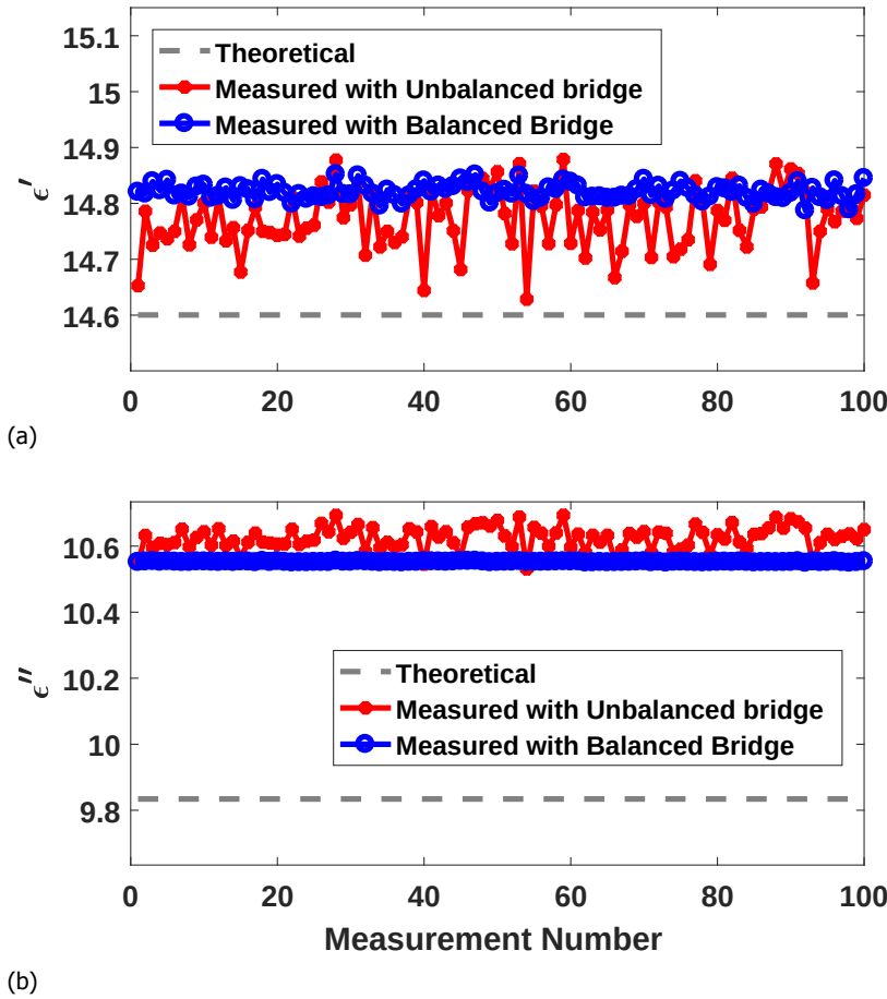
Figure 4.12: Repeated measurements of Ethanol at 1 GHz, showing the reduced readout variation for the balanced bridge case (blue trace) versus an imbalanced case (red trace, for both real and imaginary permittivity values).
