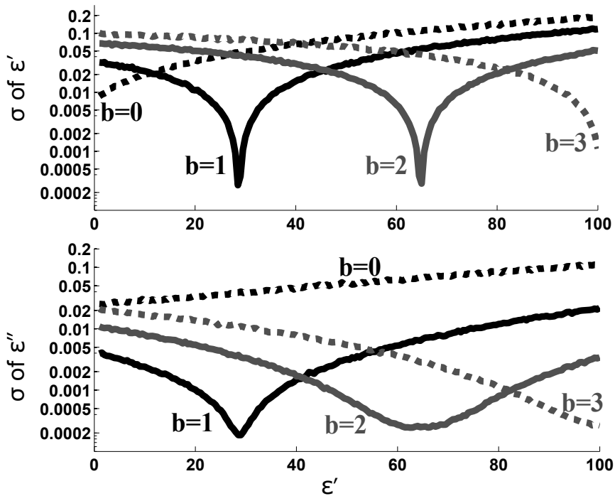
Figure 2.20: Simulated (a) \epsilon' (top) and (b) \epsilon'' (bottom) precision versus real part of permittivity, at different bridge capacitance settings for f = 1 \text{ GHz} , \Delta f = 1 \text{ kHz} , IPN = -90 \text{ dBc} , NF = 7.5 \text{ dB} , CG = 30 \text{ dB} (off-chip amplification included).
