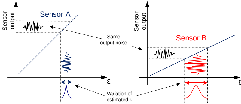
Figure 1.5: Effect of sensor sensitivity on permittivity measurement. In the example of two sensors, A and B, with the same amount of readout noise, sensor B will translate to a higher permittivity variation than sensor A because it has lower sensitivity. Therefore, the precision of sensor B is lower than that of sensor A.
