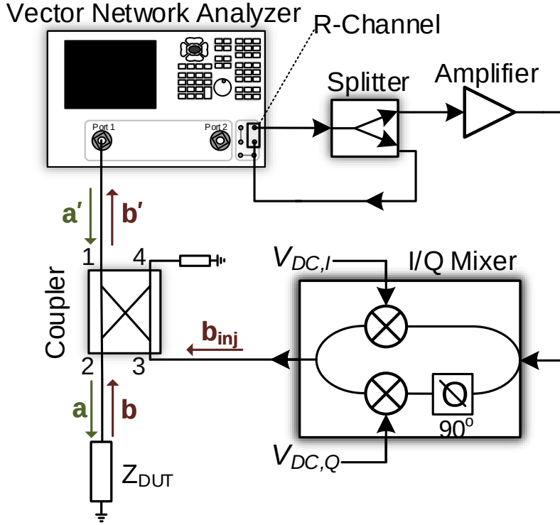
Figure 2.7: Simplified block scheme of the proposed I/Q-steering interferometric technique.
