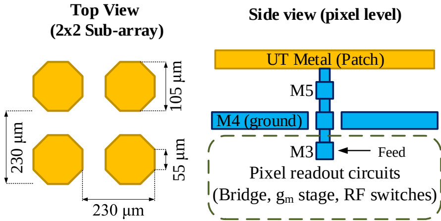
Figure 5.3: Side and top view of the patch within the implemented matrix.
