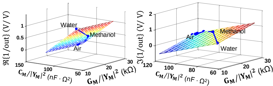
Figure 4.7: Calibration surfaces acquired from the measurements of different liquids, showing a linear dependence of the inverse output real and imaginary part to the normalized admittance and conductance.
