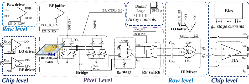
Figure 5.2: Permittivity imager circuit-level architecture.
