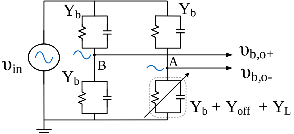
Figure 4.4: RF bridge equivalent schematic for calibration.
