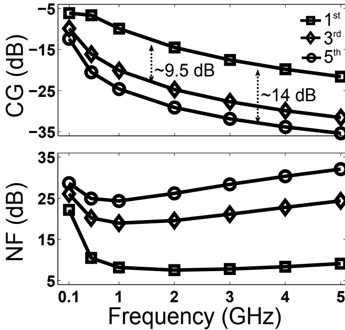
Figure 3.5: Simulated conversion gain (top) and noise figure (bottom) of the downconversion mixer versus fundamental RF frequency f_{RF} , at the first, third, and fifth operation harmonic. An IF frequency of 150 kHz is used.
