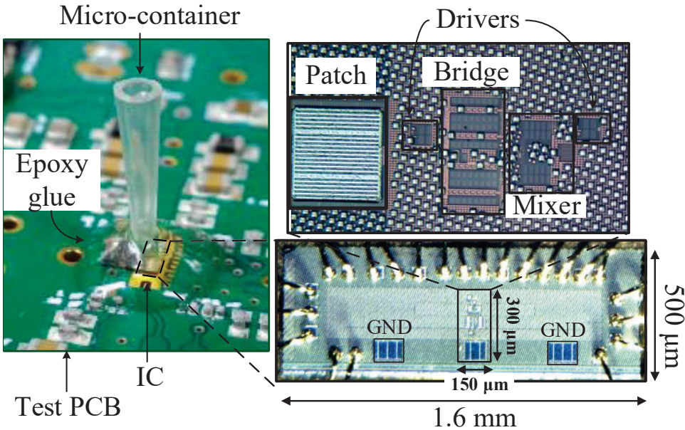
Figure 4.1: Photographs of the fabricated prototype chip and its PCB packaging to measure the complex permittivity of liquid materials.
