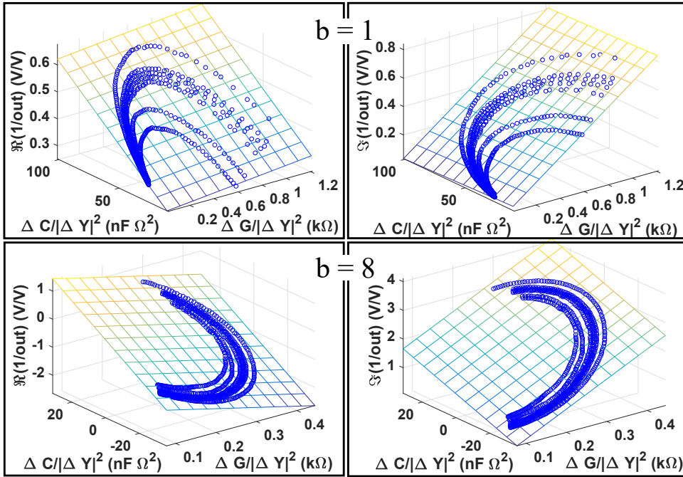
Figure 4.5: Calibration surfaces acquired from all admittance measurements, showing a linear dependence of the real and imaginary part of the inverse output to the normalized admittance and conductance, as suggested by eq. 2.14 and 2.15.
