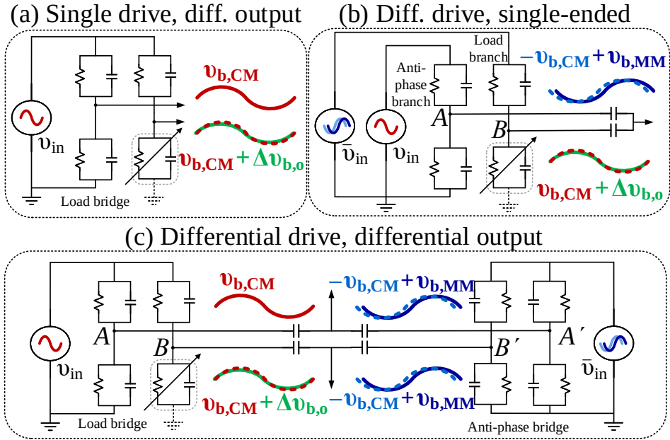
Figure 2.16: Evolution of single-driven, single-ended impedance bridge towards a fully differential, double-balanced topology. v_{b,CM} denotes for common-mode signal, while v_{b,MM} is the signal caused by the phase mismatch between the two out-of-phase driving sinusoids.
