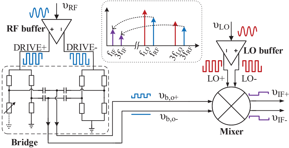
Figure 3.1: Block-level diagram of the multi-harmonic IF downconversion architecture with annotated signals and their frequency-domain representation (insert).
