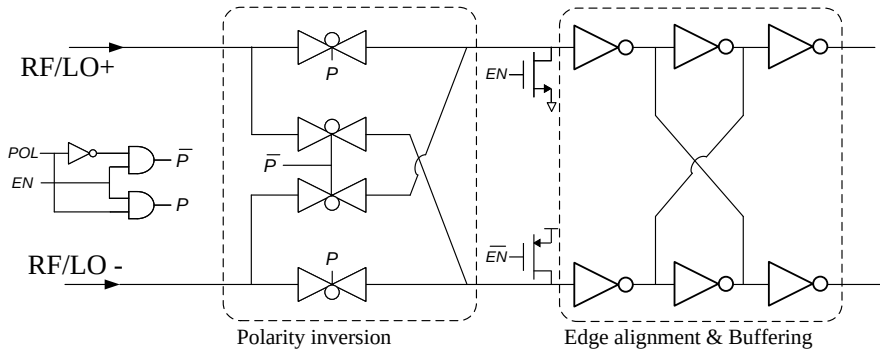
Figure 5.4: RF/LO buffer with enable and polarity option.
