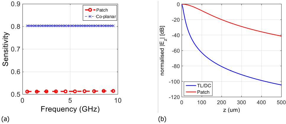
Figure 2.3: Comparison of (a) element sensitivity and (b) magnitude of the normal component of the electric field, normalized to the field intensity at the element-MUT interface between the patch and co-planar capacitive elements.
