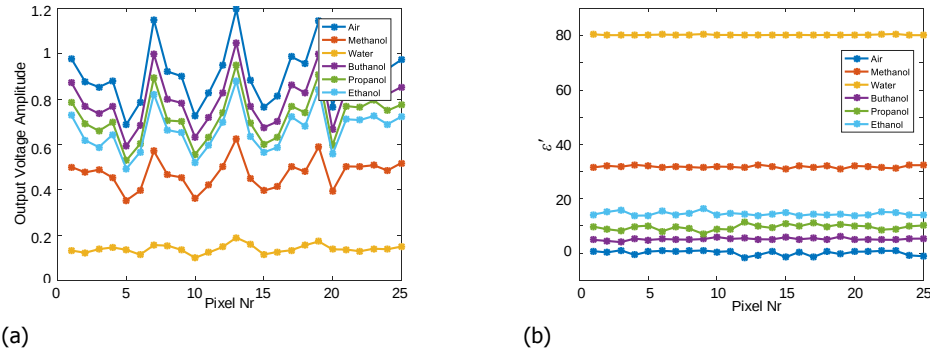
Figure 5.7: (a) Raw output voltage amplitude and (b) calibrated \epsilon' versus array pixel. Ethanol is used as an independent material, with all the others as calibration materials. Pixel numbering starts from top left. Measurements are performed at 900 MHz.
