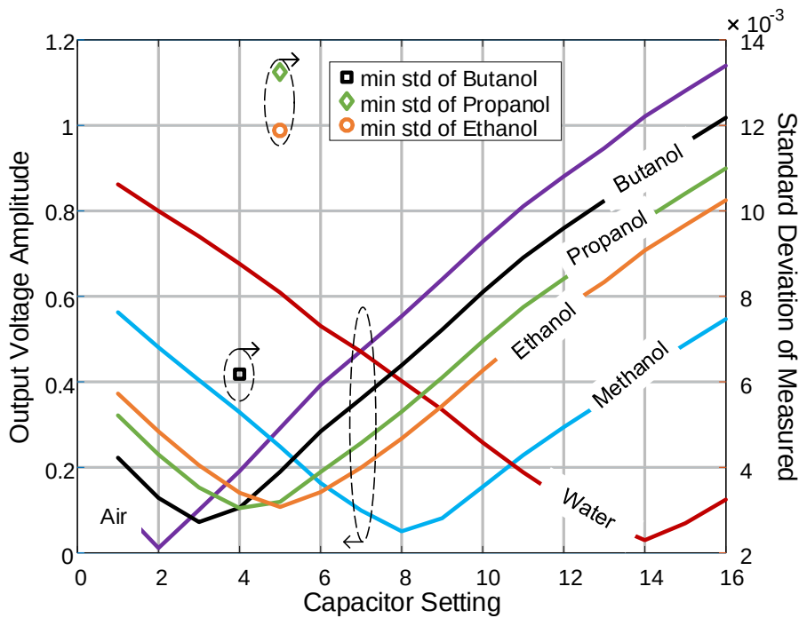
Figure 5.6: Normalized output voltage amplitude of center Pixel (pixel 13) versus capacitor setting for 6 materials at 900 MHz, and the corresponding lowest standard deviation ( \sigma ) of chosen independent material.
