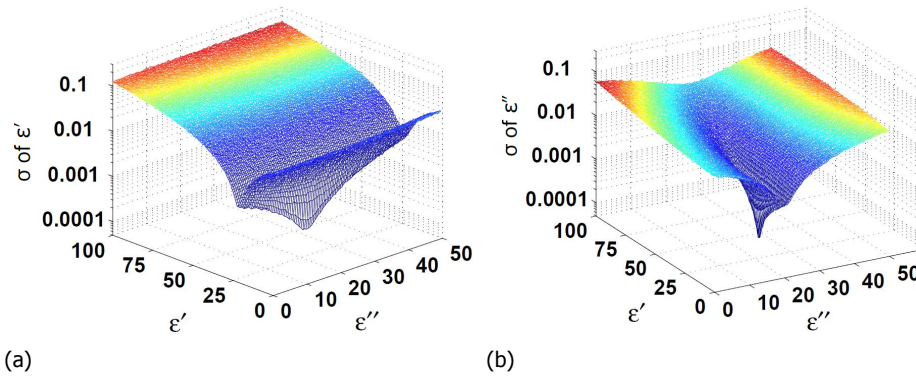
Figure 2.19: Simulated \epsilon' and \epsilon'' precision versus permittivity for the chip model for f = 1 \text{ GHz} , b = 2 , \Delta f = 1 \text{ kHz} , \text{IPN} = -90 \text{ dBc} , \text{NF} = 7.5 \text{ dB} , \text{CG} = 30 \text{ dB} (off-chip amplification included).
