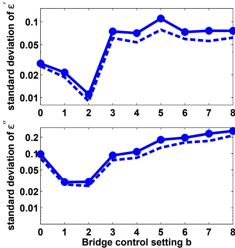
Figure 4.11: Permittivity precision versus bridge control setting b , for ethanol measurement at 1 GHz (solid line). The dashed line corresponds to the expected precision if the phase and amplitude variance were equal to the Cramér-Rao bound.
