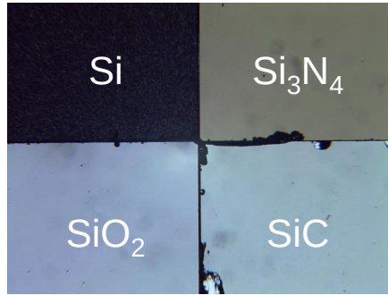
Figure 2.13: Multi-die structure comprising Si, Si 3 N 4 , SiO 2 , and SiC dies placed aside for permittivity measurement with the proposed SMM setup .
