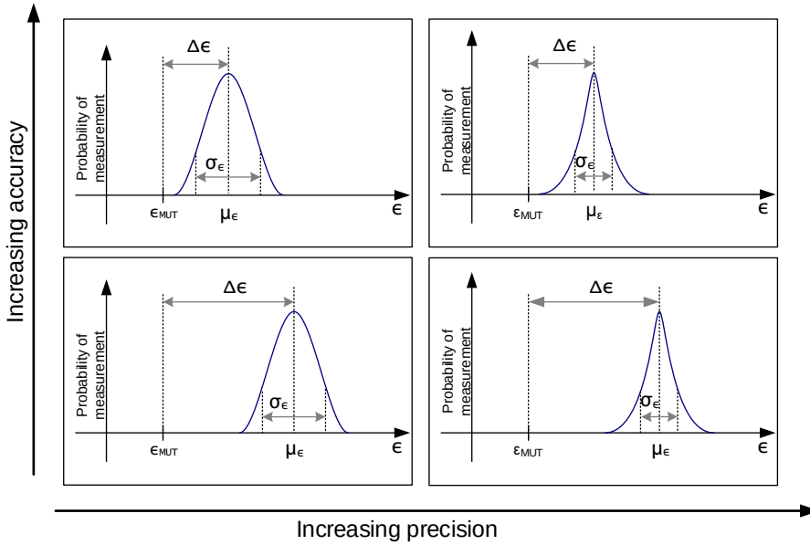
Figure 1.4: Examples demonstrating the difference between accuracy and precision: in a high accuracy system, the mean measured value is close to the actual MUT value, while a high precision system features a low variance of repeated measurements.
