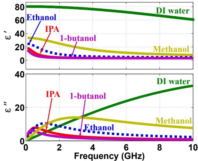
Figure 1.2: The real and imaginary part of permittivity of the materials measured, versus frequency, generated from their Debye models [15]. Ethanol (dashed line) is often used for sensor system validation as independent reference material.
