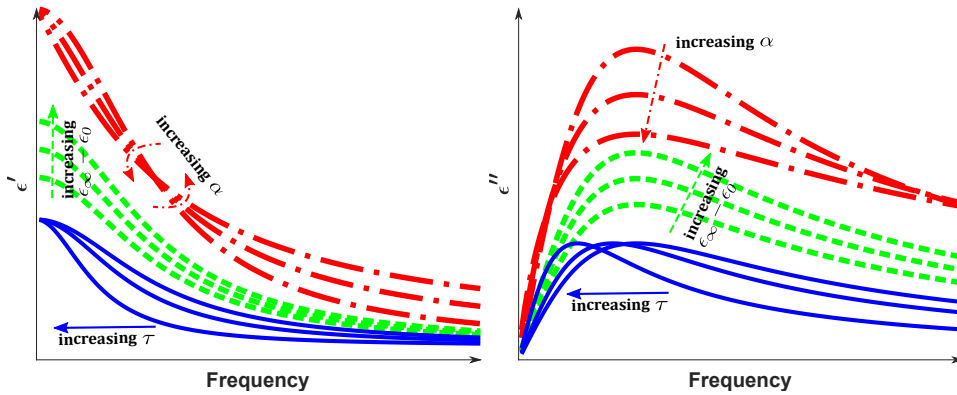
Figure 1.1: Illustrative plots of typical \epsilon' and \epsilon'' variation versus frequency, according to the Cole-Cole equation (1.1). It shows how individual Cole-Cole model parameters affect \epsilon' and \epsilon'' when all other parameters of the model are kept constant.
