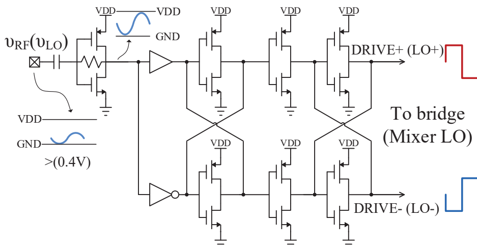
Figure 3.6: Schematic of the bridge and mixer drivers.
