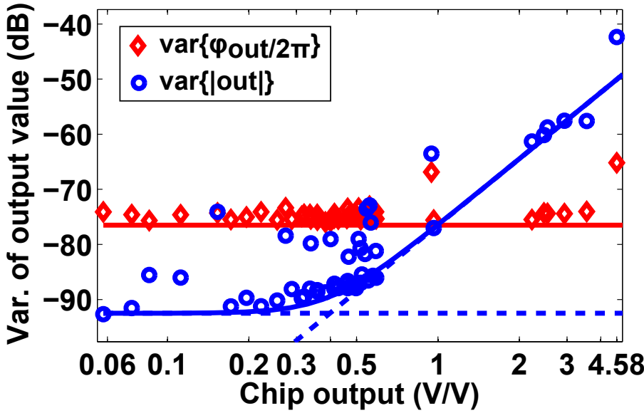
Figure 4.10: Output phase and amplitude variance versus chip ratiometric output value for all measured materials and all bridge capacitance settings (varying bridge imbalance) at 1GHz, with annotated expected Cramér-Rao measurement bounds of (2.26) and (2.27). \Delta f = 1 \text{ kHz} , IPN = -90 \text{ dBc} , NF = 7.5 \text{ dB} , CG = 30 \text{ dB} (off-chip amplification included).
