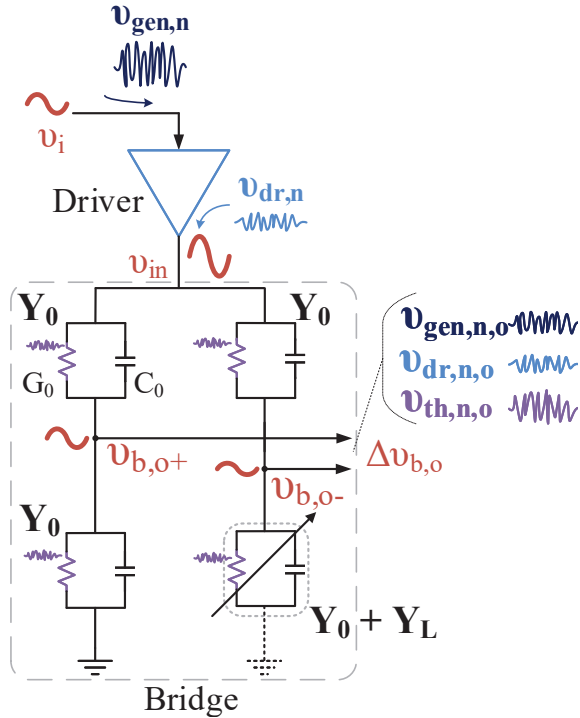
Figure 2.15: Balanced impedance bridge, driven at RF frequency by a driver, with annotated signals and noise sources contributing to the total noise at the output of the bridge.
