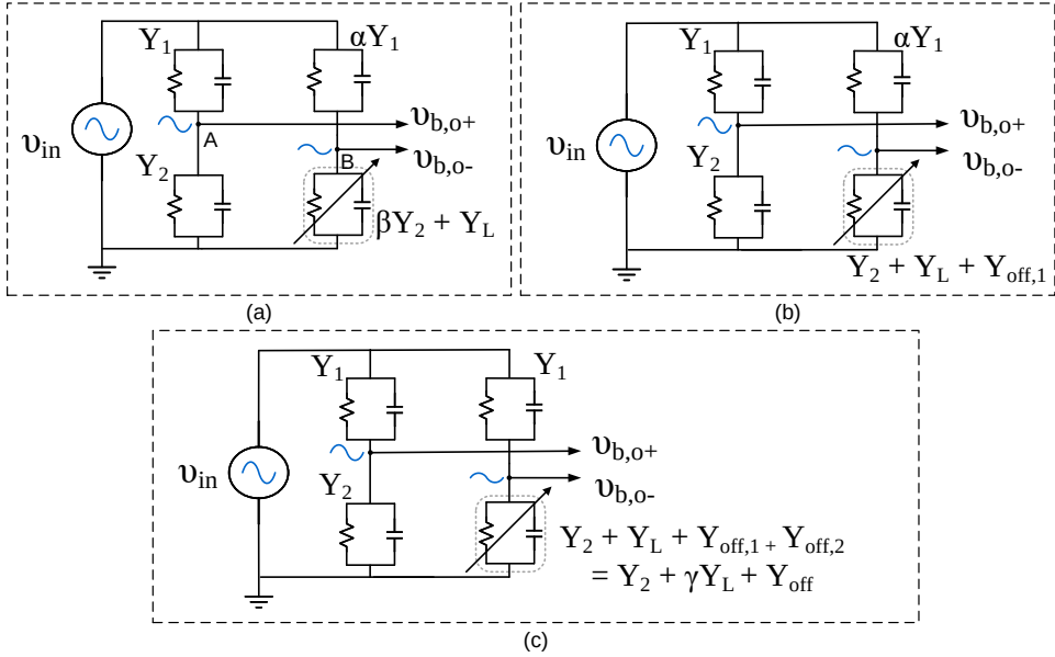
Figure A.1: Bridge analysis in the presence of mismatch between the branches.
