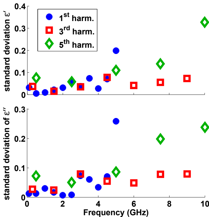
Figure 4.8: Measured permittivity precision of ethanol using first, third, and fifth frequency harmonics.
