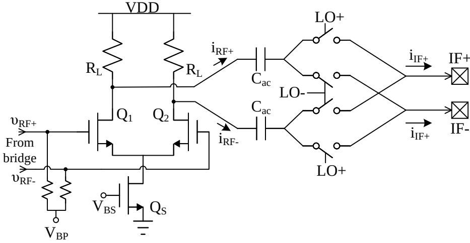
Figure 3.4: Current-mode downconversion mixer schematic consisting of a transconductance stage and a current-mode switch quad.
