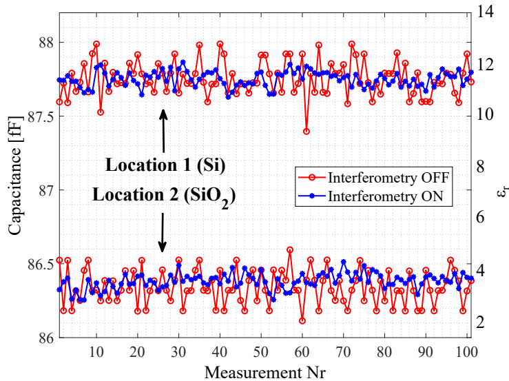
Figure 2.12: Measurement traces (100 points) of two locations of the wafer with different materials ( \text{SiO}_2 and Si respectively), with and without the interferometric technique (blue asterisk and red circle trace, respectively).
