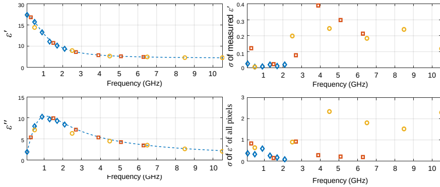
Figure 5.8: Measured ethanol real ( \epsilon' ) and imaginary ( \epsilon'' ) versus frequency, as a result of averaging of all 25 pixels and associated measured standard deviations among individual array pixels. Blue diamond: first harmonic, orange square: third harmonic, yellow circle: fifth harmonic.
