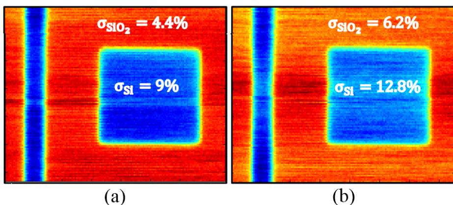
Figure 2.11: Two-dimensional images of a 3 \times 2.4 \text{ mm}^2 extract of the wafer (scanning step of 20 \mu\text{m} ). (a) Image acquired from measured \Gamma amplitude with interferometric technique and (b) image acquired from measured \Gamma phase without the interferometric technique. The standard deviation of measurement of all measurement points that fall within the same material is annotated ( \text{SiO}_2 – red and Si – blue).
