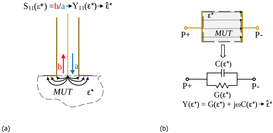
Figure 2.1: Commonly used broadband permittivity sensing elements : (a) Coaxial probe and (b) parallel-plate capacitance.
