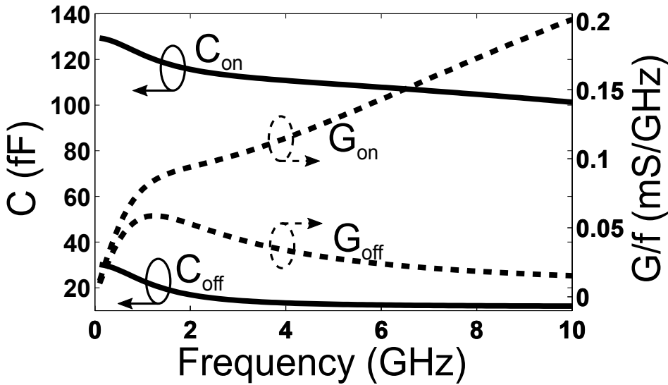
Figure 3.3: Equivalent parallel capacitance and normalized conductance of switched-capacitor at on and off stage.
