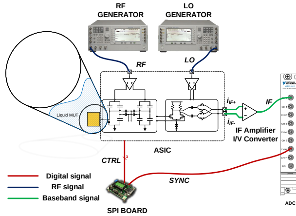
Figure 4.2: Block diagram of chip measurement setups; (a) setup used to verify the bridge operation with an RF tuner as load and (b) setup for the measurement of liquid MUTs. The RF, LO, and read-out circuitry control is the same in both the tuner and the liquid material measurement.
