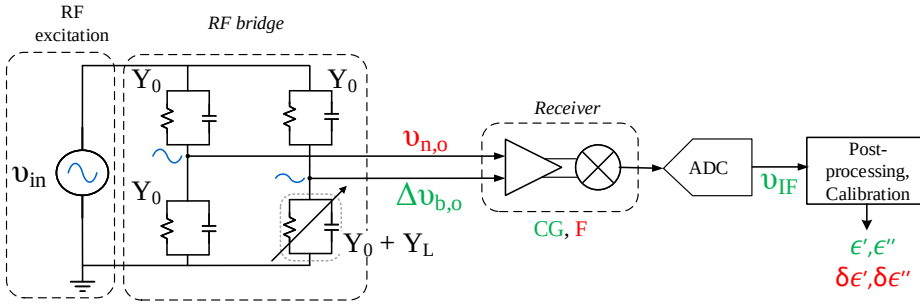
Figure 2.18: Generic receiver-based readout system, including the RF bridge.
