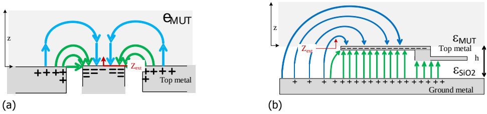
Figure 2.2: Cross-sections and pictorial representation of field lines and charge distribution for two CMOS-compatible sensing element implementations : (a) Differential sensing element and (b) single-ended patch.
