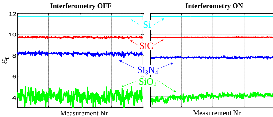
Figure 2.14: Permittivity measurement of the four materials in the multi-die structure of fig. 2.13, when the proposed active interferometric technique is OFF (left) or ON (right)).
