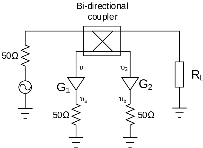
Figure 2.6: Principle schematic for the measurement of a reflection coefficient.
