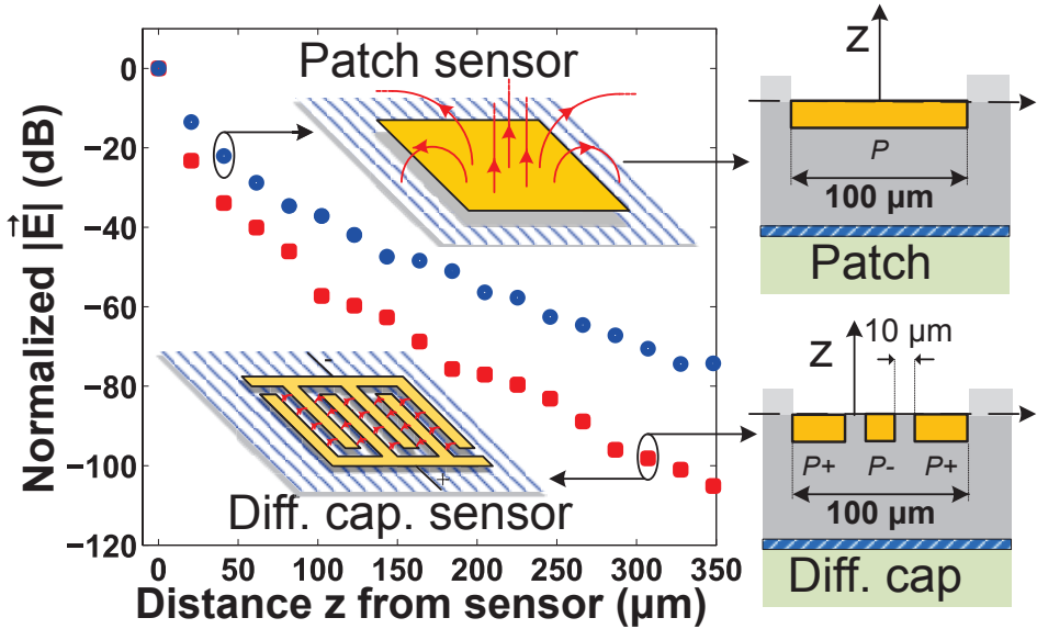
Figure 2.4: EM simulation of normalized electric field magnitude versus vertical distance from the sensor interface for two types of sensors both occupying the same 100 \times 100 \mu\text{m}^2 area: a single-ended patch and a differential capacitor with 10 \mu\text{m} between fingers.
