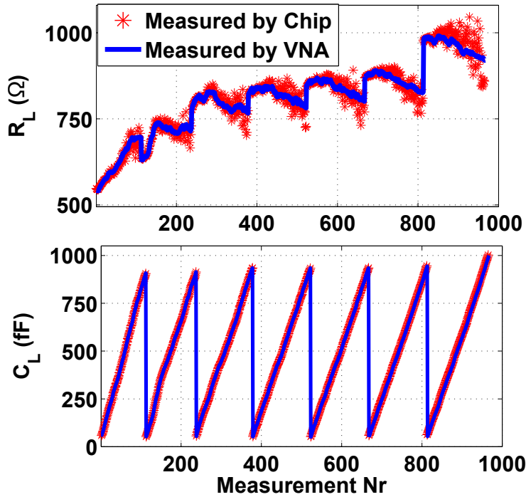
Figure 4.6: Measured load shunt capacitance and resistance for 960 different tuner settings at b = 1 .
