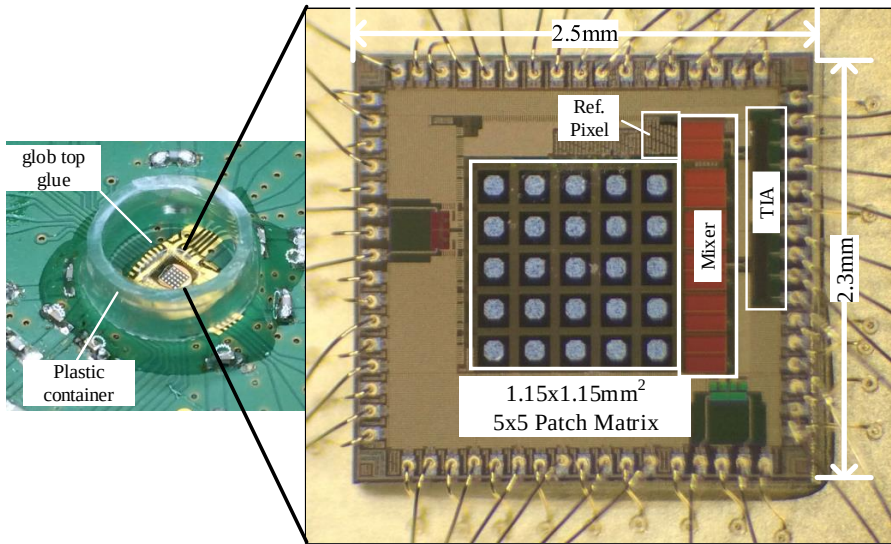
Figure 5.5: Photograph of prototype chip assembly and chip micrograph.
