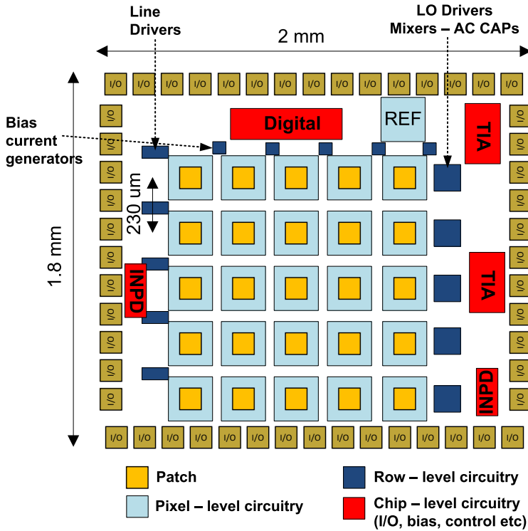
Figure 5.1: Floorplan of the implemented 5 \times 5 permittivity imaging array, depicting the physical placement of individual building blocks and the hierarchical levels.
