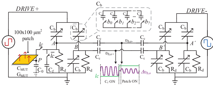
Figure 3.2: Schematic of the fully differential, double-balanced bridge with its sensing patch, implemented on the top metals of the 40-nm CMOS technology.
