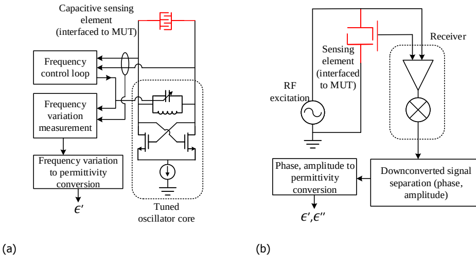
Figure 1.3: Categorization of CMOS integrated BDS system architectures : (a) PLL-based architecture and (b) receiver-based architecture.
