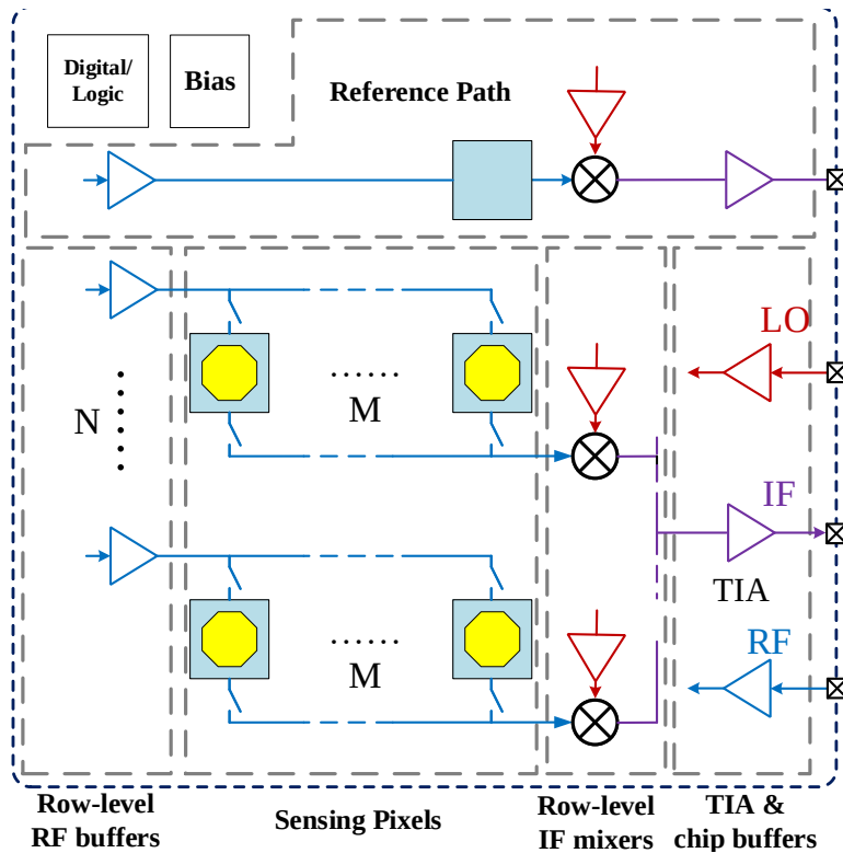
Figure 3.7: Conceptual top-level block diagram of a N \times M permittivity sensing array.
