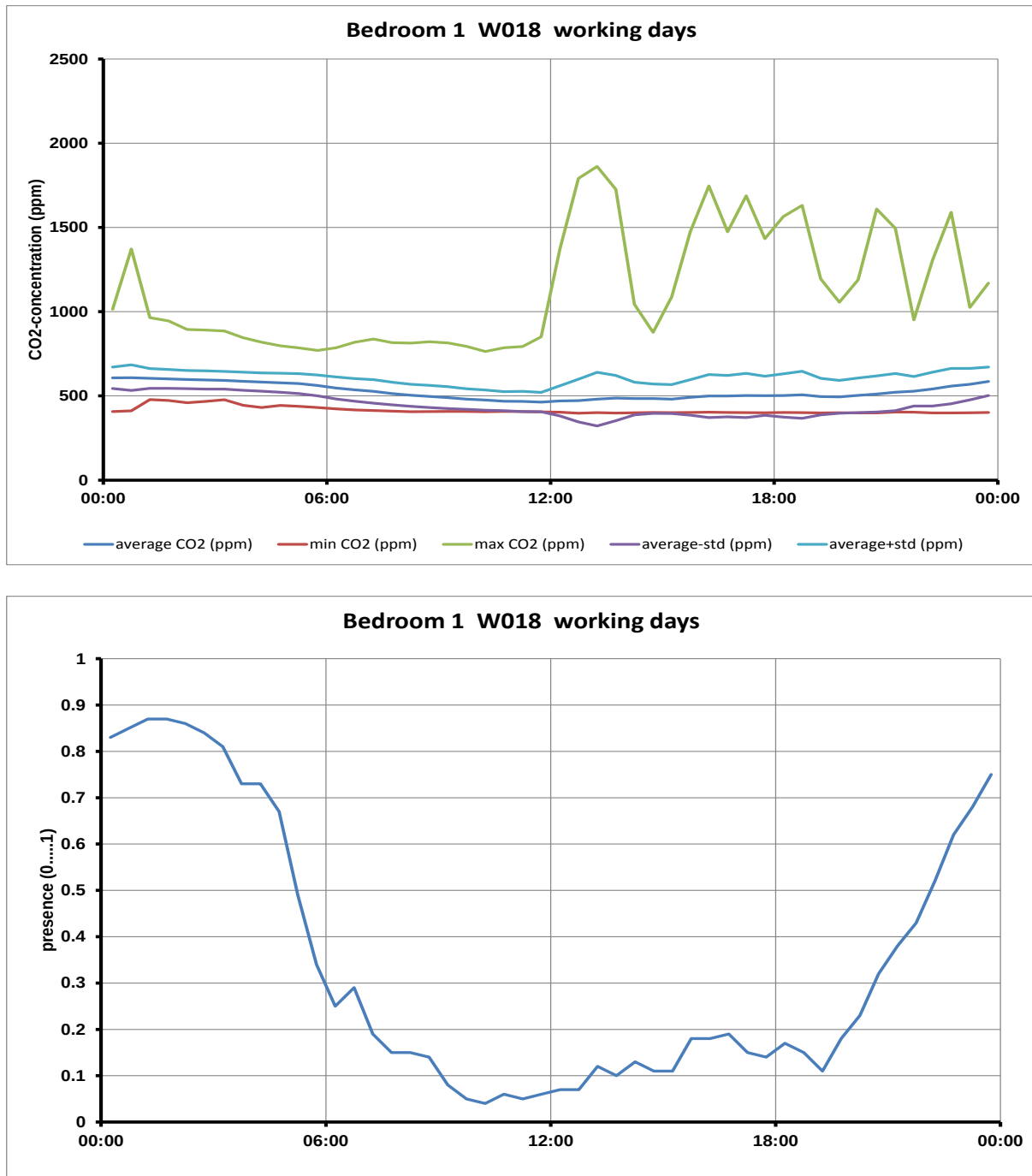
Figure 6.17: CO 2 -profile and presence profile for bedroom 1 in dwelling W018 for working days based upon the complete 6 months measuring period
