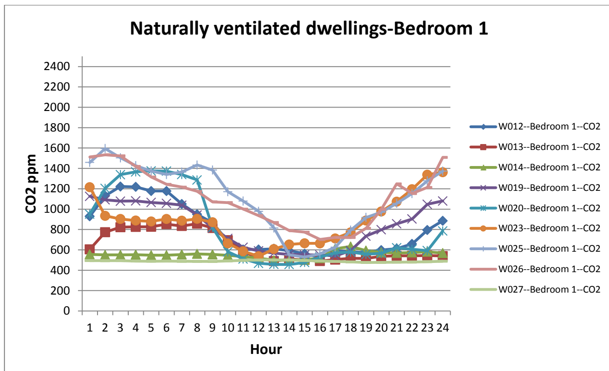
Figure B.10: 24-hour CO 2 profiles of bedroom 1 for the naturally ventilated dwellings.
