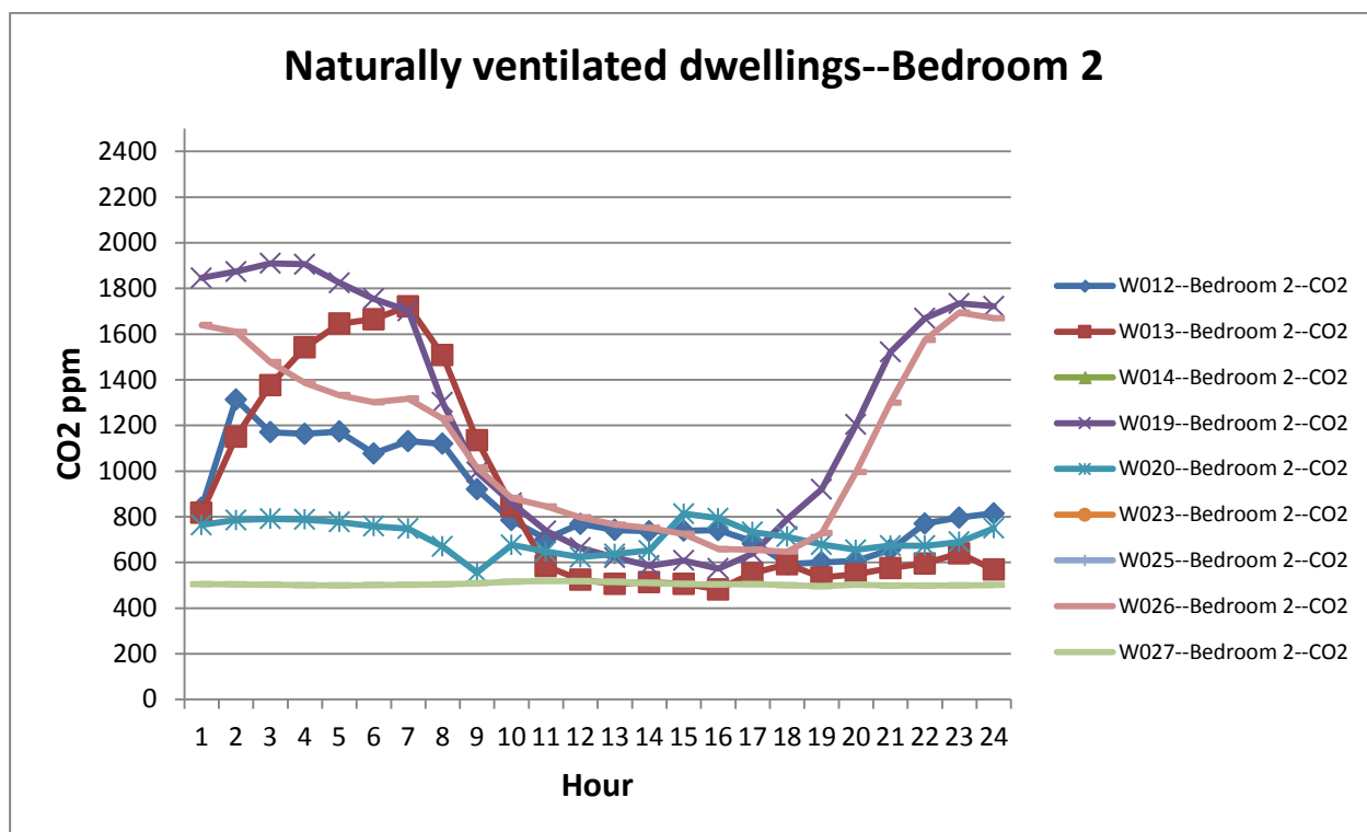
Figure B.11: 24-hour CO 2 profiles of bedroom 2 for the naturally ventilated dwellings.
