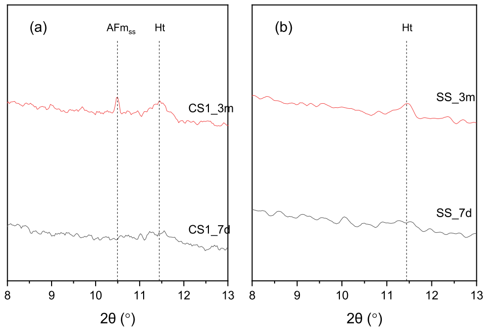
Fig. 14. XRD patterns from 8 to 13° ( 2\theta ) of (a) C_3S -slag CS1 and (b) C_3S -slag SS blends highlight the presence of Ht and AFm-phase. Ht: hydrotalcite; AFm ss : solid solution of hemihydrate and OH^- substituted monosulfate.
