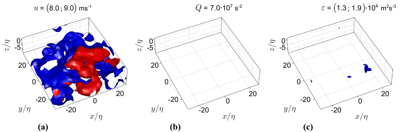
Fig. 15 Instantaneous snapshot from a so-called ‘sleeping’ state of the flow showing iso-surfaces of a streamwise velocity, b Q , and c turbulent dissipation rate \varepsilon
