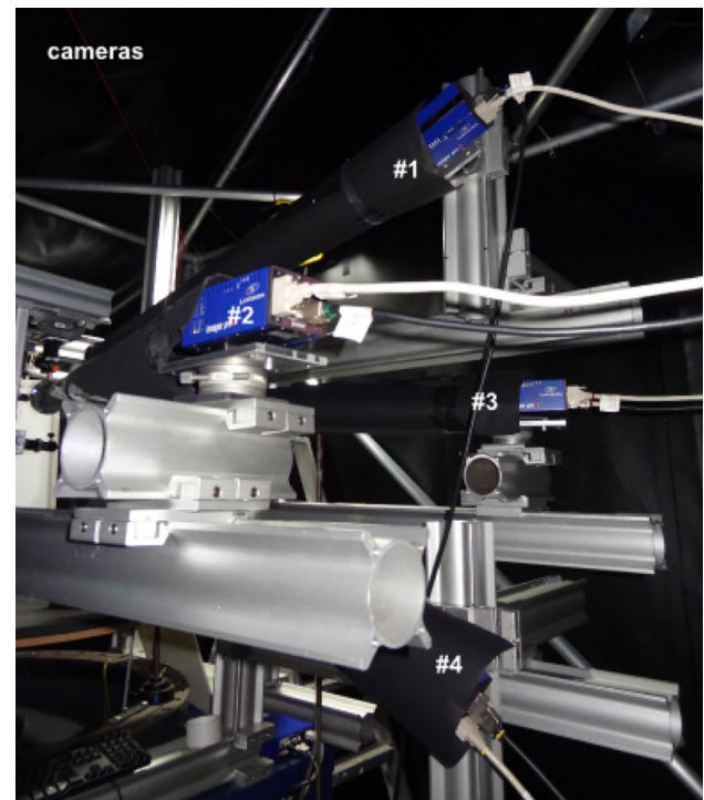
Fig. 3 Photograph of the experimental setup showing the positioning of the four cameras in the 3D space. For each camera, the optical path between the CCD sensor and the associated lens was shielded to reduce the capturing of day light
