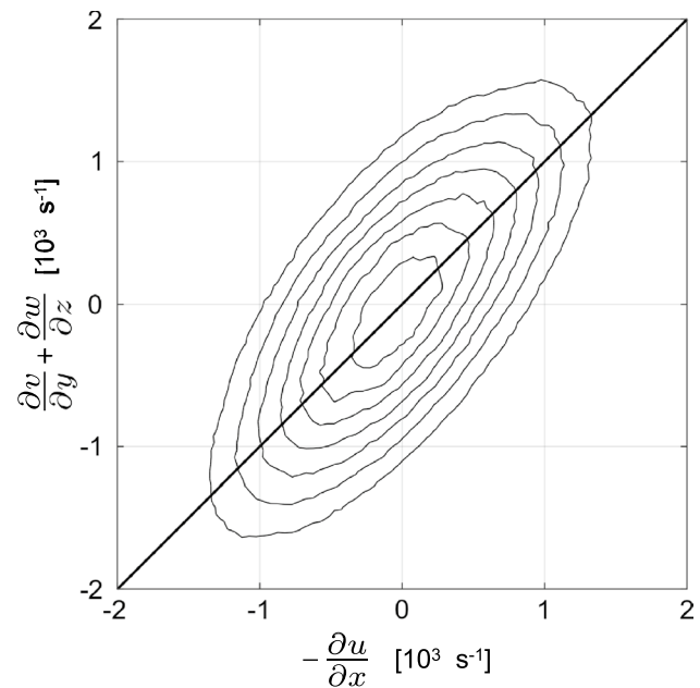
Fig. 9 Joint probability density function of -\partial u/\partial x and (\partial v/\partial y + \partial w/\partial z) with VIC+ and the regression filter. Contours in range from 7 \cdot 10^{-8} to 2.5 \cdot 10^{-7} in increments of 3 \cdot 10^{-8}
