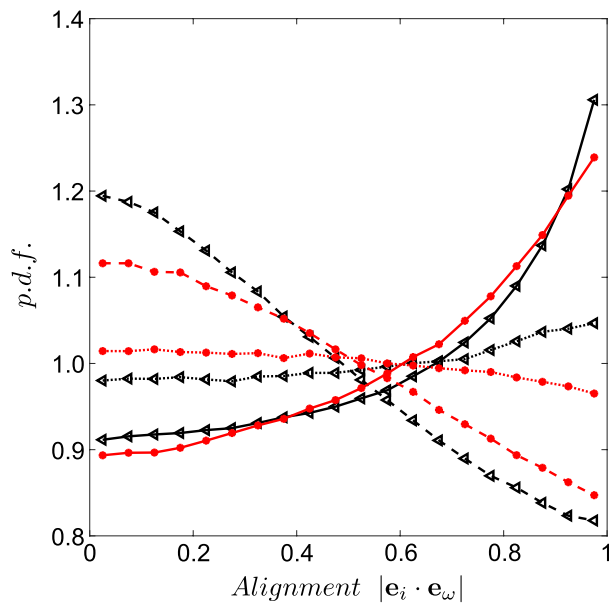
Fig. 12 Probability density functions of the cosine alignments between the eigenvectors of the strain-rate tensor and the vorticity vector. Red lines with circles are results from the present experiment; black lines with triangles are results from DNS simulations of homogeneous isotropic turbulence (HIT) at Re_\lambda \approx 433 (Li et al. 2008). Extensive, intermediate, and compressive eigenvectors are identified, respectively, by dotted lines, dashed lines, and continuous lines
