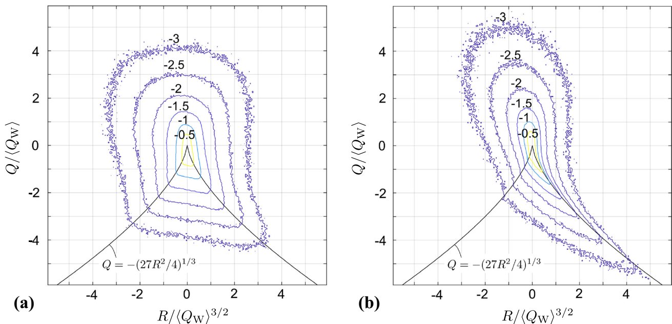
Fig. 11 Joint probability density functions of the second (Q) and third (R) invariants of the velocity gradient tensor obtained from velocity vector fields from a the present experiment, and b DNS simulations of homogeneous isotropic turbulence (HIT) at Re_\lambda \approx 433
