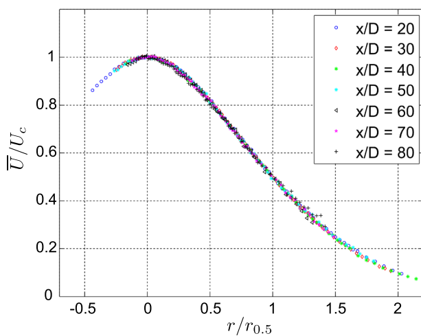
Fig. 1 Mean streamwise velocity against radial position at different nozzle diameters D downstream from the jet nozzle, from measurements with hot-wire anemometry
