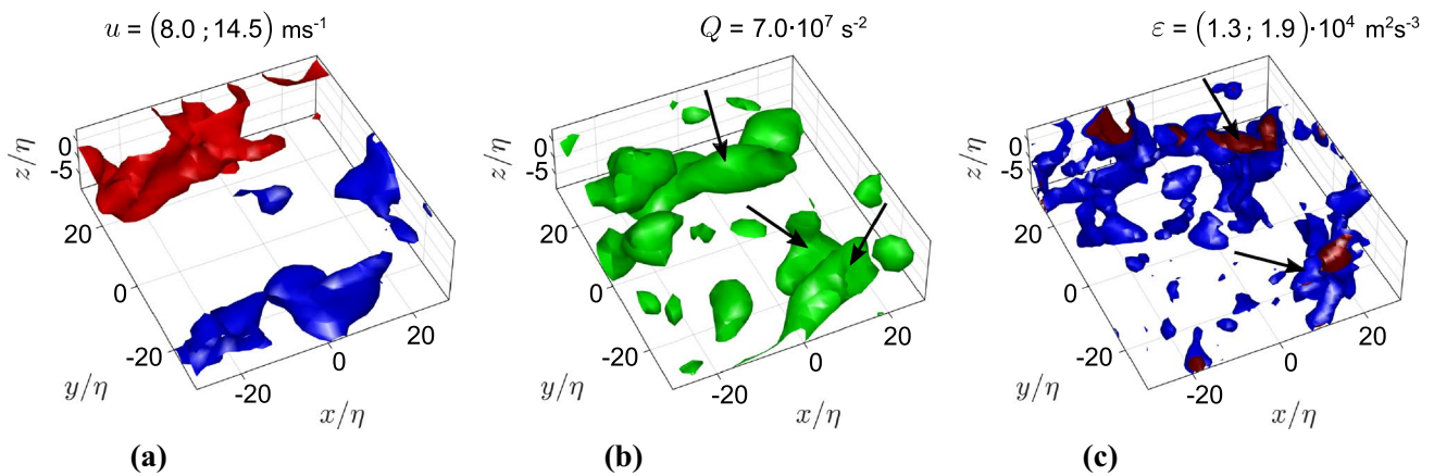
Fig. 14 Instantaneous snapshot from a so-called ‘hyperactive’ state of the flow showing iso-surfaces of a streamwise velocity, b Q , and c turbulent dissipation rate \varepsilon
