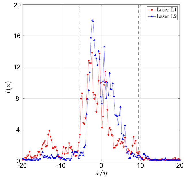
Fig. 7 Light intensity distribution in a tomographic reconstruction averaged along the x and y directions. L1 corresponds to the first image (first laser pulse) and L2 to the second one (second laser pulse). The thickness of the light sheet can be estimated to be approximately 16\eta , equivalent to 912\text{ }\mu\text{m} . The dashed lines identify the extent along the z -axis of the reconstructed volume for cross-correlation
