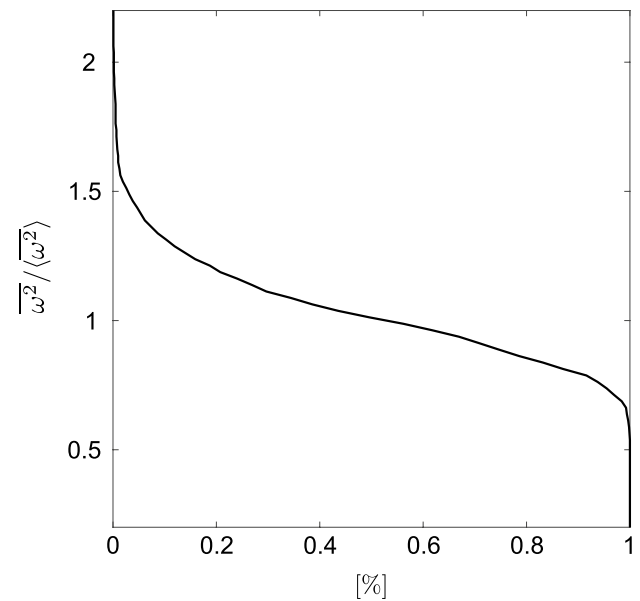
Fig. 13 Cumulative distribution function of the average non-dimensional enstrophy in each snapshot
