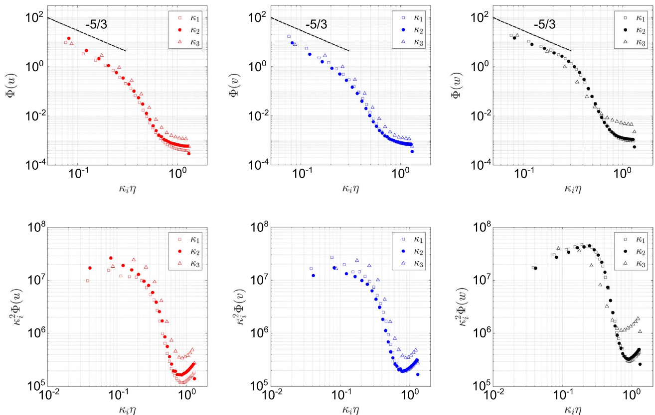
Fig. 8 Spectra of the streamwise (left), transversal (middle), and out-of-plane components of the velocity (right column) along the three Cartesian axes; top , velocity spectra and, bottom , dissipation spectra
