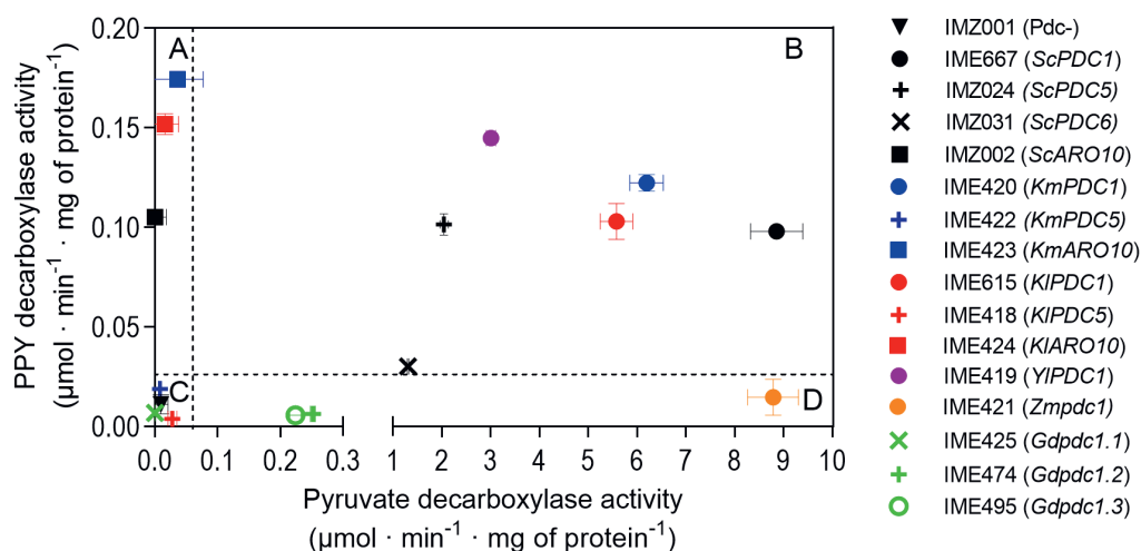
Figure 4. Specific decarboxylase activities for pyruvate and phenylpyruvate (PPY) in cell extracts of CENPK711-7C ( pdclΔ pdc5Δ pdc6Δ aro10Δ thi3Δ URA3 ↑ ) expressing individual 2-oxo acid decarboxylase genes from a multicopy plasmid. All strains were grown duplicates at 30 °C on synthetic medium containing 2% (v/v) glycerol and 2% (v/v) ethanol as carbon source (SMEG). Black: S. cerevisiae , blue: K. marxianus , purple; Y. lipolytica , red: K. lactis , orange; Z. mobilis , green: G. diazotrophicus . Strains tested were IMZ001 ( pdclΔ pdc5Δ pdc6Δ aro10Δ thi3Δ URA3 ↑ ), IMZ002 ( ScARO10 ↑ ), IMZ024 ( ScPDC5 ↑ ), IMZ031 ( ScPDC6 ↑ ), IME418 ( KlPDC5 ↑ ), IME419 ( YlPDC1 ↑ ), IME420 ( KmPDC1 ↑ ), IME421 ( Zmpdc1 ↑ ), IME422 ( KmPDC5 ↑ ), IME423 ( KmARO10 ↑ ), IME424 ( KlARO10 ↑ ), IME425 ( GdPdc1.1 ↑ ), IME474 ( GdPdc1.2 ↑ ), IME495 ( GdPdc1.3 ↑ ), IME615 ( KlPDC1 ↑ ) and IME667 ( ScPDC1 ↑ ). The dotted line indicates the detection limit for decarboxylase activity, which was <0.04 \mu\text{mol} \cdot \text{mg protein}^{-1} \cdot \text{min}^{-1} for pyruvate as substrate and <20 \text{ nmol} \cdot \text{mg of protein}^{-1} \cdot \text{min}^{-1} for phenylpyruvate as substrate. This results in the visualization of 4 classes: enzymes with decarboxylase activity for A) PPY but not pyruvate, B) both PPY and pyruvate C) no activity for either substrate and D) activity for pyruvate, but not PPY.
