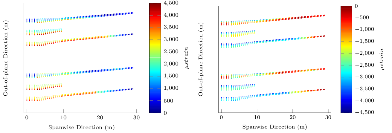
(a) \epsilon_{\max} of the spars of the quasi-isotropic wing (top three) and the tailored wing (bottom three) for load case 5, LE to TE from top to bottom. (b) \epsilon_{\min} of the spars of the quasi-isotropic wing (top three) and the tailored wing (bottom three) for load case 5, LE to TE from top to bottom.
