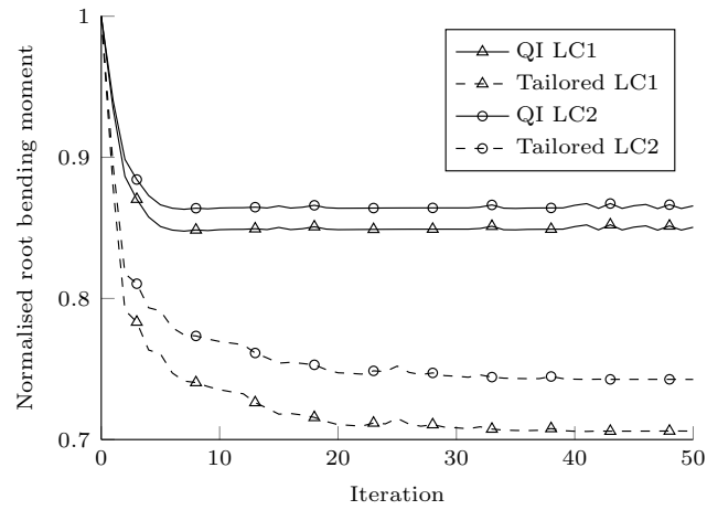
(b) Evolution of the root bending moment of load case 1 and load case 2 normalised with respect to the initial design
