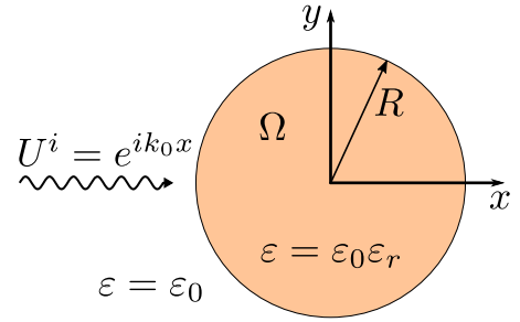
FIG. 4. Geometry of the 2D problem. The incident plane wave U_i represents either the z component of the electric field, E_z , or the z component of the magnetic field H_z . In this work, we will only consider the TM polarization case (namely the E_z case).
