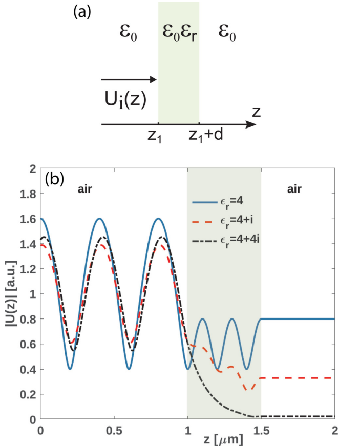
FIG. 1. (a) Geometry of the 1D electromagnetic problem studied. The scatterer has relative permittivity \epsilon_r and thickness d . (b) Absolute value of the analytical solution of the total field U(z) . Each curve corresponds to a different medium: \epsilon_r = 4 , blue-solid line, \epsilon_r = 4 + i , red-dashed line, \epsilon_r = 4 + 4i black-dot dashed line. Also, z_1 = 1 \mu\text{m} and d = 500 \text{ nm} .
