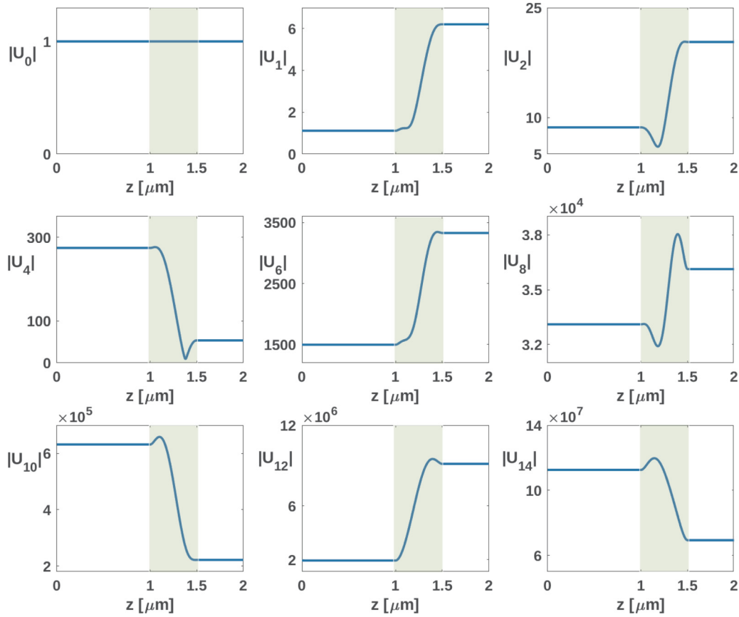
FIG. 2. Some perturbation orders of Eq. (6), for the case where \varepsilon_r = 4 + i , d = 500 nm and \lambda = 800 nm. The series clearly diverges for any value of z .
